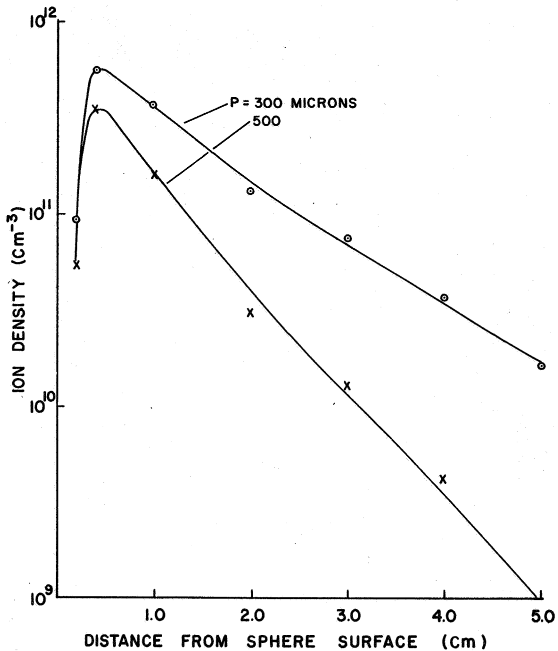
ION DENSITY PROFILES: 50mA
