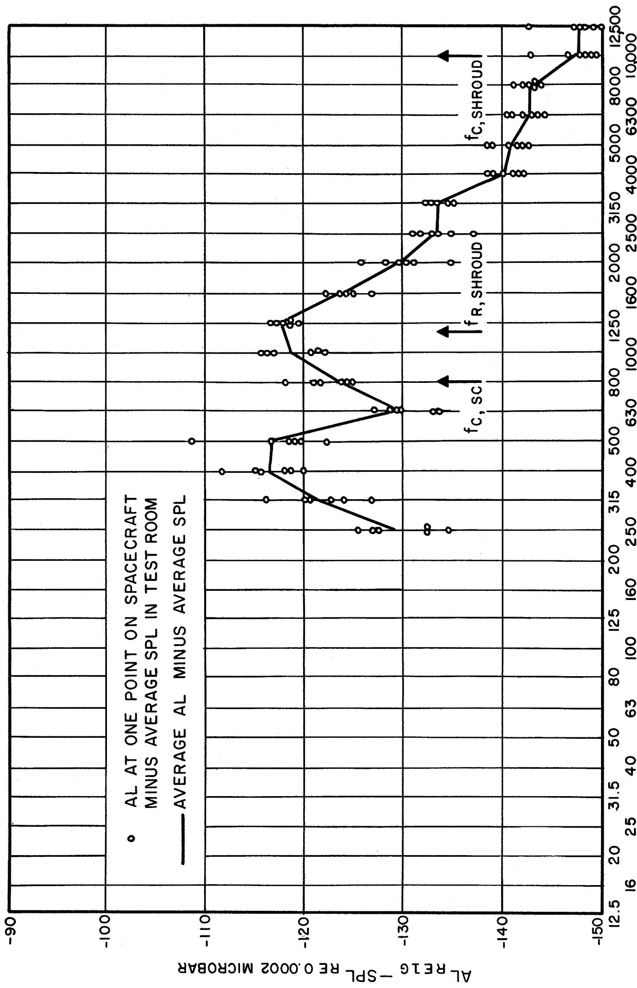
FIG.25 RESPONSE OF MODEL SPACECRAFT WHEN ENCLOSED IN MODEL-SHROUD - MOUNTING TRUSSES NOT CONNECTED
