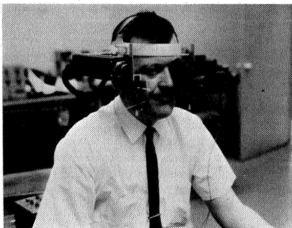
FIGURE 1.—Eye motion analysis. The individual is being tested to determine how his eye movement reacts to a display. On the left is a small television vidicon camera that shows the area at which the subject is looking. On the right is a device that shines a light on the subject's eyeball and picks up the reflection that is superimposed on the field of view seen by the TV camera.
