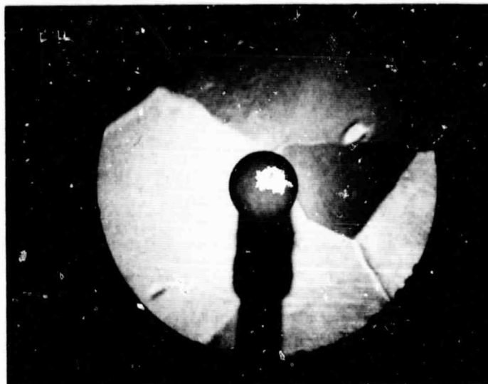
a. Initially Polished (662X)
