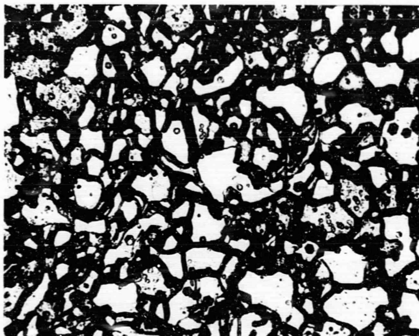
Figure 7. 100X Photomicrograph of Polished and Electro- Etched Vapor-Deposited Rhenium (see Fig. 6)
