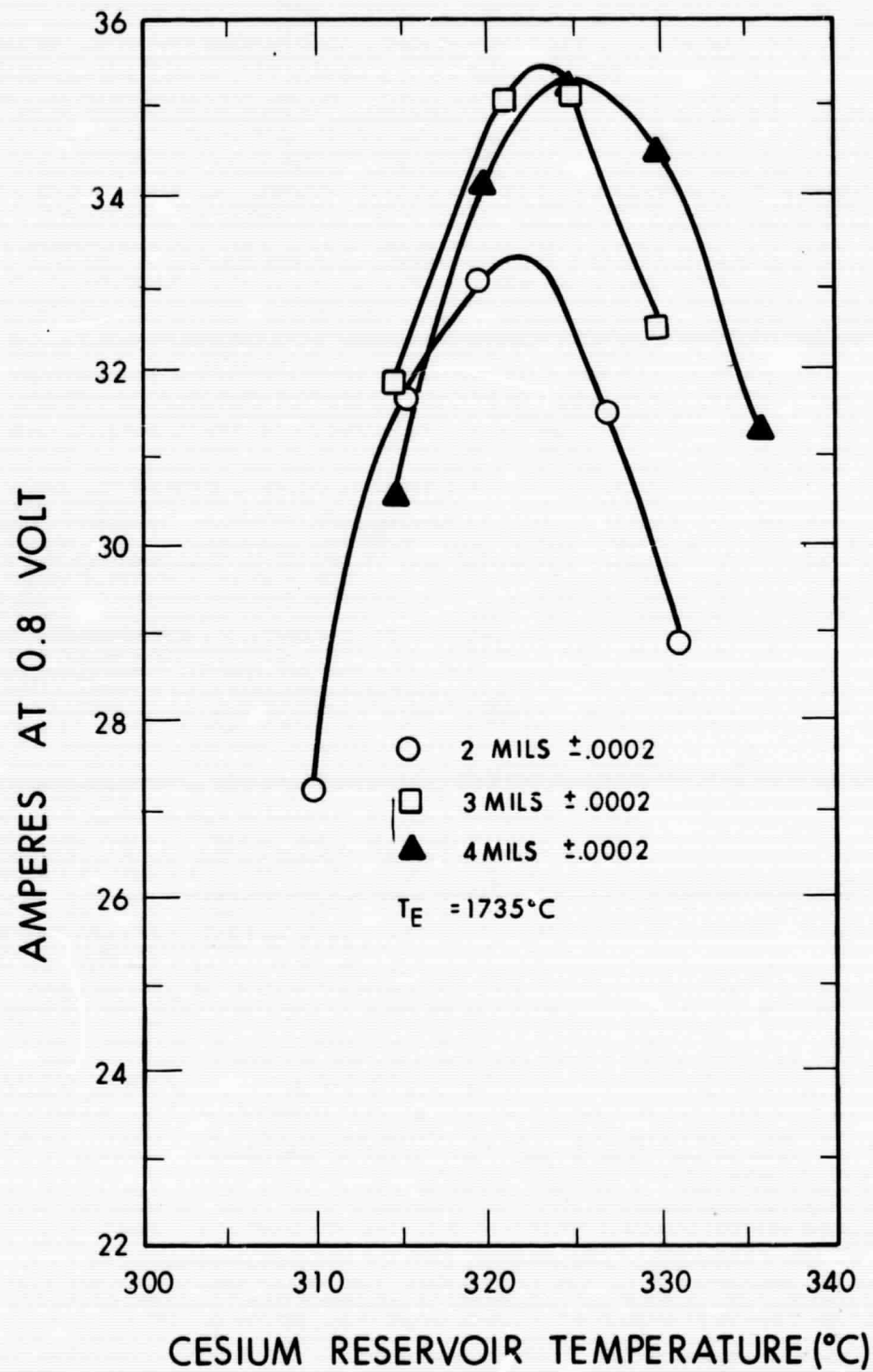
Figure 51. Converter Optimization at 0.80 Volt. Temperature of Collector 704 to 710 ^\circ\text{C} (all dc data points)
