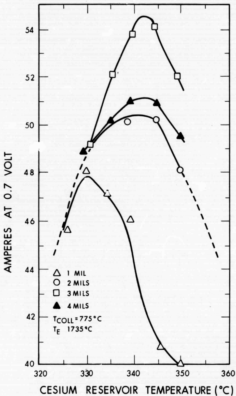
Figure 49. Converter Optimization at 0.7 Volt. Temperature of Collector 775^{\circ}\text{C} (all dc data points)
