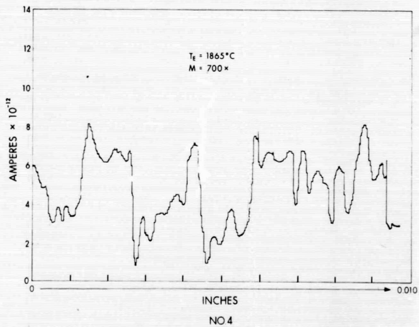
Figure 32. Mapped Composite of Sample Area with Current Profiles
