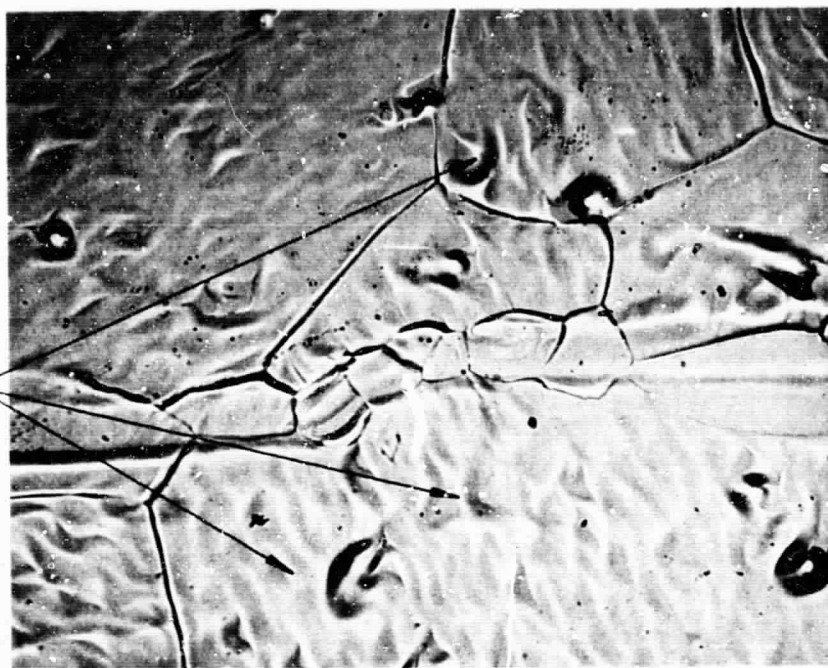
Figure 2. 500X Photomicrograph of Diamond Lapped Vapor-Deposited Rhenium, Sample II, After 2 Hours of Vacuum Outgassing at 2270°C and 60 Hours of Operation at 1900°C
