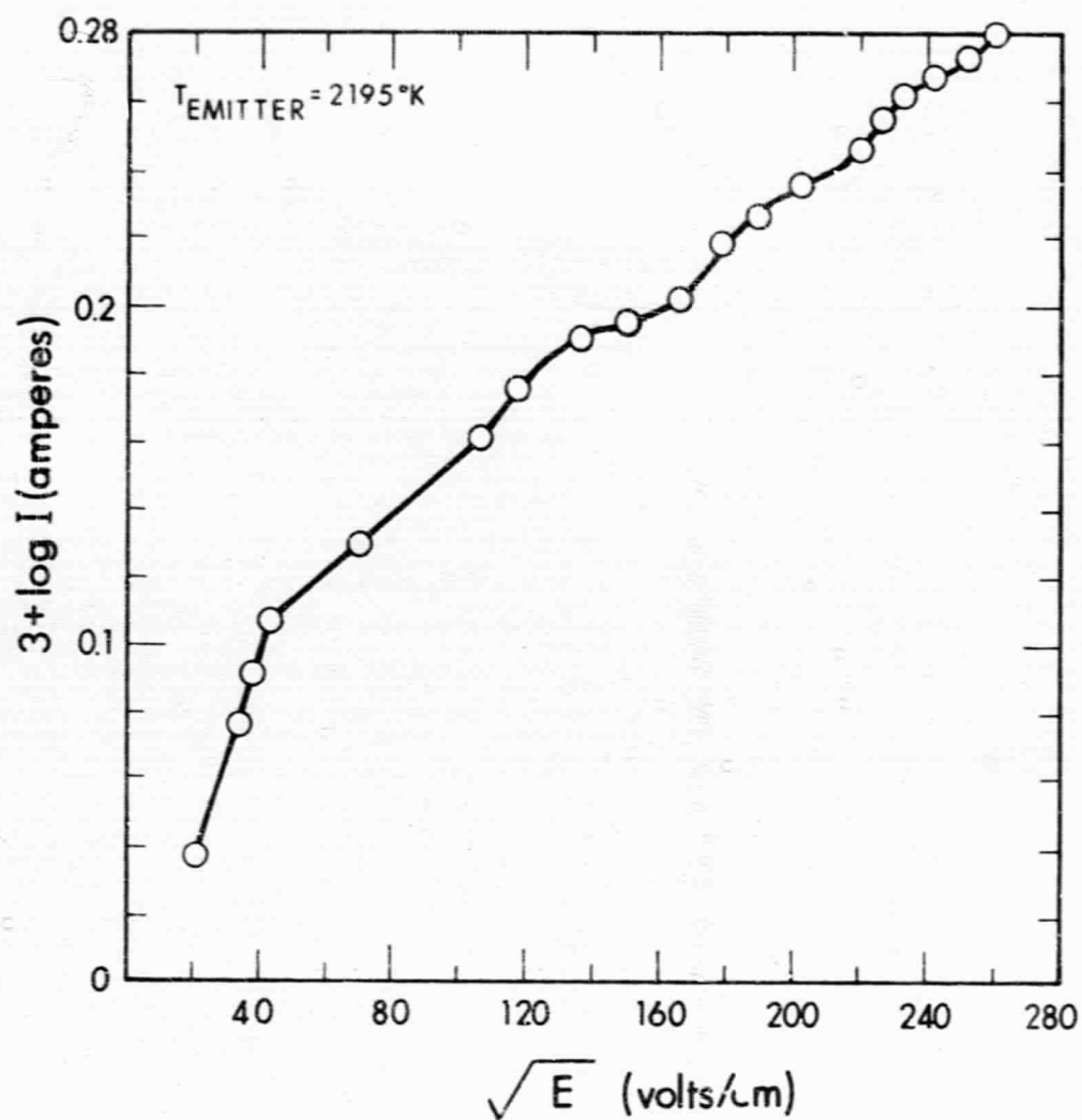
Figure 13. Periodic-Type Variations in a Schottky Plot of Electron Emission
