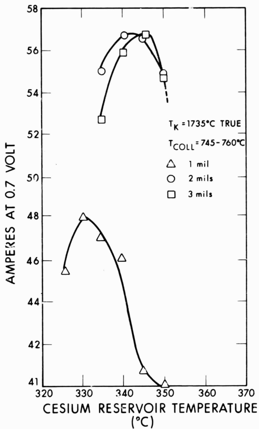
Figure 48. Converter Optimization at 0.7 Volt. Temperature of Collector 745 to 760°C (all dc data points)
