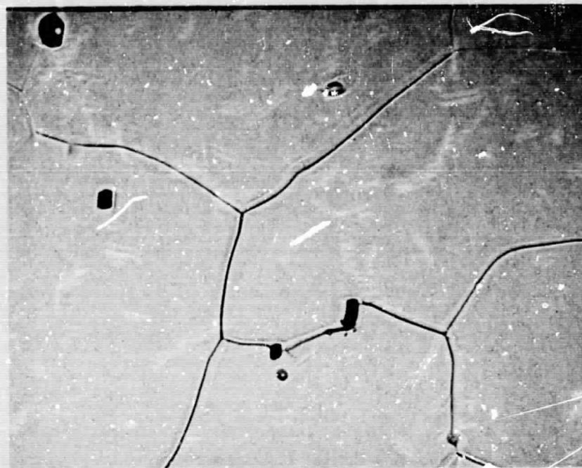
Figure 3. 500X Photomicrograph of Polished Vapor-Deposited Rhenium after 2 Hours of Vacuum Outgassing at 2250°C and 58 Hours of Operation at 1900°C
