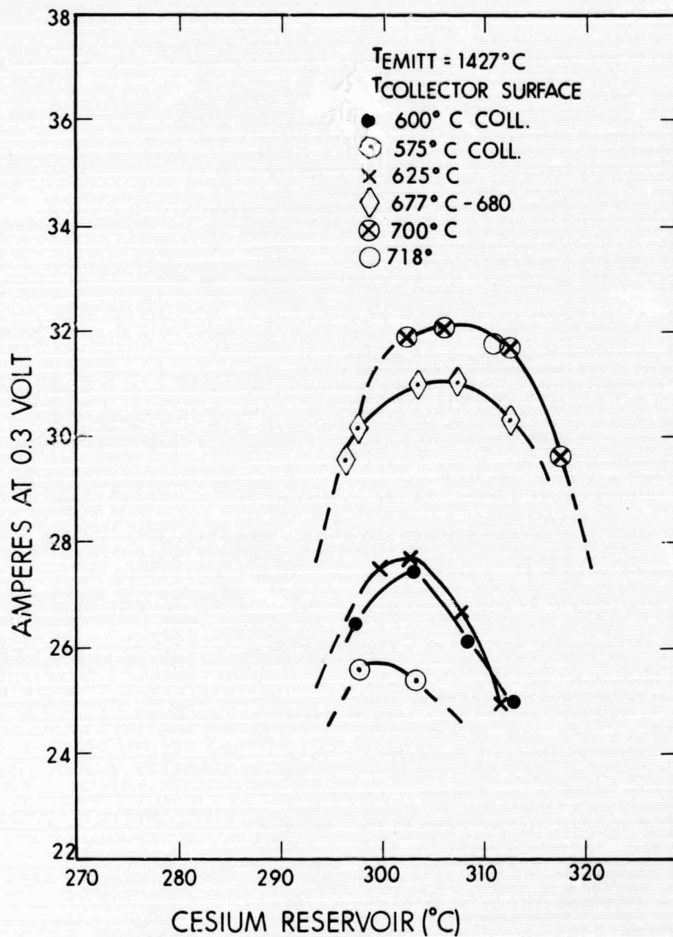
Figure 64. Converter SN-110 Performance, Optimized for a T_{\text{emitter}} of 1427^{\circ}\text{C} and Voltage Output of 0.3 Volt
