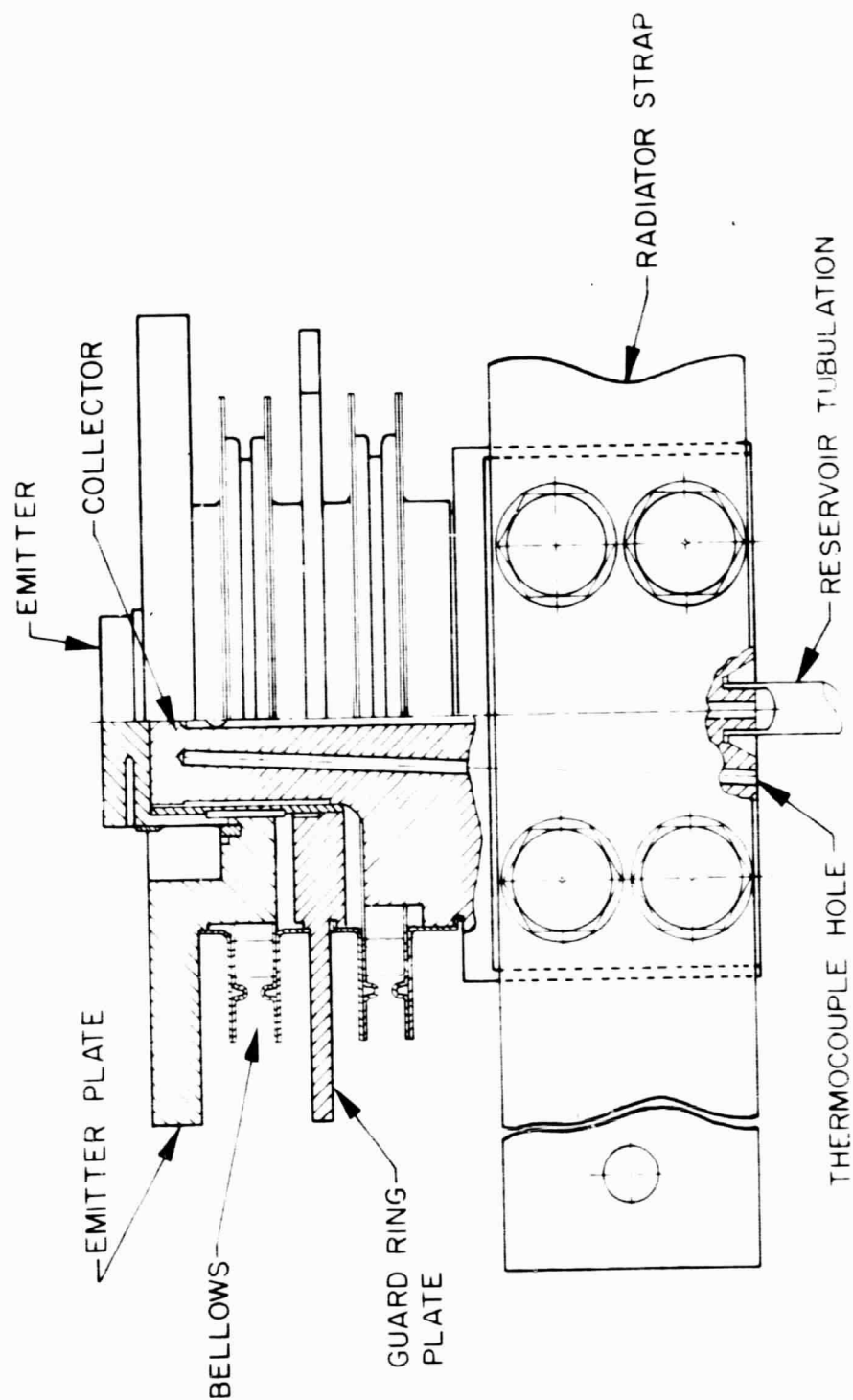
Figure 35. Variable Parameter Test Vehicle, Basic Design
