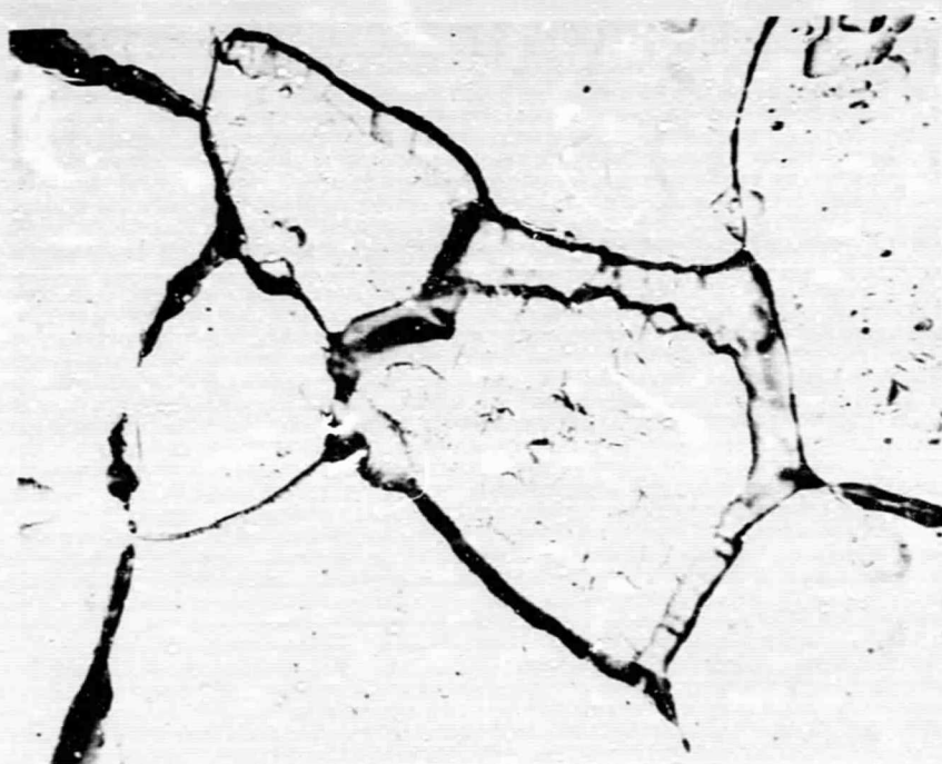
Figure 5. 500X Photomicrograph of Rough Diamond Lapped Vapor-Deposited Rhenium after Electroetching (see Fig. 4)
