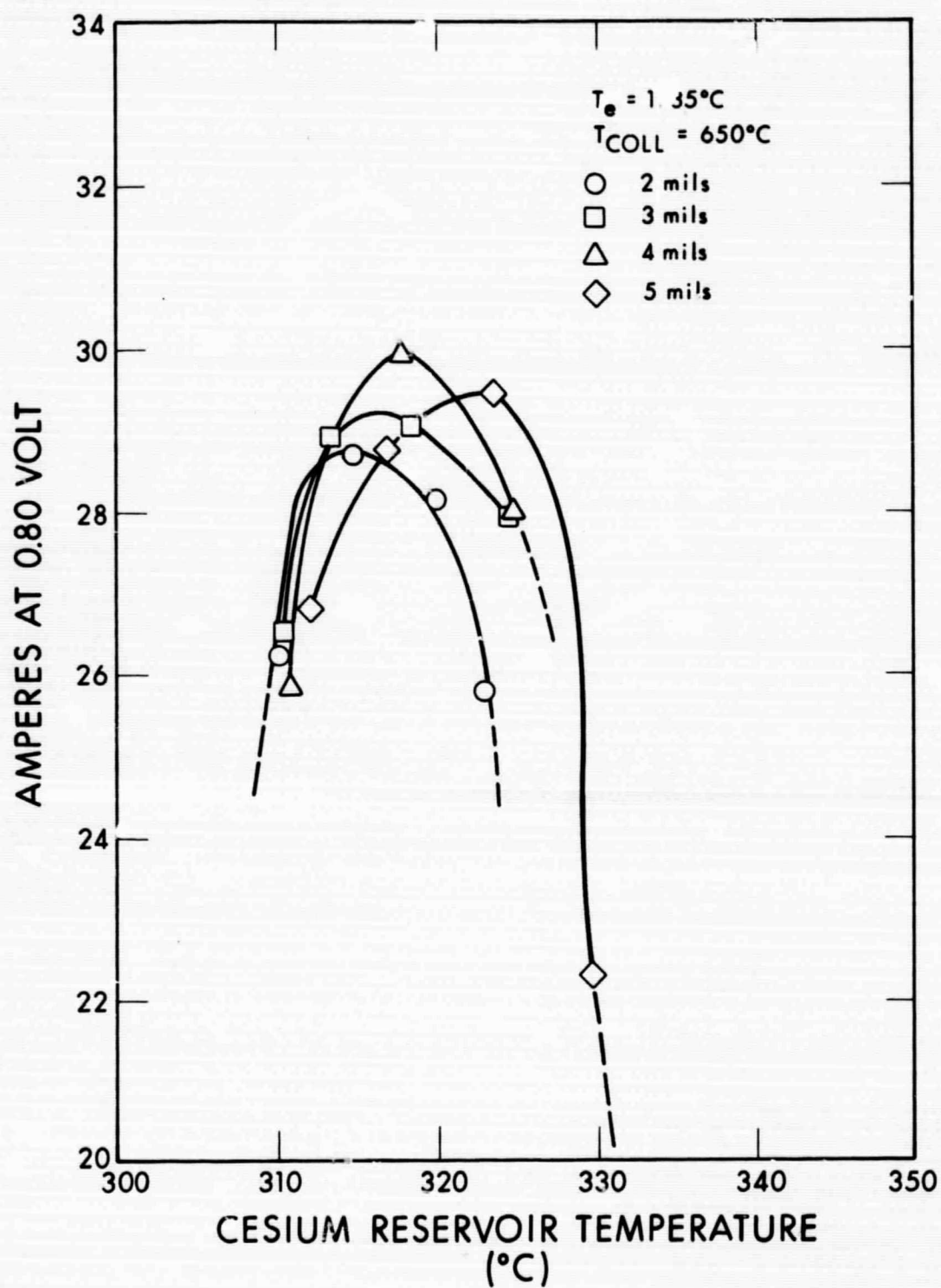
Figure 50. Converter Optimization at 0.80 Volt. Temperature of Collector 640 to 650°C (all dc data points)
