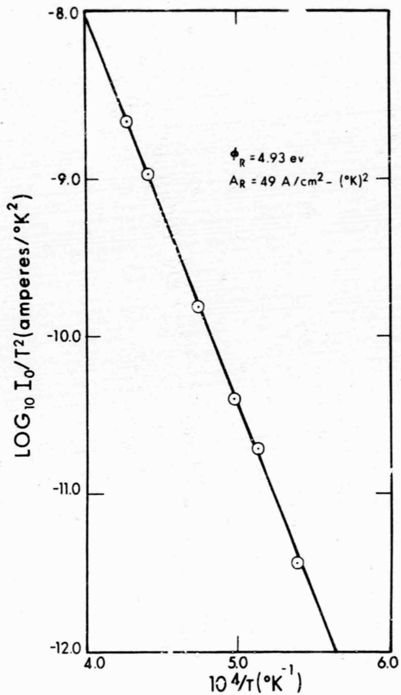
Figure 14. Richardson Plot for Vapor-Deposited Rhenium Emitter I
