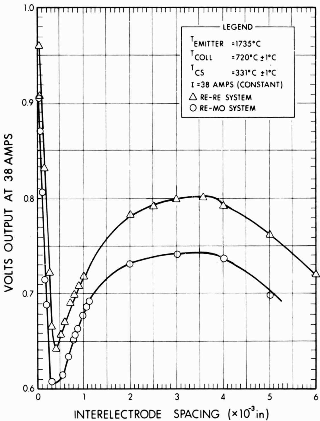
Figure 45. Comparison Plot of Re-Re System to Re-Mo System Showing Voltage Output Difference of 0.060 to 0.080 Volts Over Entire Spacing Range
