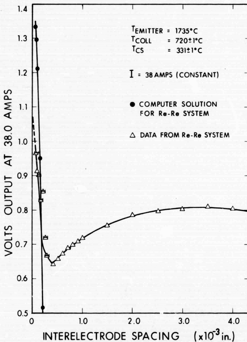
Figure 69. Comparison of Computed Results with Experimental Results
