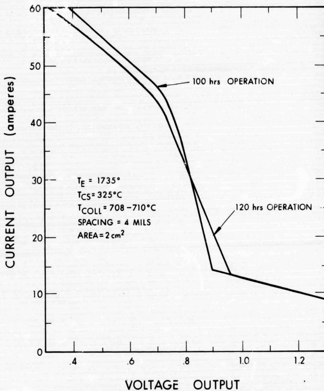
Figure 52. Vapor-Deposited Rhenium Variable Parameter Test Vehicle Characteristics Showing Shift in Performance Between 100 and 120 hours of Testing
