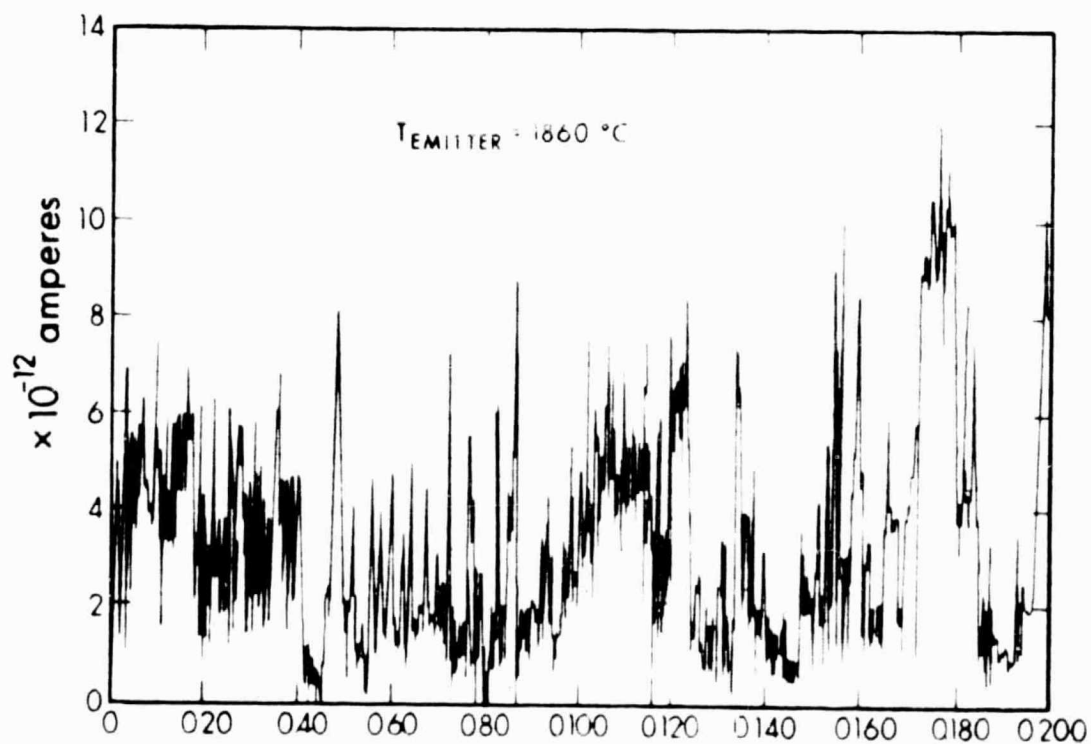
Figure 34. Emission Profile, Before and After Electro-Etching
