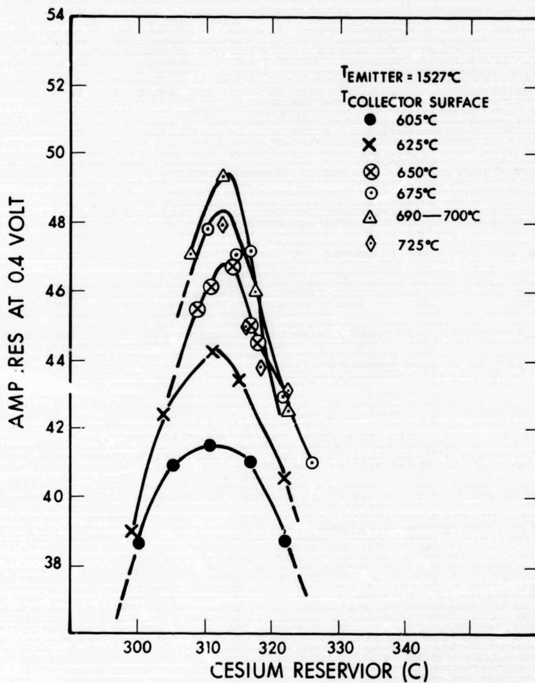
Figure 63. Converter SN-109 Performance, Optimized for a T_{\text{emitter}} of 1527^{\circ}\text{C} and Voltage Output of 0.40 Volt
