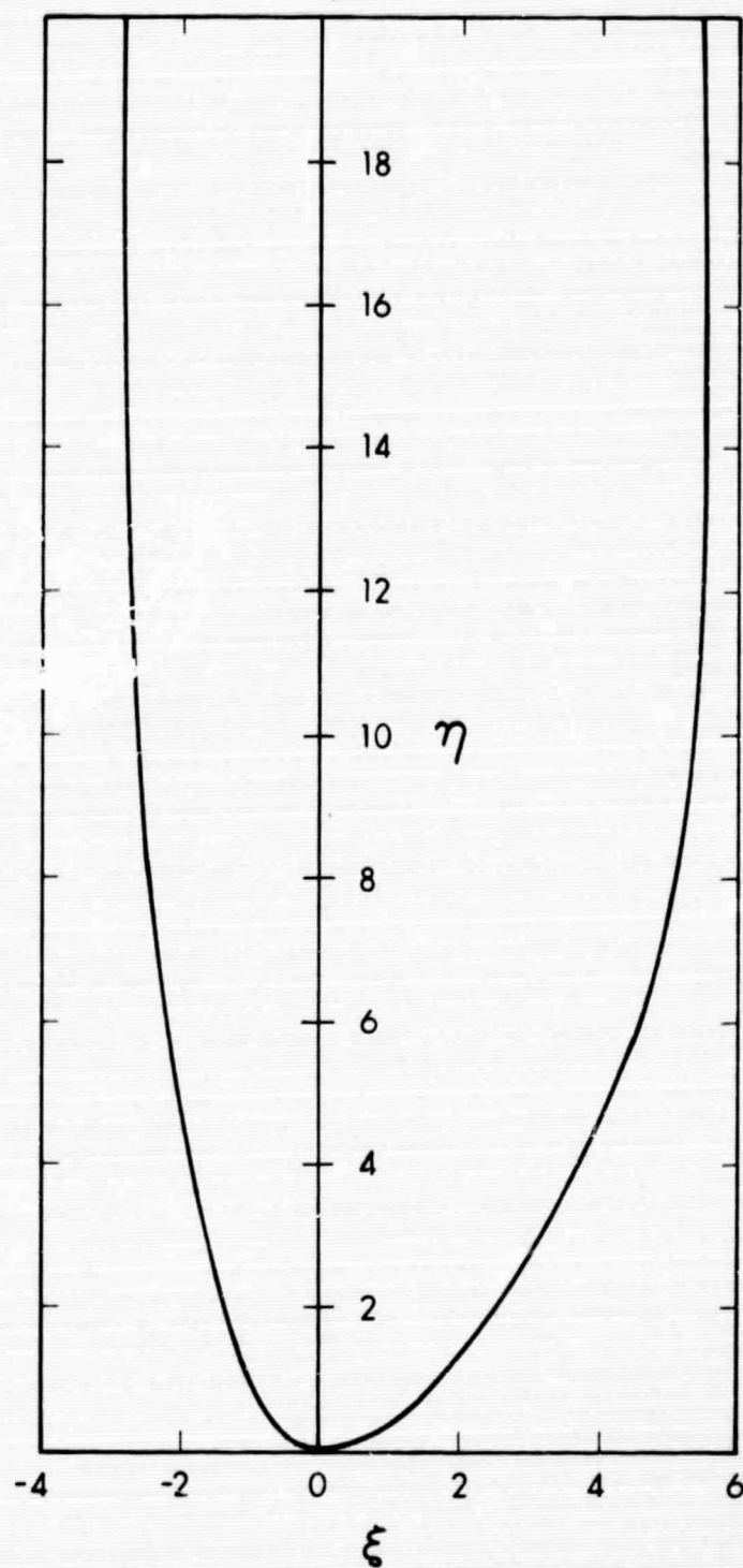
Figure 68. Normalized Potential versus Normalized Distance in the Interelectrode Space for \beta = 0 ( \beta is defined in the text)
