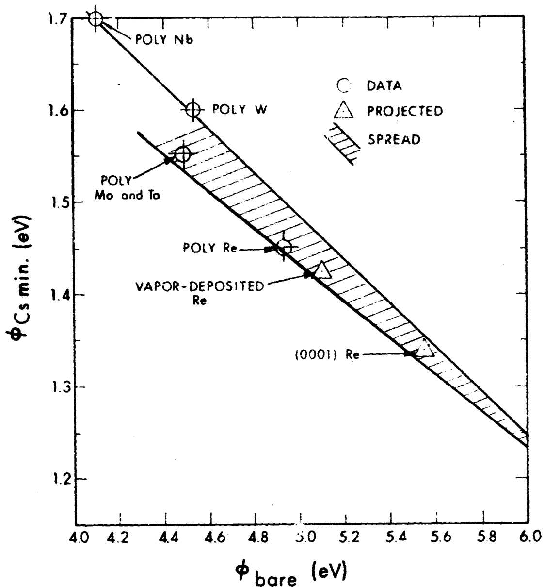
Figure 1. Empirical Relationship Between Bare Work Function, \phi_{\text{bare}} , and Minimum Cesium Work Function, \phi_{\text{Cs}}
