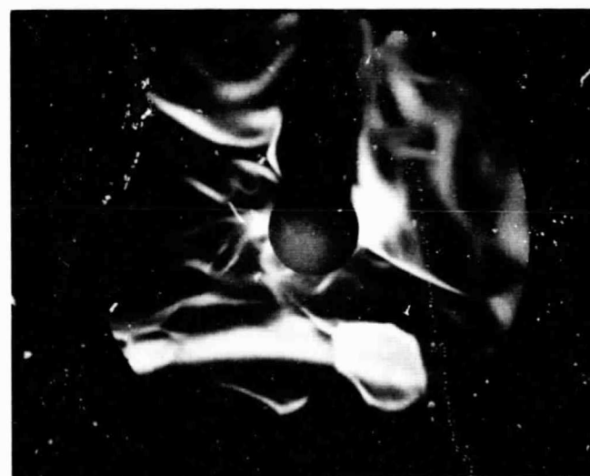
Figure 24. Recrystallization History of Selected Areas Along a Scribed Surface Before and After Secondary (Preferential) Recrystallization of Vapor-Deposited Rhenium (662X)
