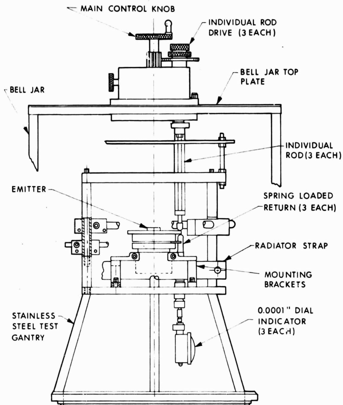
Figure 37. Variable Parameter Test Vehicle and Precision Drive Mechanism
