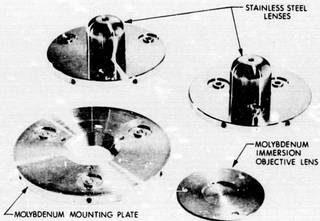
Figure 19. Lenses and Mounting Plate for Thermionic Electron Emission Microscope
