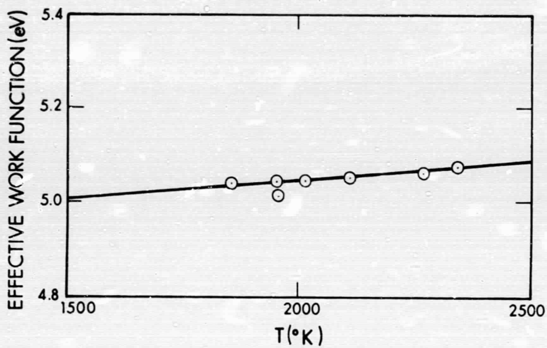
Figure 15. Effective Work Function versus Emitter Temperature for Vapor-Deposited Rhenium Emitter I
