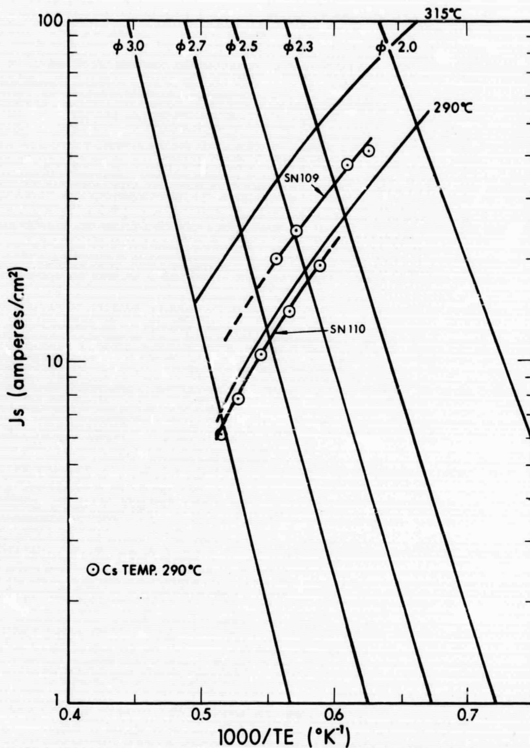
Figure 62. Comparison of Saturated Electron Emission from Polycrystalline Rhenium and Converters SN-109 and SN-110
