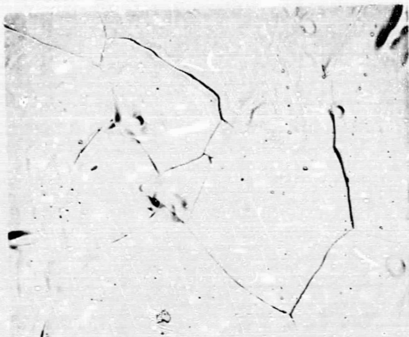
Figure 4. 500X Photomicrograph of Rough Diamond Lapped Vapor-Deposited Rhenium after 2 Hours of Vacuum Outgassing at 2270°C and 40 Hours of Operation at 1900°C
