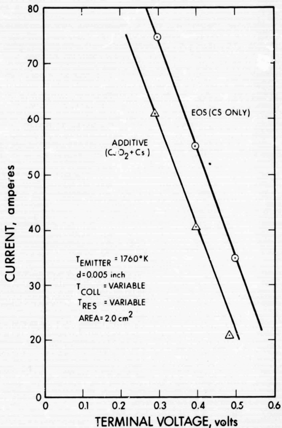
Figure 46. Optimized Performance Plot Comparing Additive Data to EOS Nonadditive Data
