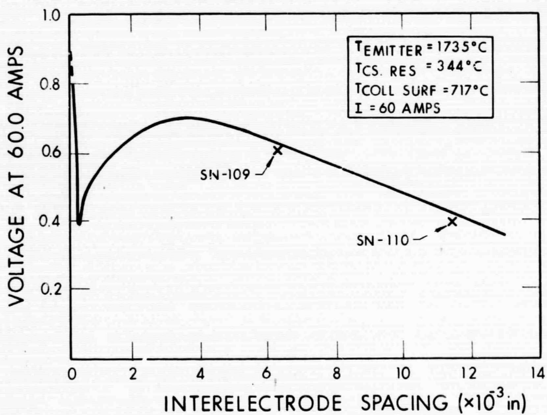
Figure 61. Comparison of Polycrystalline Rhenium Test Vehicle Performance to SN-109 and SN-110
