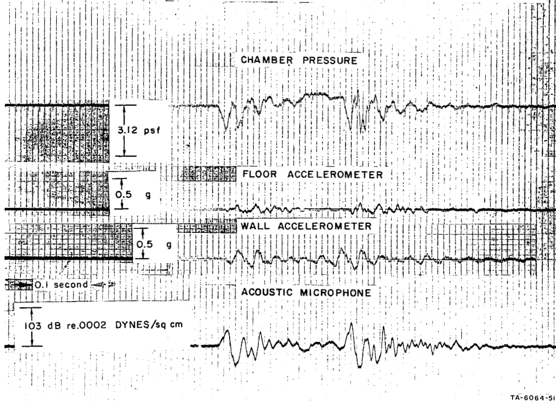
FIG. 5 CHAMBER PRESSURE (1000 Hz Low Pass Filter), ACCELEROMETER, AND INDOOR ACOUSTIC MICROPHONE TRACINGS DURING A 1.6 PSF SIMULATED SONIC BOOM
