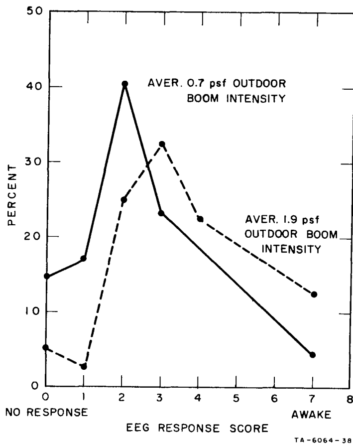
FIG. 14 STAGE 2 EEG RESPONSE TOWARD MORE AWAKENING AS FUNCTION OF SIMULATED BOOM INTENSITY
