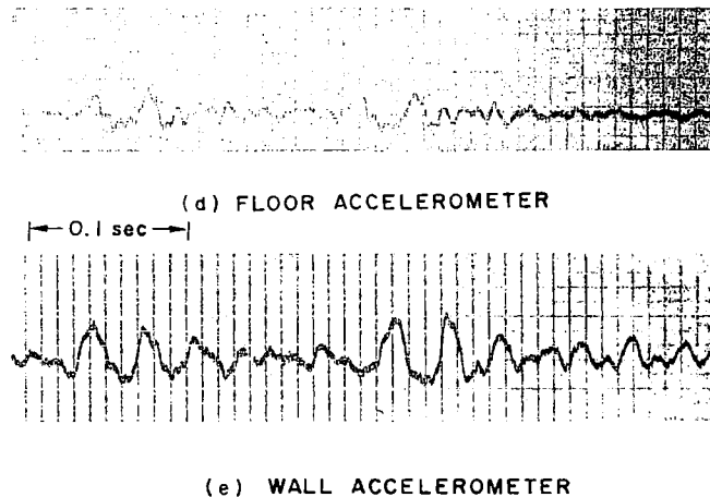
FIG. 8 ACCELERATIONS INDUCED BY AN ACTUAL B-58 SONIC BOOM IN A HOUSE AT EDWARDS AIR FORCE BASE (Ref. 4, Pg. G-II-33) AND BY A SIMULATED SONIC BOOM IN THE TEST ROOM FOR VARIOUS TRANSDUCER LOCATIONS
