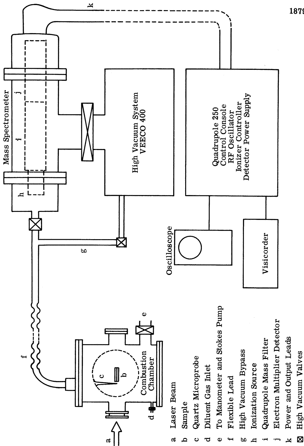
Figure 2b. Composition Probe Apparatus.
