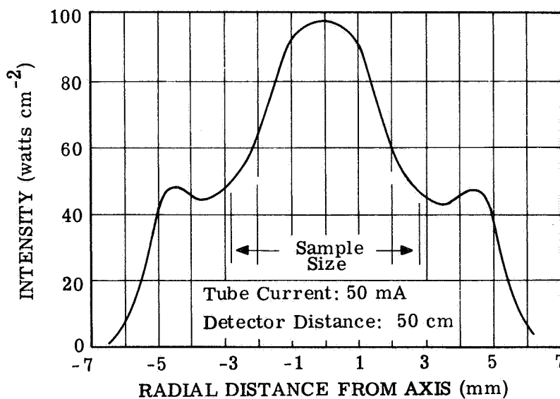
Figure 1. Laser Output Power and Intensity Distribution.
