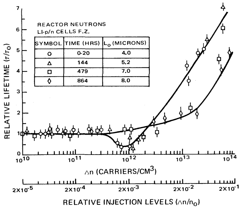
Figure 28. Relative Lifetime vs. Excess Carrier Density for F.Z. Cells Bombarded by Reactor Neutrons
