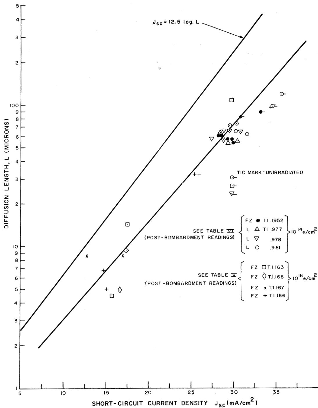
Figure 33. Diffusion Length as a Function of Short-Circuit Current for GFE Cells Before and After Irradiation by 10^{14} e/cm 2 or 10^{16} e/cm 2
