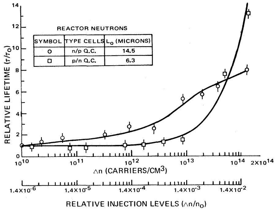
Figure 27. Relative Lifetime vs. Excess Carrier Density for Q.C. n/p and p/n Control Cells Bombarded by Reactor Neutrons
