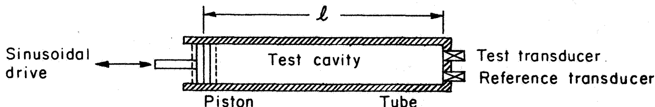
FIGURE 2. PISTON-IN-CYLINDER GENERATOR.
