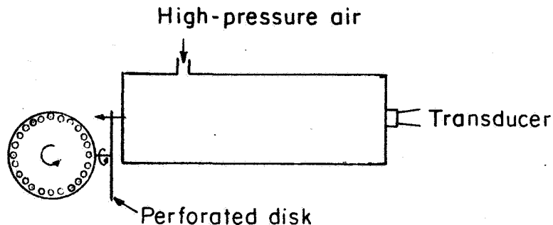
FIGURE 1. SIREN-TUNED-CAVITY GENERATOR.
