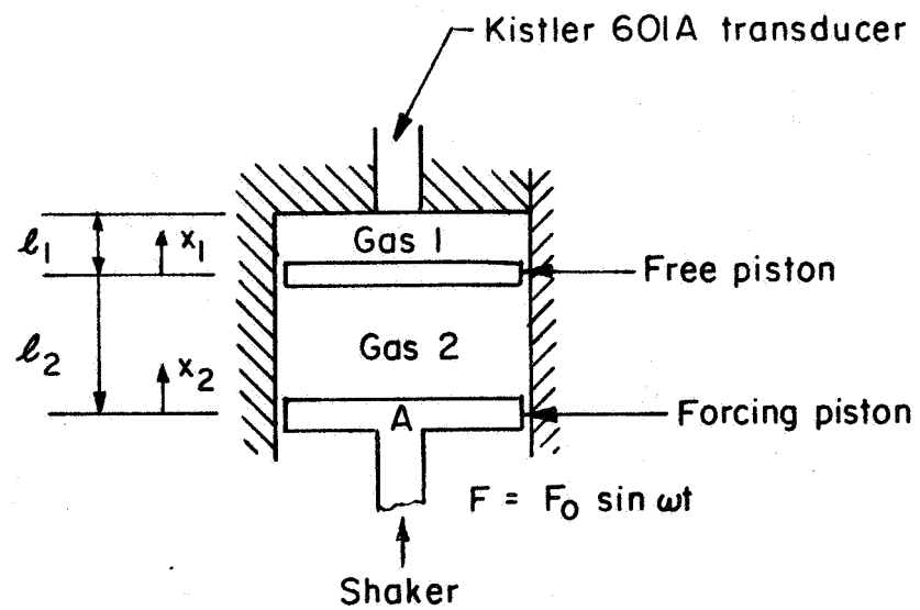
FIGURE 6. DOUBLE-PISTON GENERATOR
