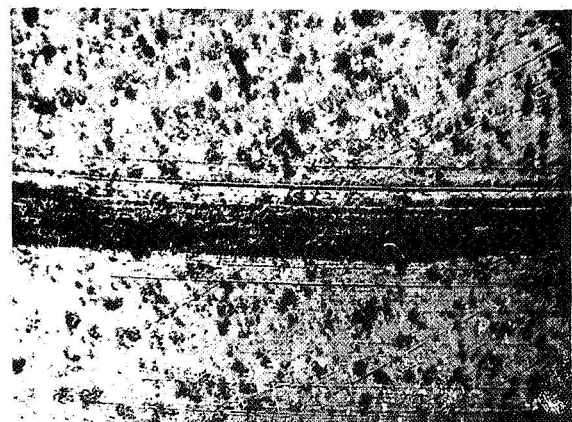
Figure 6 - Wear track in plasma-arc deposited \text{Al}_2\text{O}_3 (150X)
