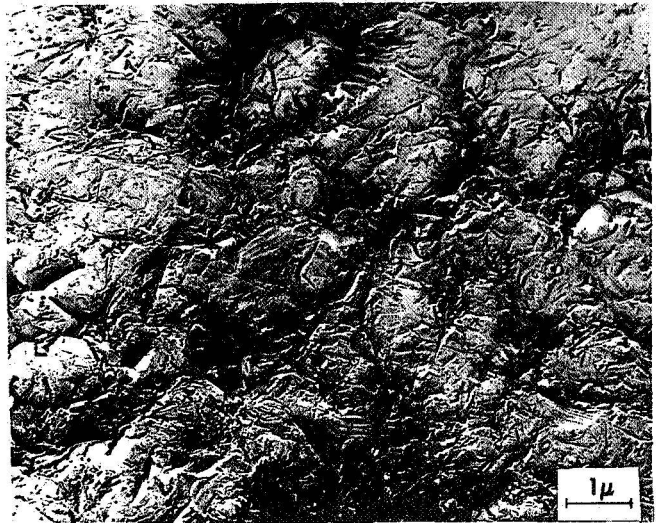
Figure 5 - As-received Carboloy surface, negative replica
