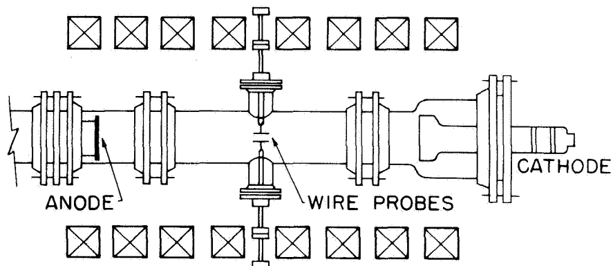
(a) SET-UP
