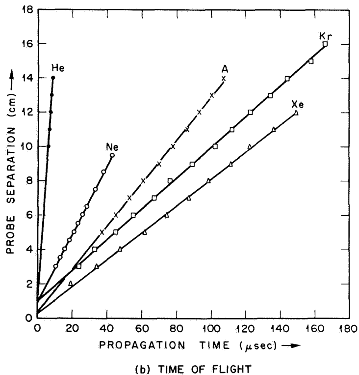
FIG. 8. LONGITUDINAL WAVE PROPAGATION: ION ACOUSTIC WAVES ( T_e \gg T_i ) (after Jones and Alexeff).
