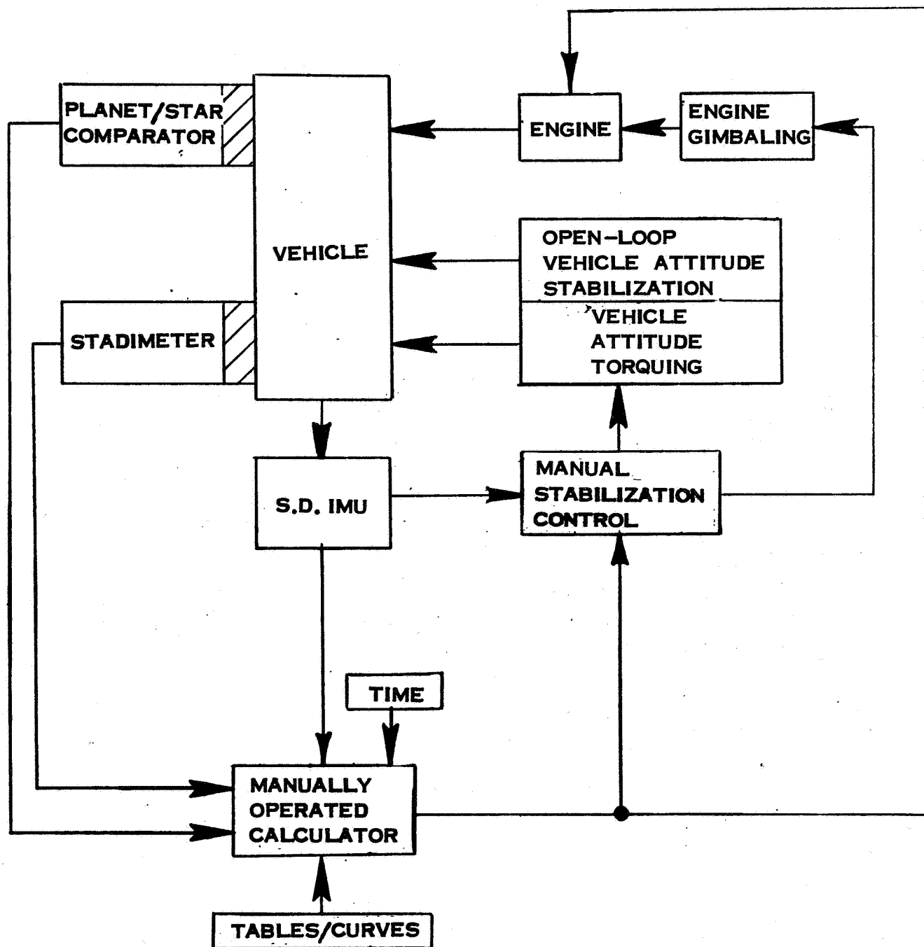
Figure 5-13. Aided-Manual Post and Terminal Adjustment
