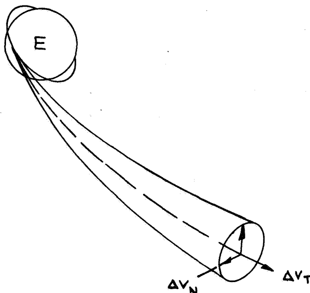
Figure 4-3. Cis-Martian Injection
