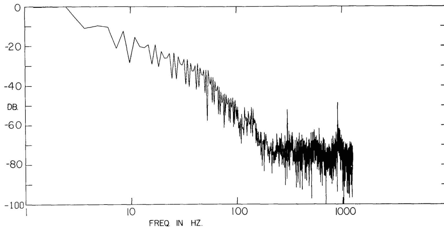
Figure 16 Spectral Energy Characteristics of Idealized 350 ms. Duration N-Wave @ Rise Time = 10 ms. as Used in Series I Tests.
