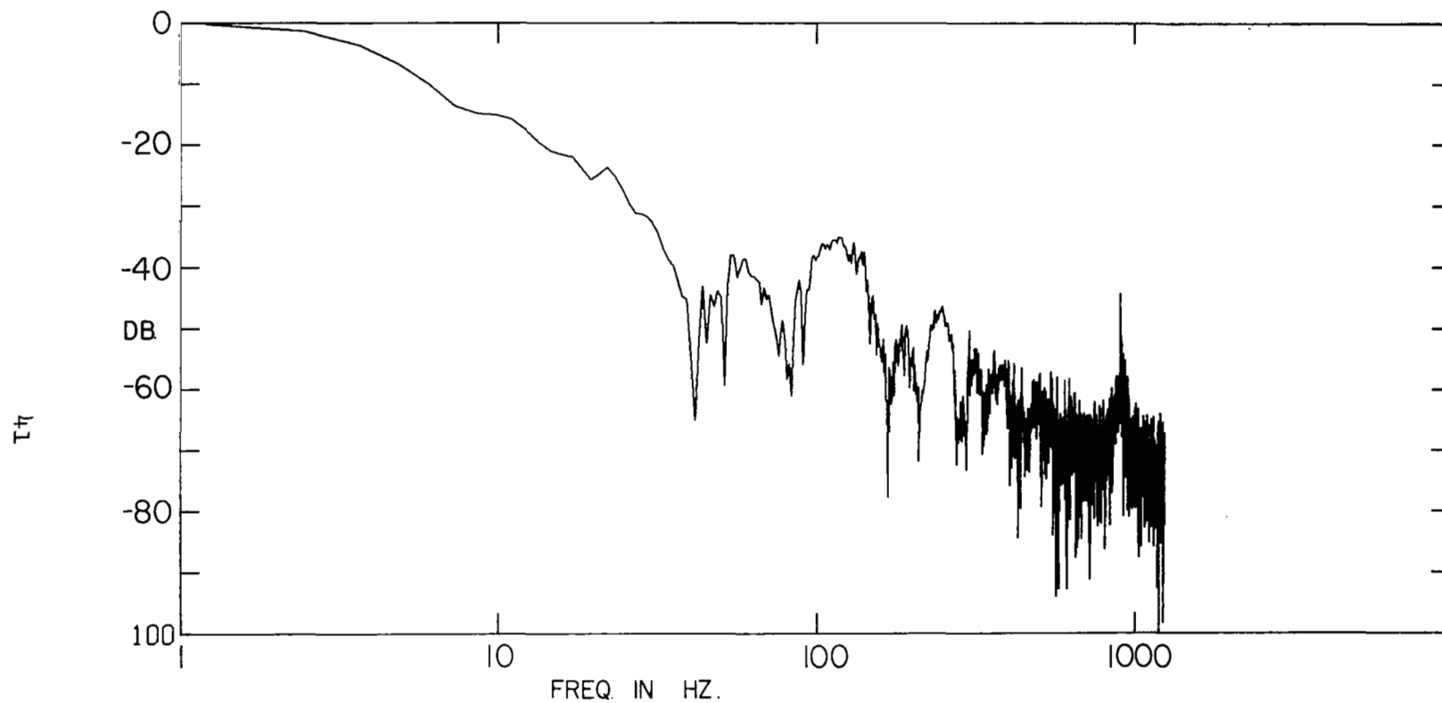
Figure 21 Spectral Energy Characteristics of Idealized 150 ms. 1/2 N-"Sawtooth" Wave @ Rise Time of 1 ms. With Interpeak Duration of 8 ms. as Used in Series III Tests. (Type 1)
