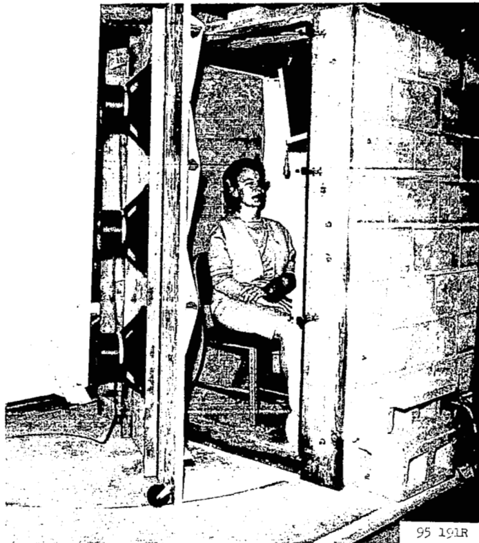
Figure 1. Sonic Boom Simulation Chamber - Note Hinged Wall Access.
