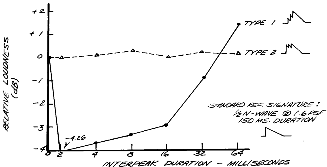
FIGURE 12. RELATIVE LOUDNESS OF \frac{1}{2} N-WAVES (TYPES 1 & 2) WITH DIFFERENT "SAWTOOTH" SPACING - SERIES III -
