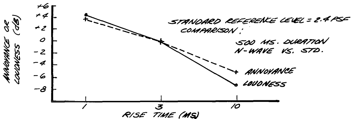
FIG. 10. RELATIVE ANNOYANCE & LOUDNESS VS. RISE TIME - SERIES I -
