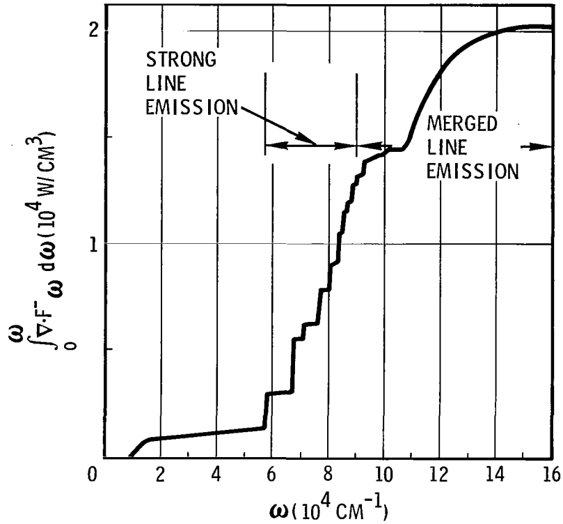
Figure 9. The Integrated \nabla \cdot \vec{F}^- for Shock-Layer Radiation Traveling Toward the Cold Wall, Evaluated 0.04 cm from the Shock
