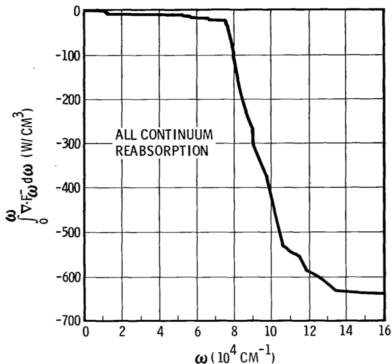
Figure 11. The Integrated \nabla \cdot \vec{F}_\omega for Shock-Layer Radiation Traveling Toward the Cold Wall, Evaluated 0.11 cm from the Wall
