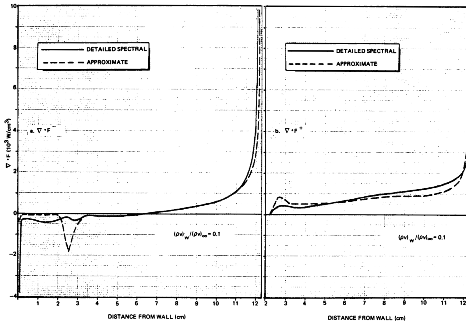
Figure 17. The Divergence of Shock-Layer Radiation Split into its Left-Moving and Right-Moving Components, Compared to Approximation using Continuum-Dominant Reabsorption Model Bu_p = 0.000018 , Bu_L = 0.0075 (Case of Massive Blowing)
