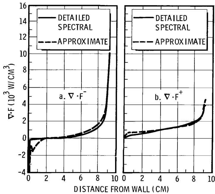
Figure 13. The Divergence of Shock-Layer Radiation Split into its Left-Moving and Right-Moving Components, Compared to Approximation Using Line-Dominant Reabsorption Model. Bu_P = 0.00004 , Bu_L = 0.008
