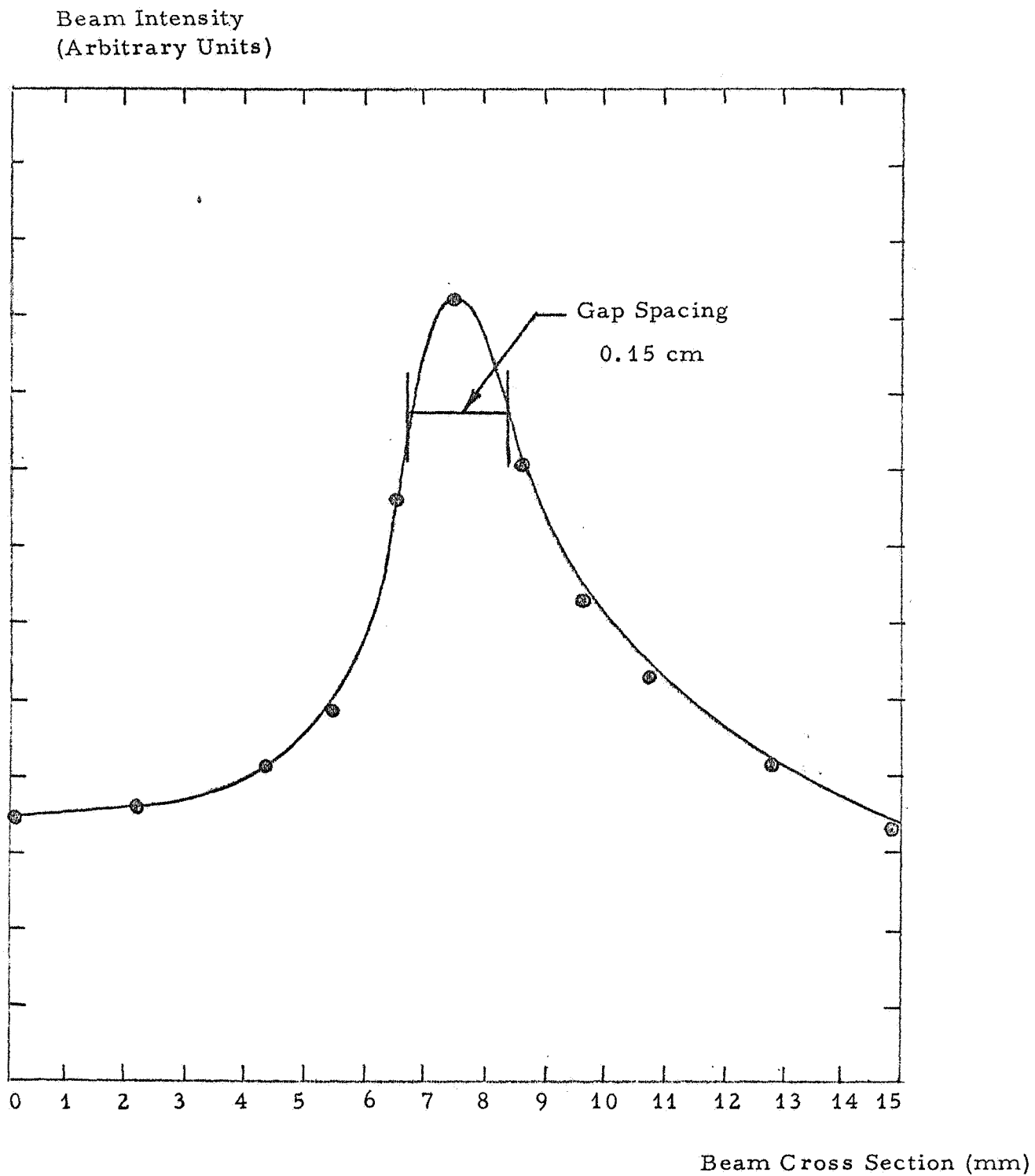
MOLECULAR BEAM PROFILE
