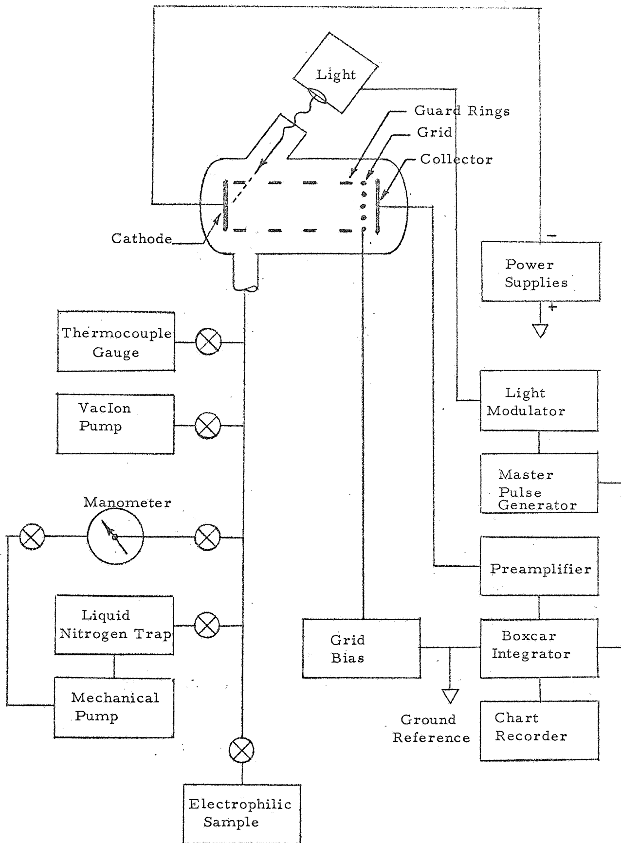
SCHEMATIC DIAGRAM OF DRIFT CHAMBER
