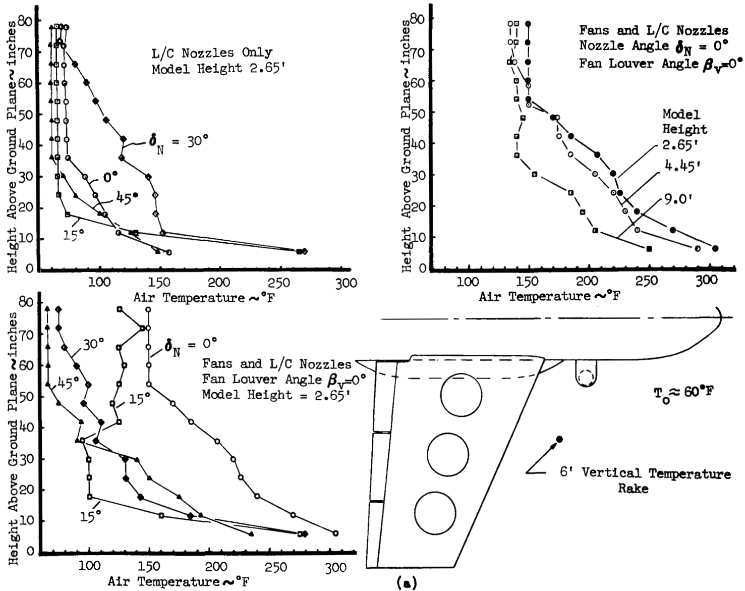
Figure 48. Six Foot Vertical Rake Temperatures
