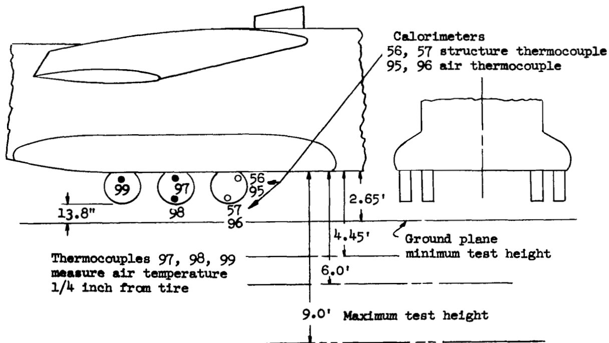
Figure 7. - Landing Gear Thermocouples.
