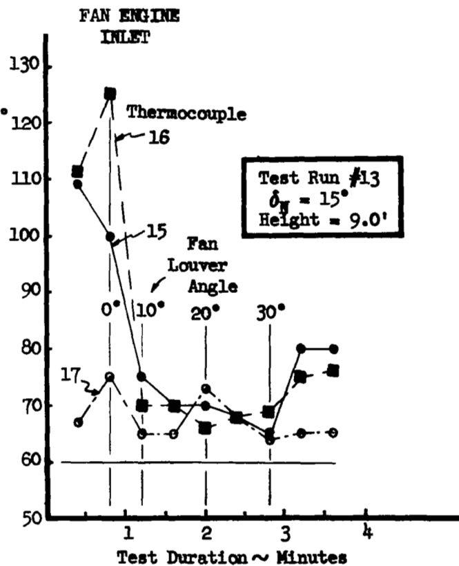
Figure 45. Engine Inlet Air Temperature Versus Time, \delta_N = 15^\circ , h = 9.0 Ft.
