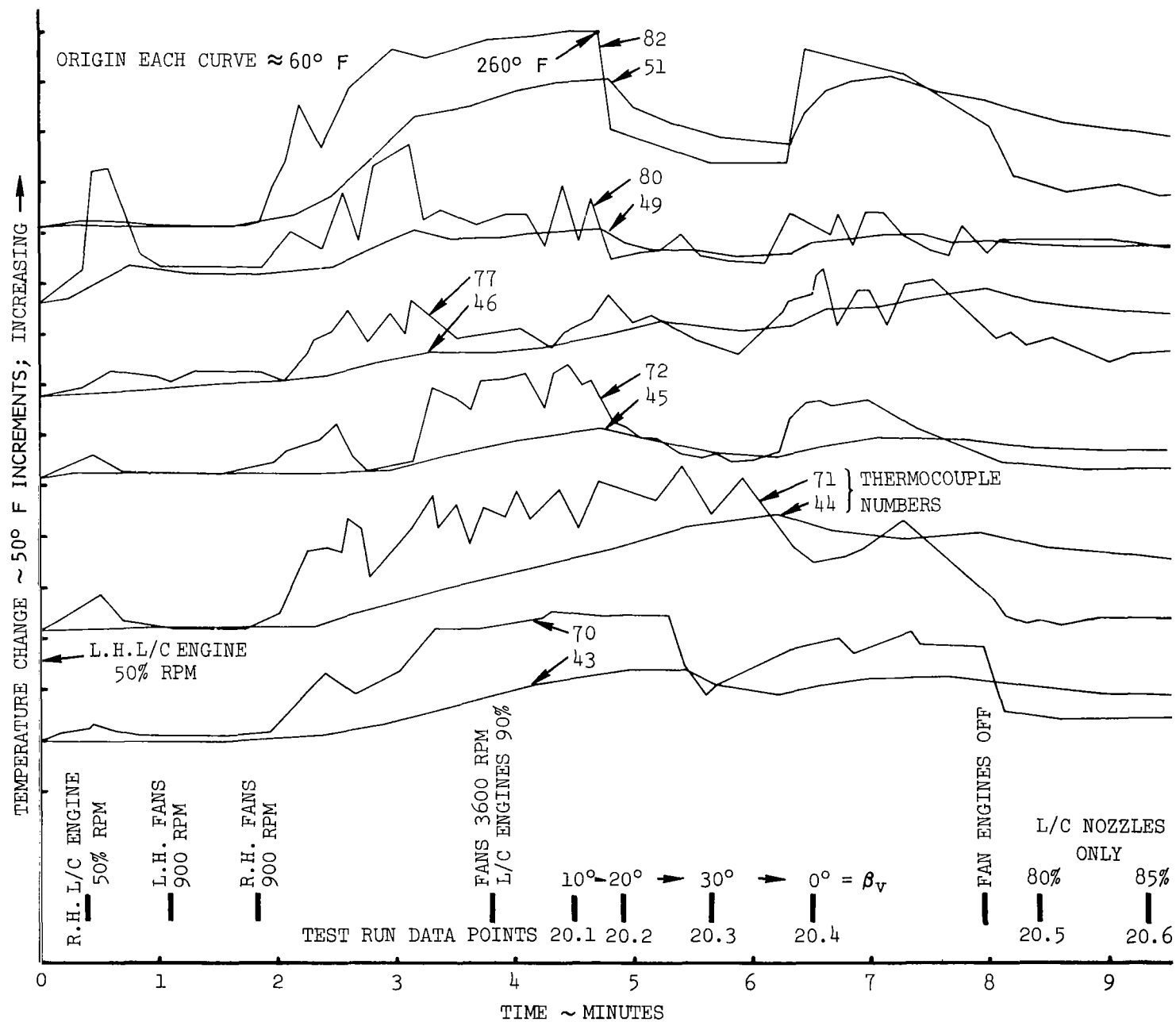
Figure 61. - Wing and Fuselage Air and Structure Temperature Traces; \delta_N = 30^\circ , h = 2.65 \text{ Ft}
