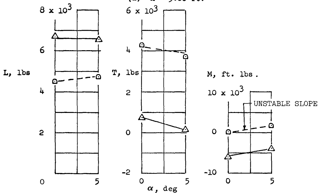
Figure 13. Effect of Angle of Attack, Six Fans at 3600 RPM, L/C Power Off, Wheel Fairings On
