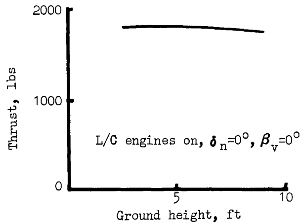
Figure 36. Variation of Right-Hand Center Fan Thrust With Model Ground Height and Fan Exit Louver Angle, Six-Fan Operation
