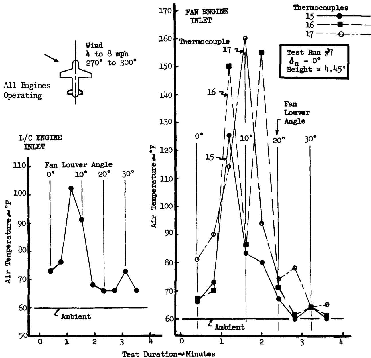
Figure 40. Engine Inlet Air Temperature Versus Time, \delta_N = 0^\circ , h = 4.45 Feet
