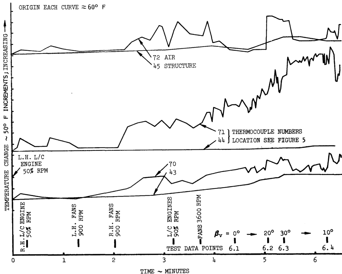
Figure 56. - Under Wing Air and Structure Temperature Traces; \delta_N = 0^\circ , h = 2.65 \text{ Ft}
