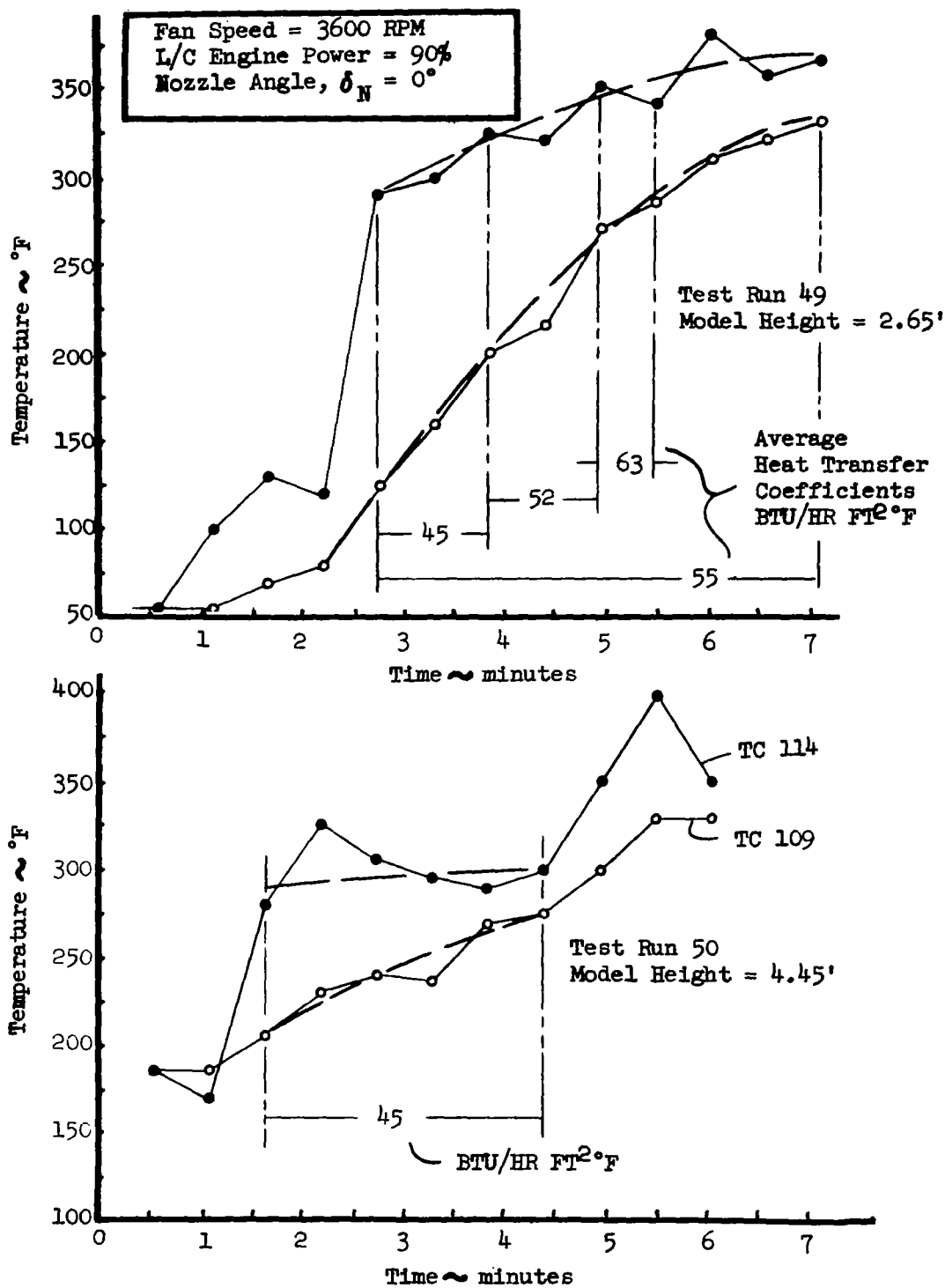
Figure 50. Ground Surface Heating Conditions - Concluded
