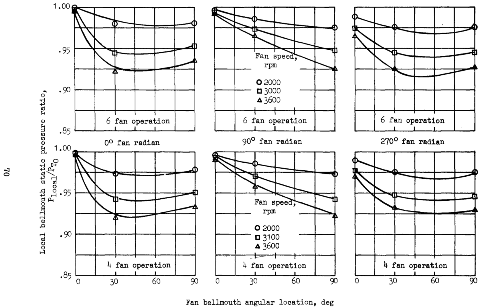
Figure 30. Fan Bellmouth Static Pressure Distributions; Right-Hand Inboard Fan, Ground Height = 2.65 Ft, L/C Engines Off, \beta_v = 0^\circ
