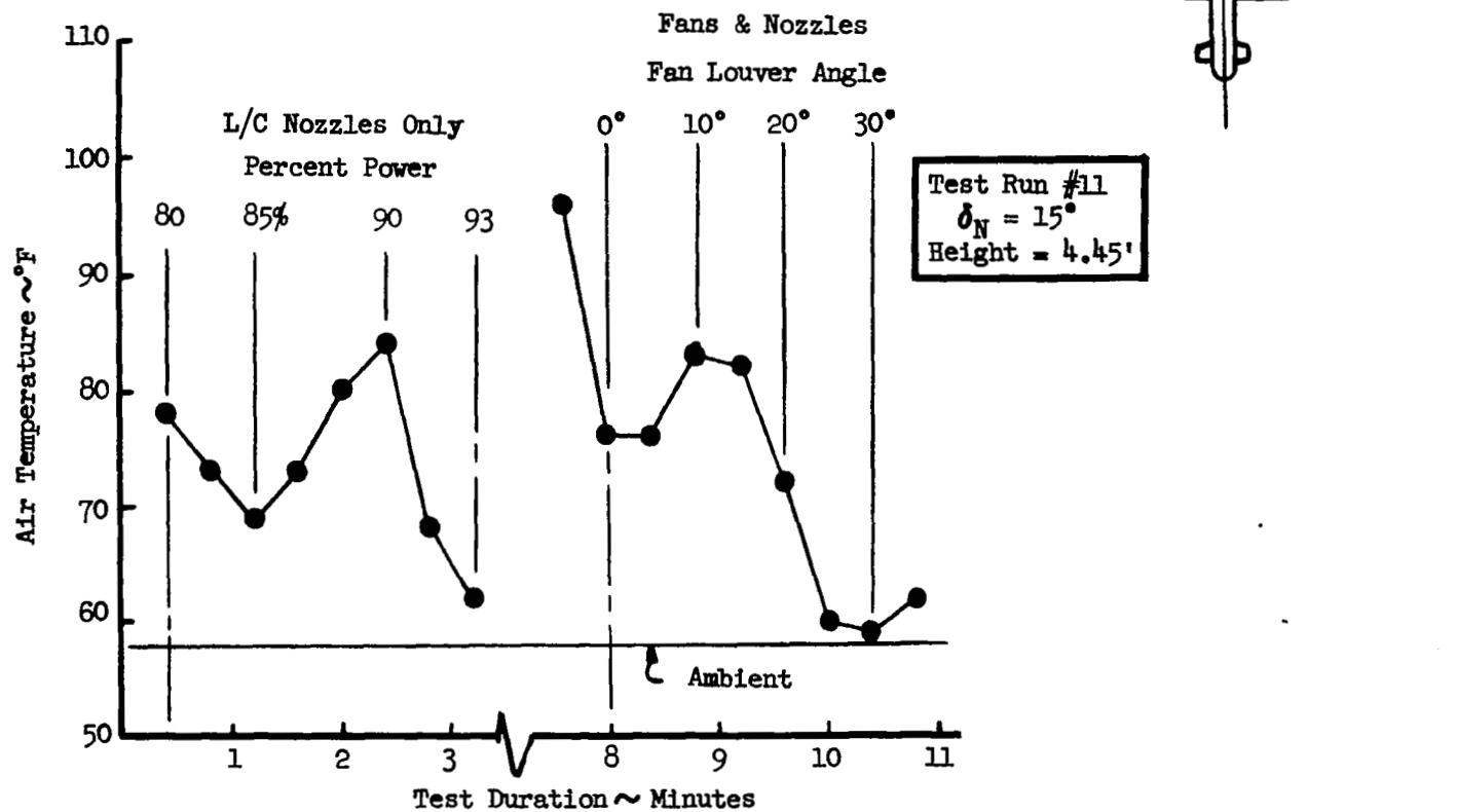
Figure 43. L/C Engine Inlet Air Temperature Versus Time, \delta_N = 15^\circ , h = 4.45 Ft.
