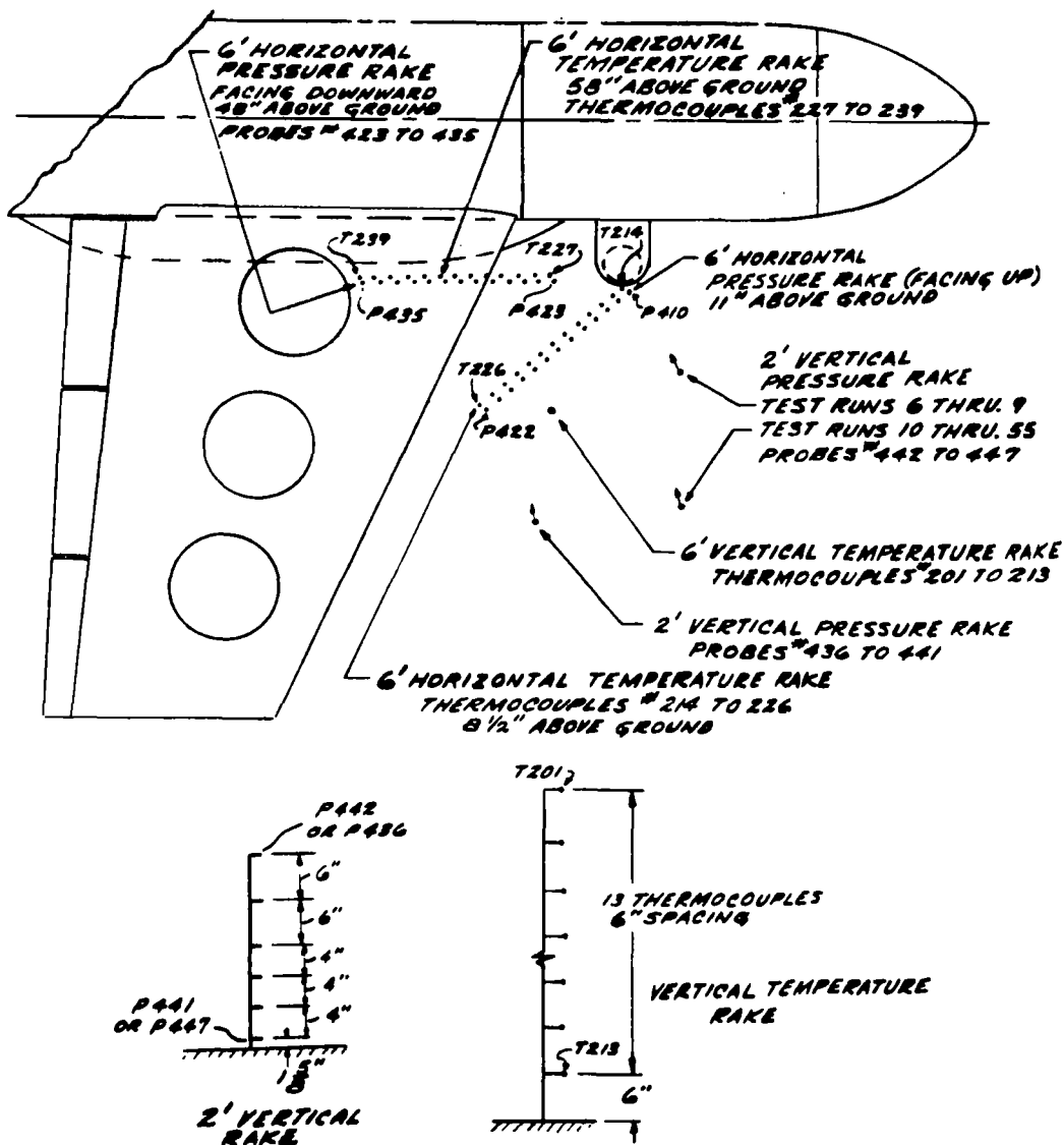
(b) Rake locations for Test Runs 6 through 55
