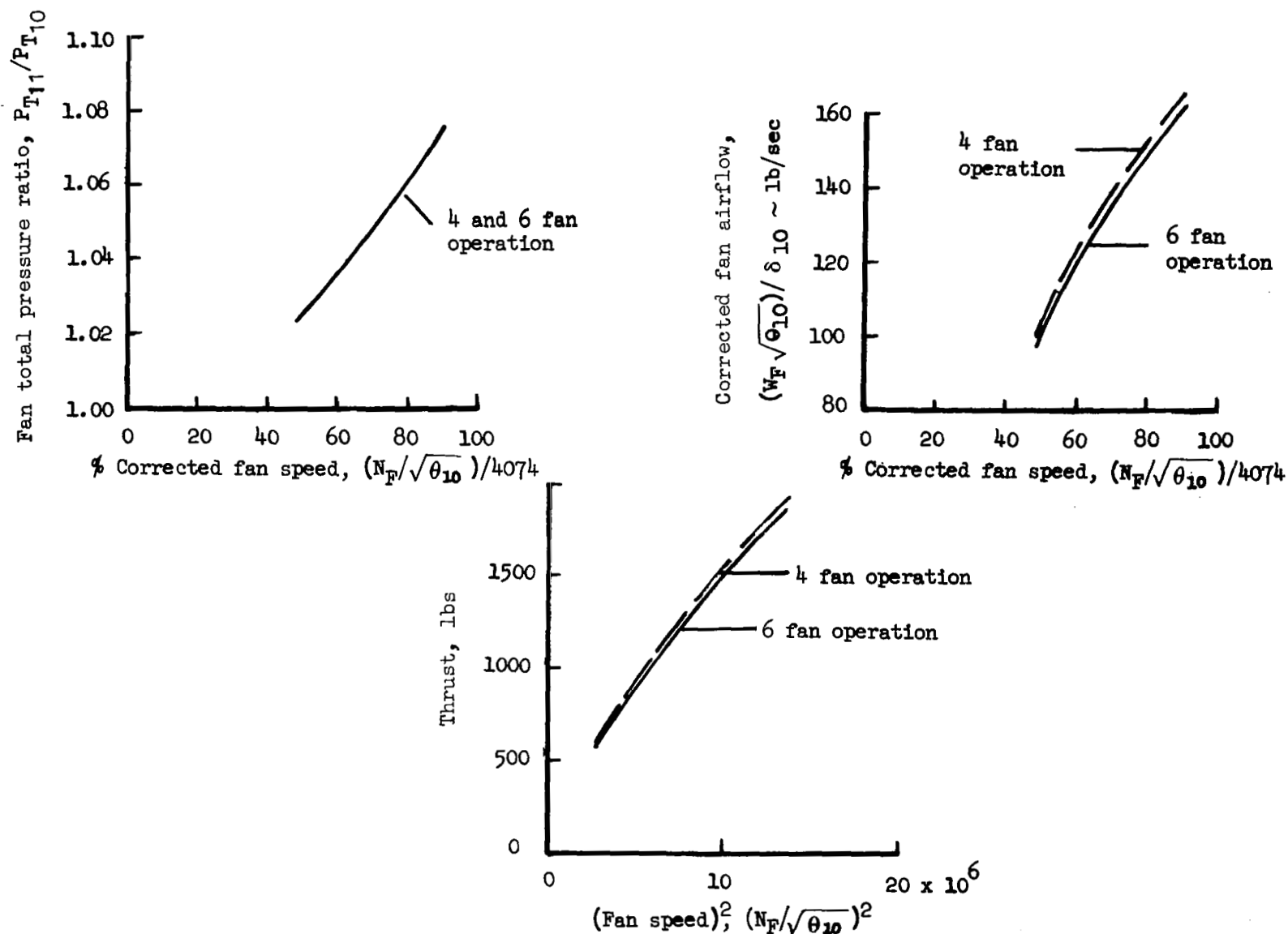
Figure 35. Fan Performance Characteristics, Right-Hand Center Fan, L/C Engines Off, Ground Height = 2.65 Feet, \beta_V = 0^\circ
