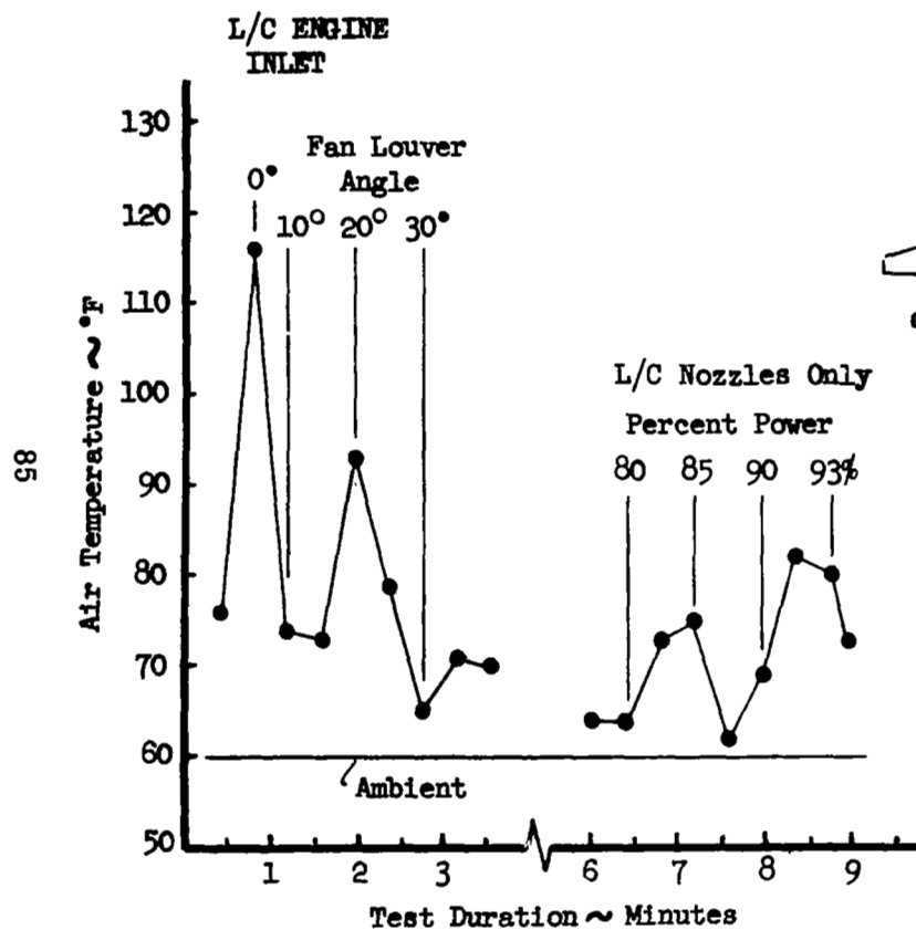
Figure 45. Engine Inlet Air Temperature Versus Time, \delta_N = 15^\circ , h = 9.0 Ft.
