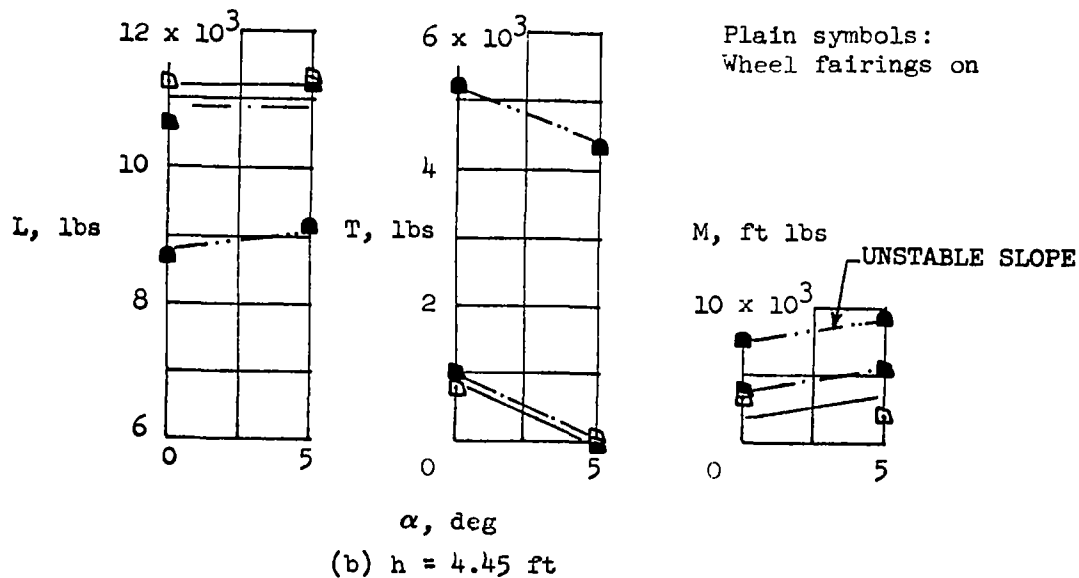
Figure 24. Effect of Angle of Attack, Fans at 3600 RPM, L/C Nozzles 90% Power, \delta_N = 0^\circ
