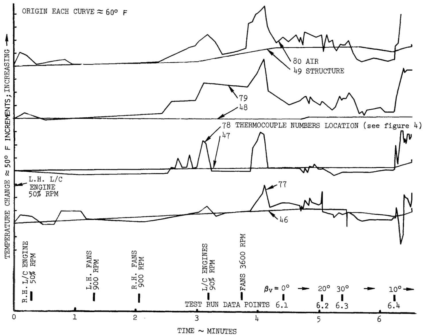
Figure 55. - Side of Fuselage Air and Structure Temperature Traces; \delta_N = 0^\circ , h = 2.65 \text{ Ft} - Concluded
