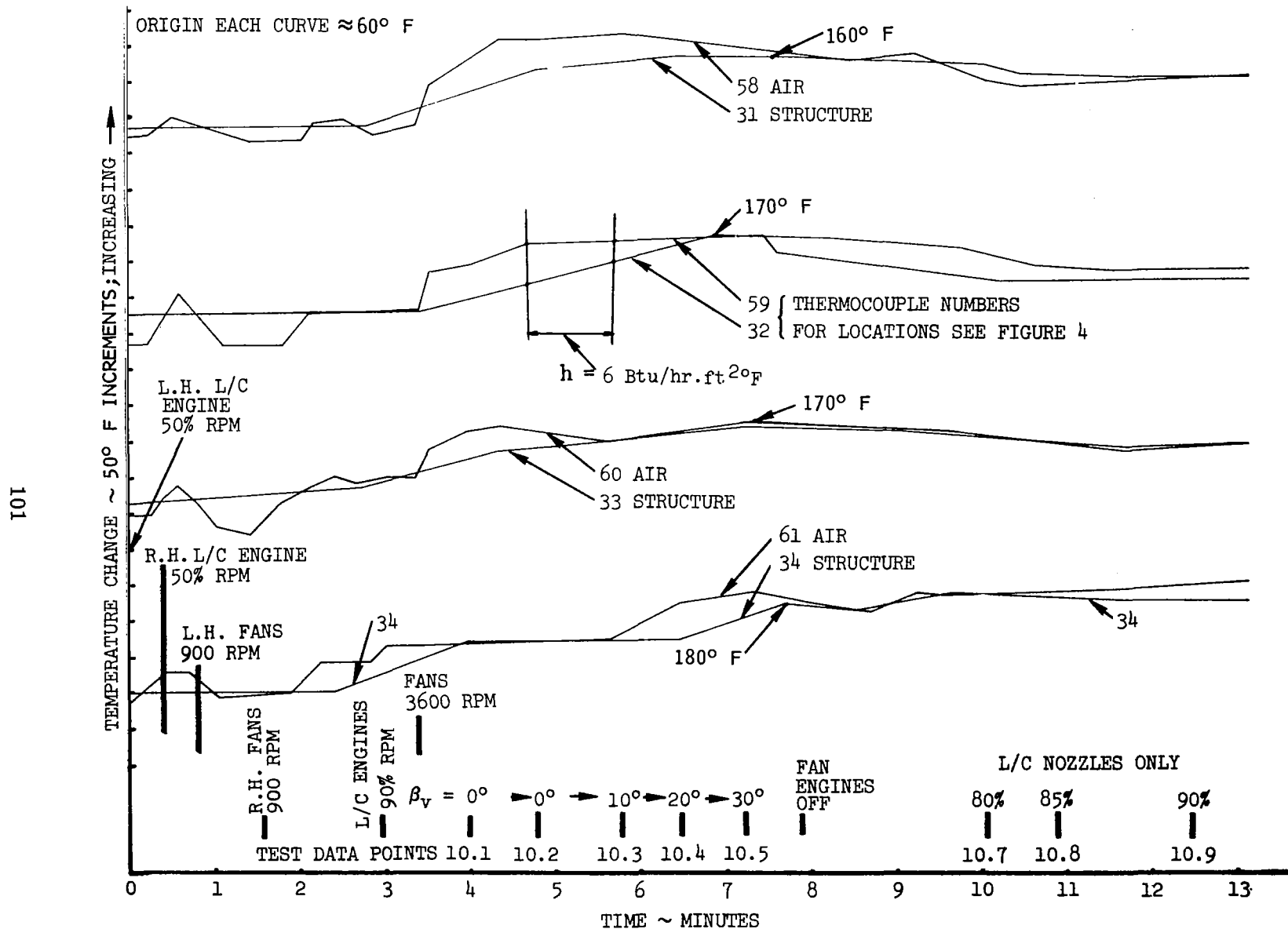
Figure 58. - Bottom of Fuselage Air and Structure Temperature Traces; \delta_N = 15^\circ , h = 2.65 \text{ Ft}
