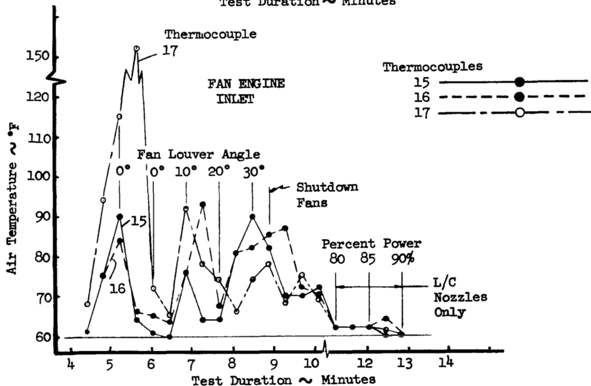
Figure 42. Engine Inlet Air Temperature Versus Time \delta_N = 15^\circ ; h = 2.65 Ft.
