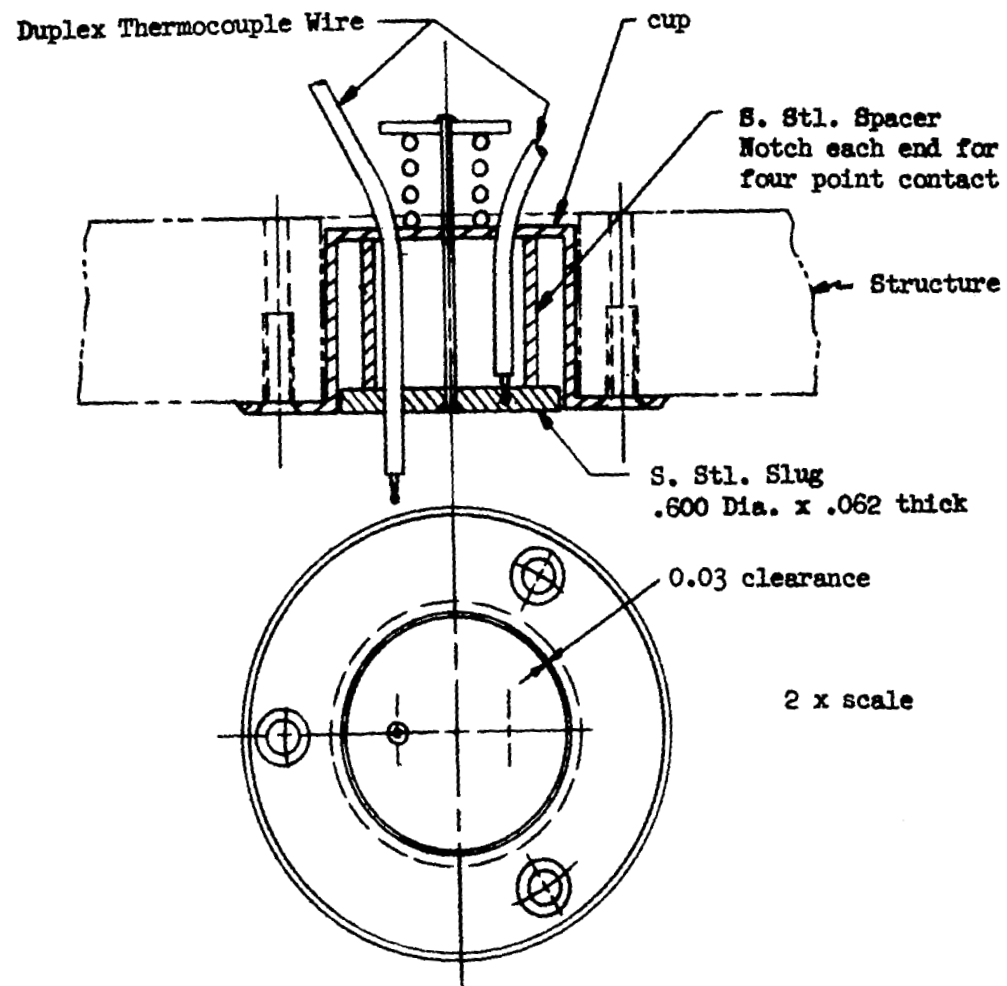
Figure 10. - Calorimeter Design.
