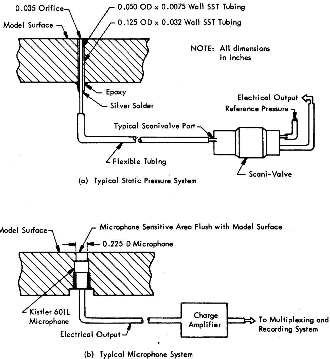
Figure 14. Details of Static Pressure and Microphone Systems
