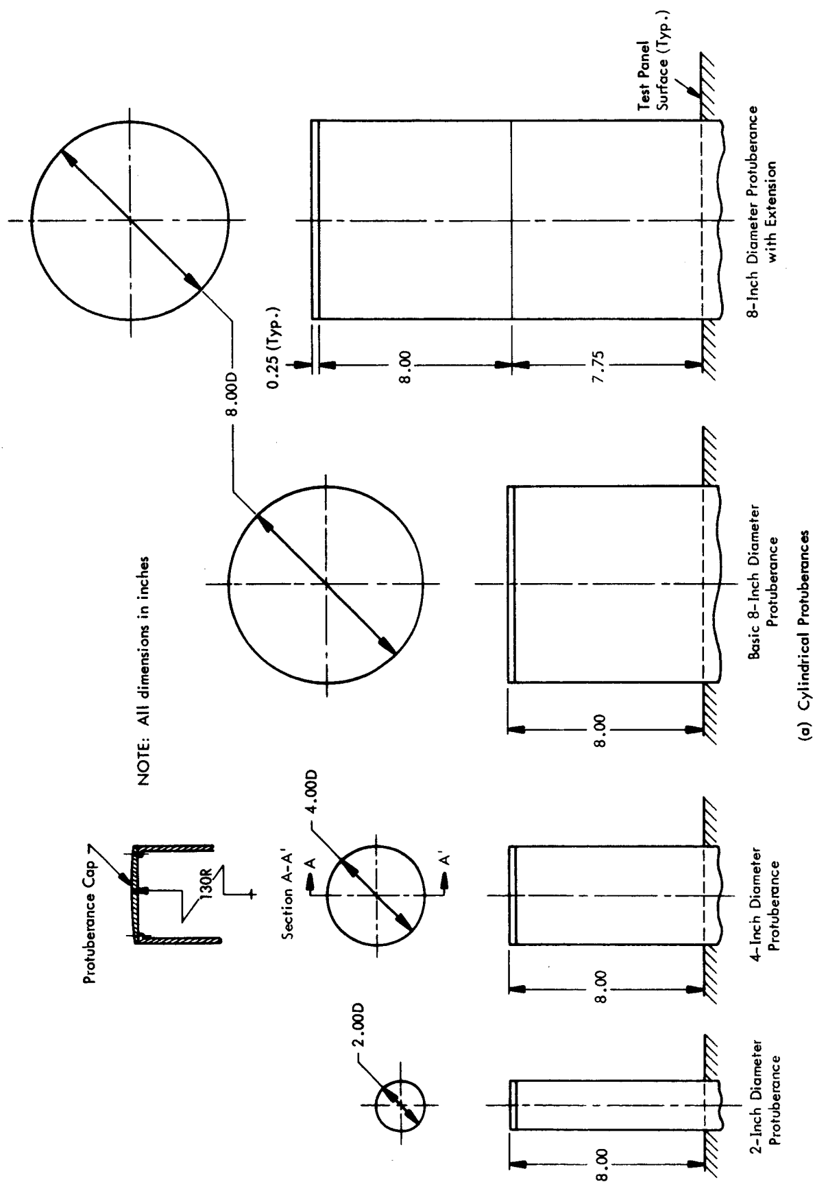
Figure 7. Details of the Cylindrical Protuberances
