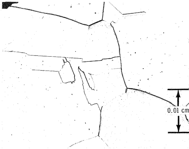
(b) Nickel 270. Etchant, 92 percent HCl, 5 percent H 2 SO 4 , and 3 percent HNO 3 ; two grain sizes, approximately 60 percent grain size 0 (1/2 grain/in. 2 at X100), approximately 40 percent grain size 2 (2 grains/in. 2 at X100).
