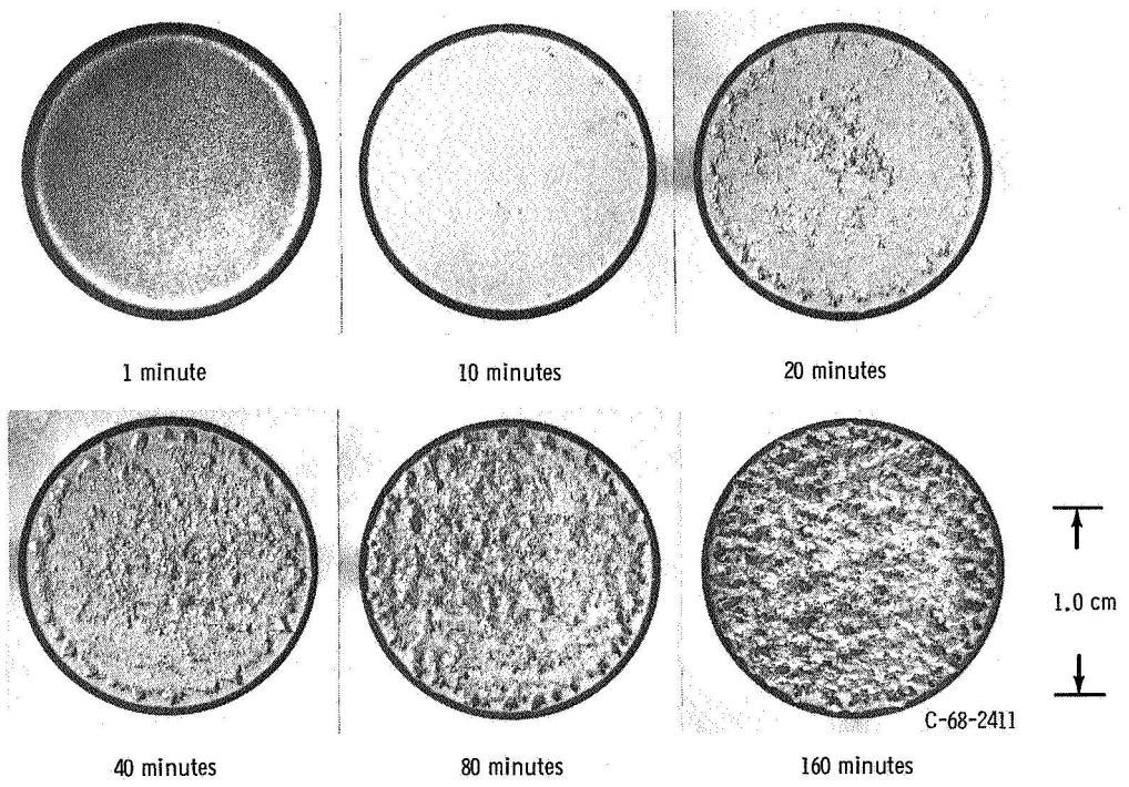
(c) 6061-T6 aluminum. Figure 9. - Concluded
