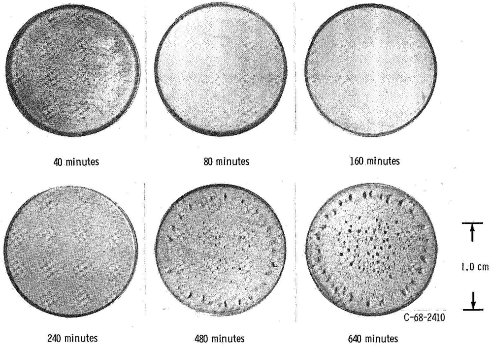
(a) AISI type 316 stainless steel.
