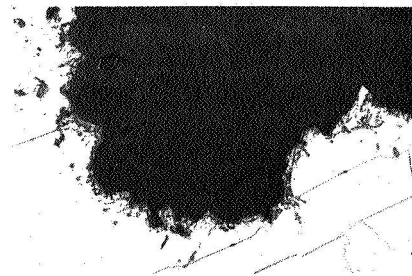
Figure 10. - Cavitation damage in duplicate test specimens of each material as viewed under oblique lighting. X2.
