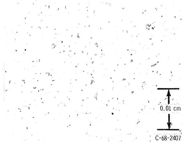
(c) 6061-T6 aluminum. Etchant, 30 milliliters glycerine, 20 milliliters HNO 3 , and 10 milliliters HF. No grain boundaries visible.
