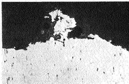
Figure 11. - Photomicrographs of sectioned specimens after exposure to cavitation in water at 75° F (23.9° C). X250.
