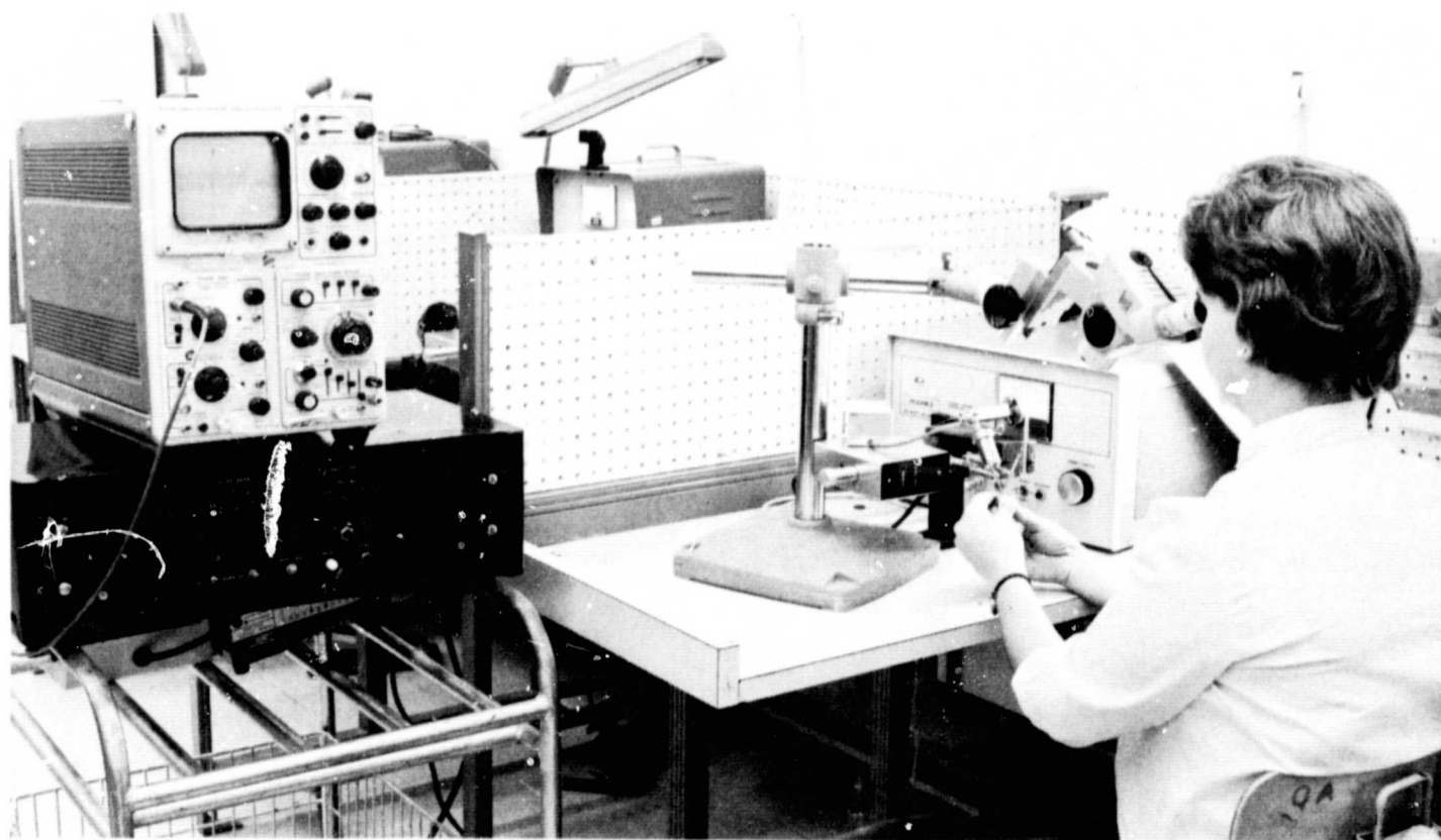
Figure 10. System Operation of Breadboard in Microweld Area
