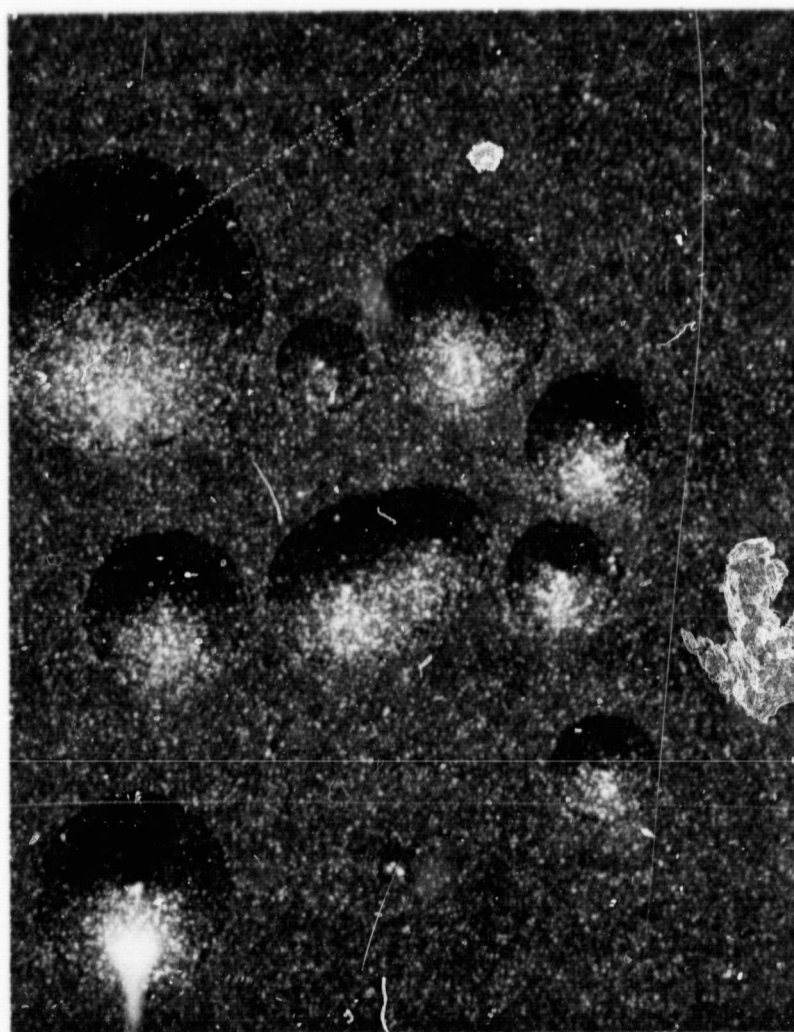
DEPOSITION SEQUENCE: \text{CdS} + \text{Cu} + \text{Cd Cl}_2 MAGNIFICATION 430 X
