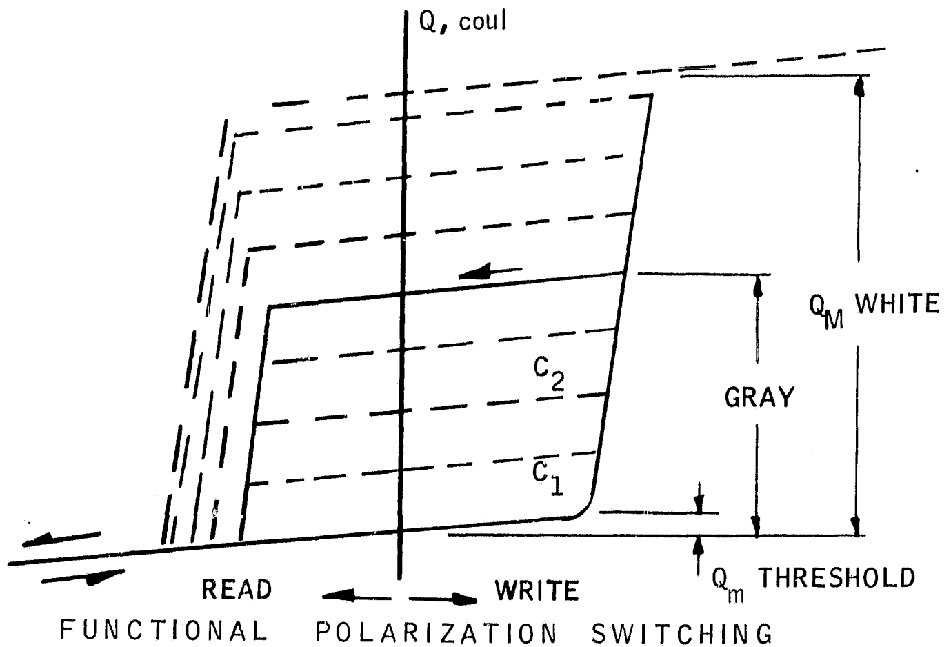
Figure 9 HYSTERESIS LOOPS
