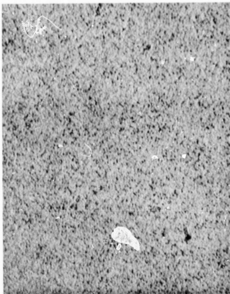
DEPOSITION SEQUENCE: \text{CdS} + \text{Cu} + \text{Cd Cl}_2 MAGNIFICATION 940 X
