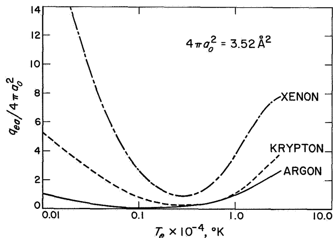
Fig. 3. Averaged momentum transfer cross sections
