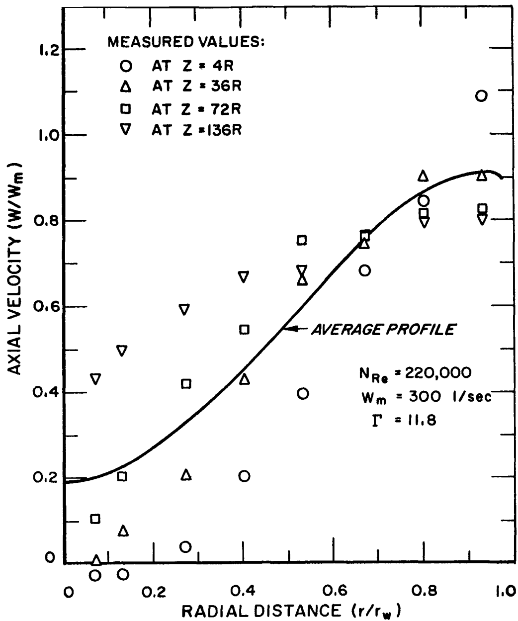
FIGURE 15. AVERAGE RADIAL DISTRIBUTION OF AXIAL VELOCITY.
