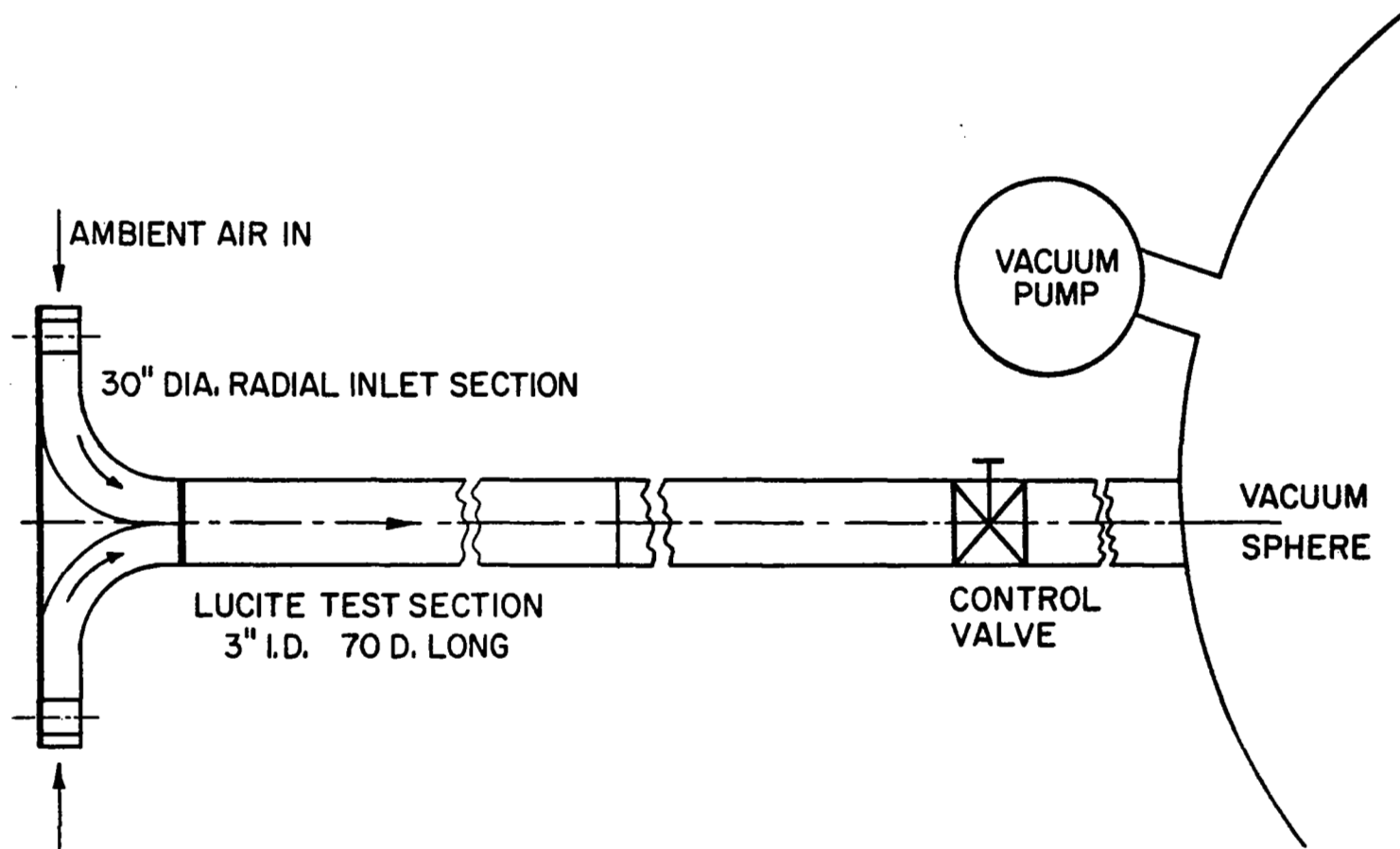
FIGURE 12. SCHEMATIC DIAGRAM OF IITRI's SWIRLING FLOW EXPERIMENTAL SET-UP.
