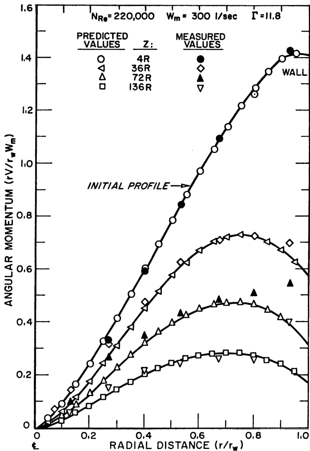
FIGURE 19. COMPARISON OF MEASURED AND PREDICTED RADIAL DISTRIBUTIONS OF ANGULAR MOMENTUM.
