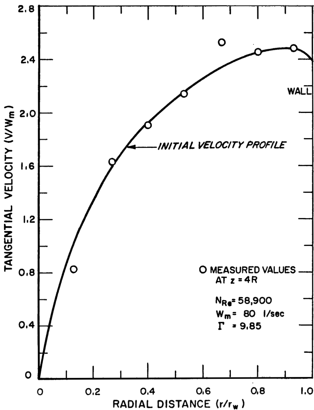
FIGURE 14. MEASURED TANGENTIAL VELOCITY PROFILE.
