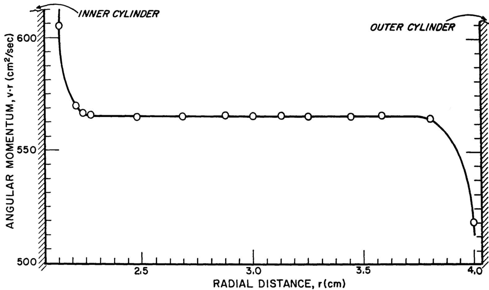
FIGURE 4. DISTRIBUTION OF ANGULAR MOMENTUM IN THE ANNULAR SPACE BETWEEN TWO CONCENTRIC CYLINDERS (INNER CYLINDER ROTATING) AFTER G. I. TAYLOR (7) .
