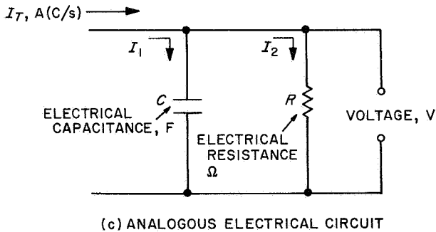
Fig. 5. HBW squib: thermal and analogous electrical circuits
