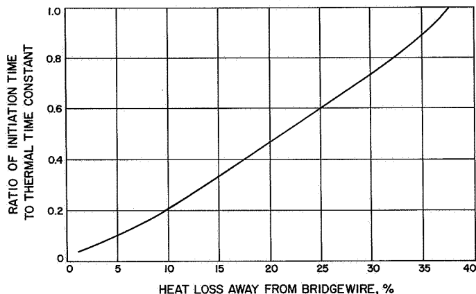
Fig. 7. Heat loss vs ratio of initiation time to thermal time-constant
