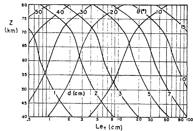
Fig. 7. Cross plots of data from Tables VI and VII, relating limiting values of shield diameter d , altitude z , view half-angle \theta , and thermal entry length Le_T for safety factors \alpha .
