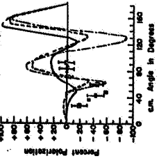
POLARIZATION ANGULAR DISTRIBUTION FOR THE C^{12}(n,p)C^{12} REACTION FOR 14.7 MeV INCIDENT NEUTRONS
