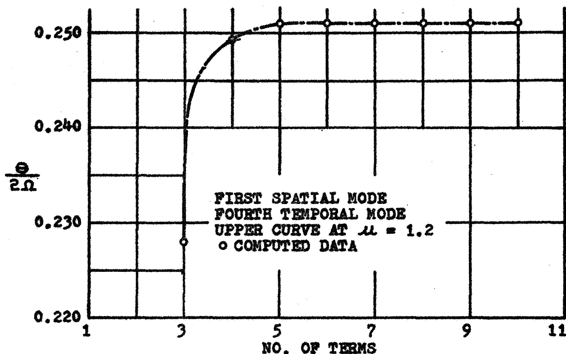
Fig. 10 Convergence Curve Associated with Mathieu's Equation Fourth Temporal Mode Upper Curve
