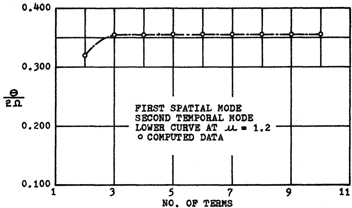
Fig. 7 Convergence Curve Associated with Mathieu's Equations Second Temporal Mode Lower Curve
