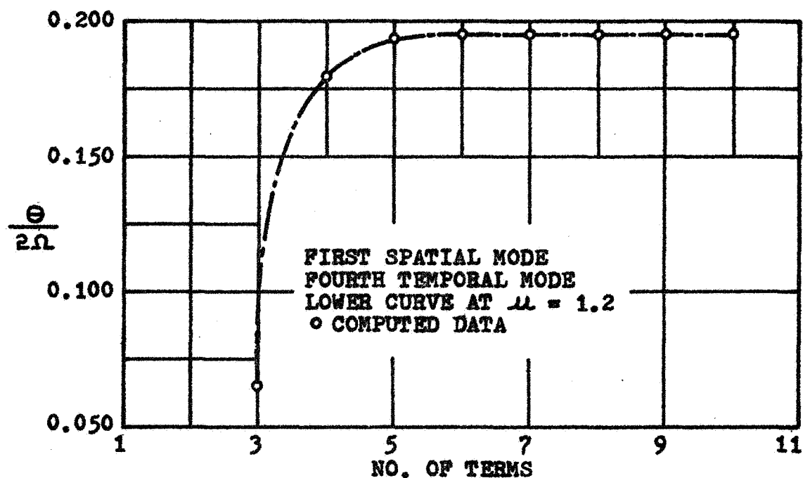
Fig. 11 Convergence Curve Associated with Mathieu's Equation Fourth Temporal Mode Lower Curve
