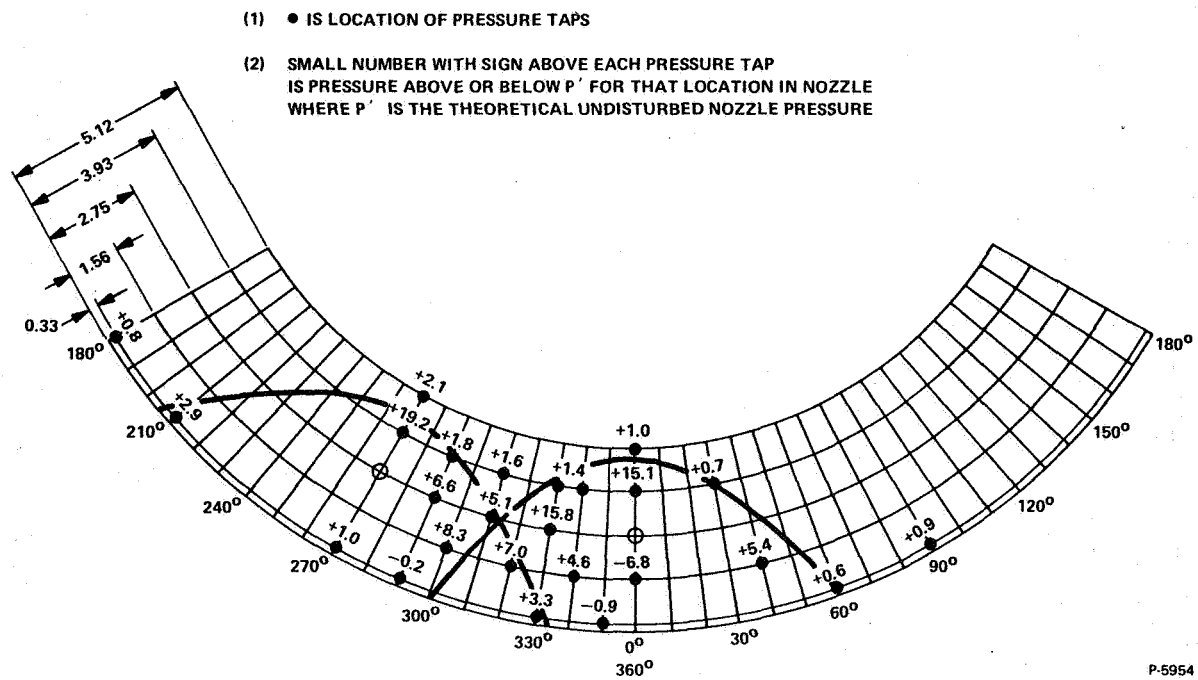
Figure 38(f) - Nozzle Pressure Probe Map - Time 4.318
