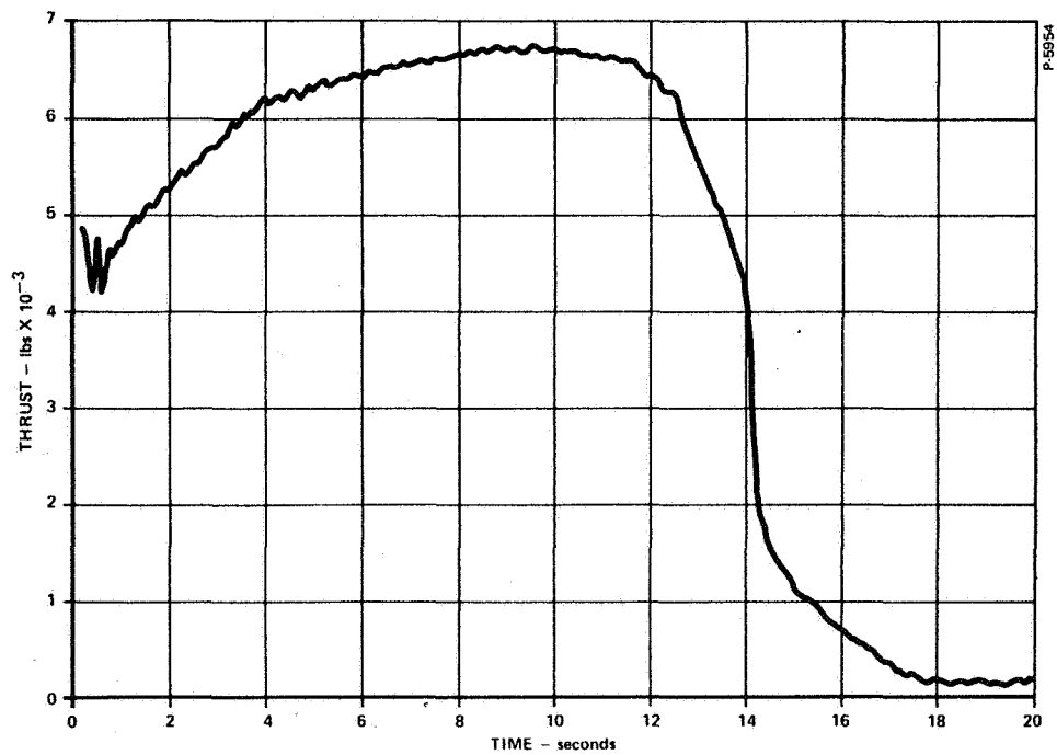
Figure 20 - EM-72 Rocket Motor Axial Thrust
