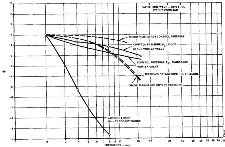
Figure 34 - Amplitude Versus Frequency, Yaw Plane of Vortex Valve Controlled SITVC System on EM-72 Rocket Engine
