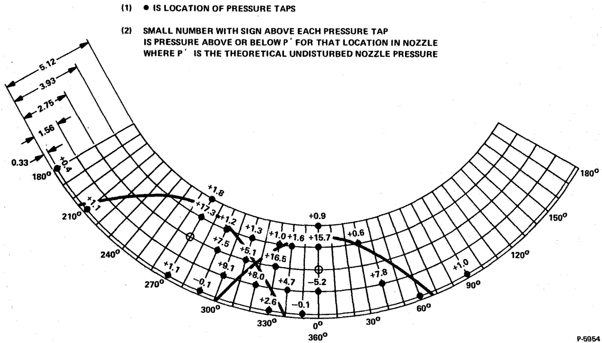
Figure 38(e) - Nozzle Pressure Probe Map - Time 4.285
