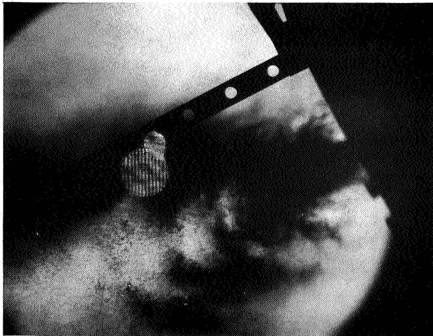
Figure 3-36. Reconstruction photograph of the edge view of the combustion spray fan recorded on \text{N}_2\text{O}_4 -50/50 \text{N}_2\text{H}_4 -UDMH firing No. B1115R
