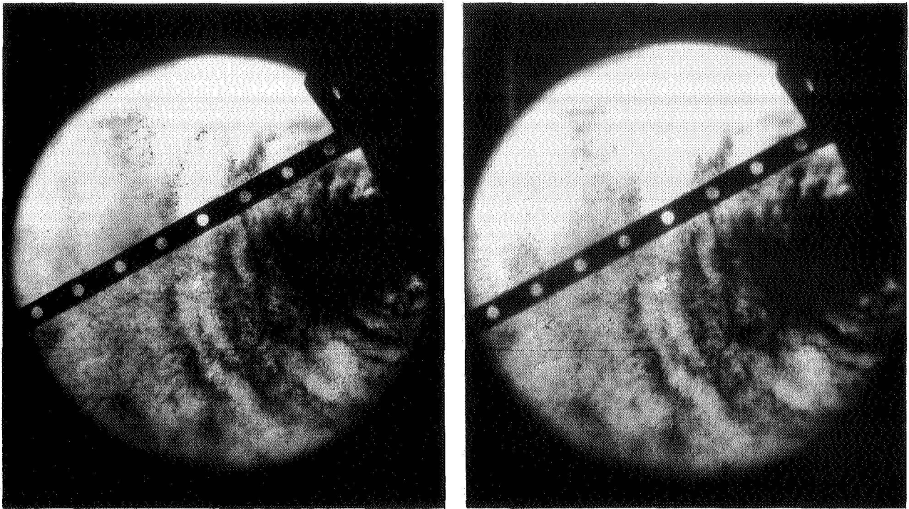
Figure 3-32. Two photographs of the reconstruction of a ruby laser hologram of the open flame combustion of \text{N}_2\text{O}_4 and 50/50 mixture \text{N}_2\text{H}_4 and UDMH (Run B1117G). The two differ by a slight change in focus of the f/8 150mm copy camera lens. In the left, the steel strap with 1/4-inch holes on 1-inch centers is in sharp focus. In the right, it is out of focus.
