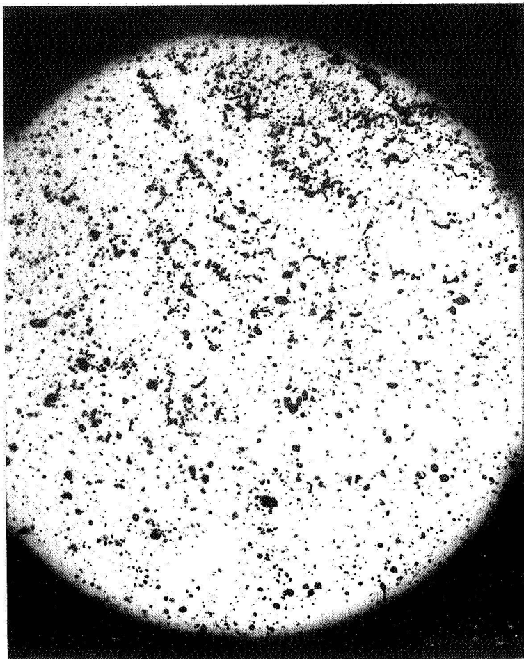
Figure 3-31. Photographic print made from a laser-illuminated photograph taken of the water flow from the JPL single element injector during test number B1113U. Direction of droplet flow is from the upper right-hand corner of the photograph to the lower left-hand portion. Examination of the Agfa 10E75 film plate (from which this print was made), under a microscope, indicated a resolution of around 25 microns.
