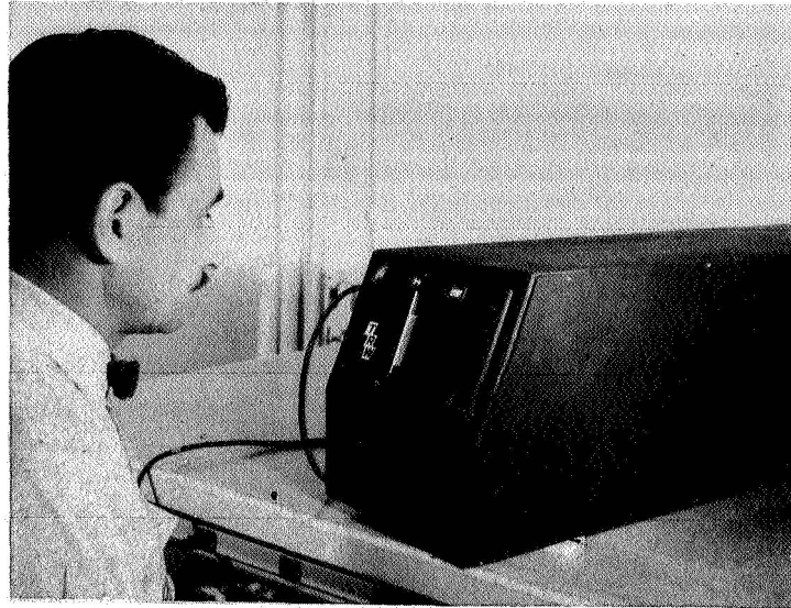
Figure 3-18. Photograph of the apparatus used to reconstruct holograms recorded in the JPL hologram camera with a 45° scene-reference beam angle
