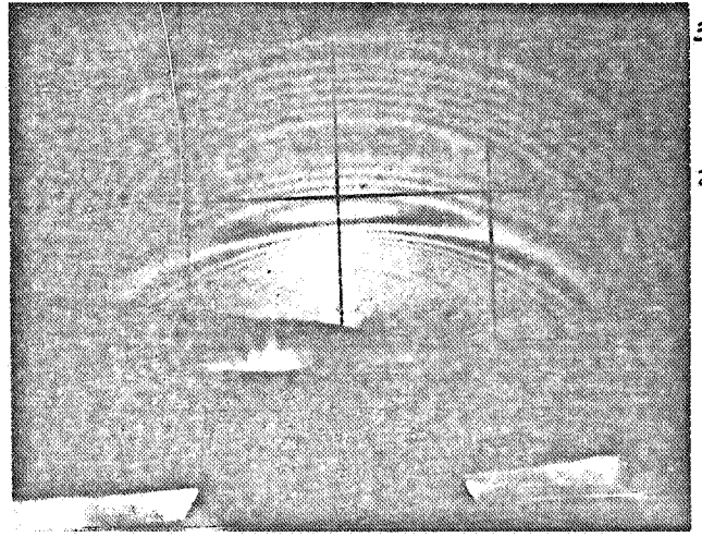
PICRIC ACID
