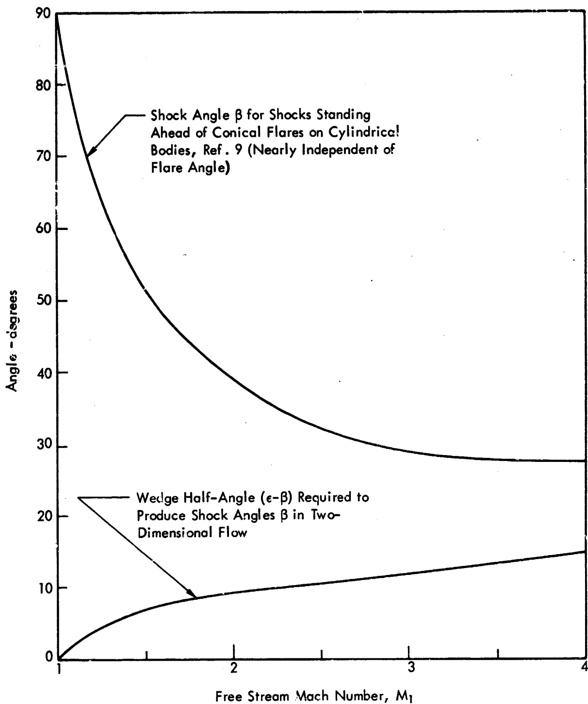
Figure 40. Interpretation for Separation Shocks Before Conical Transitions
