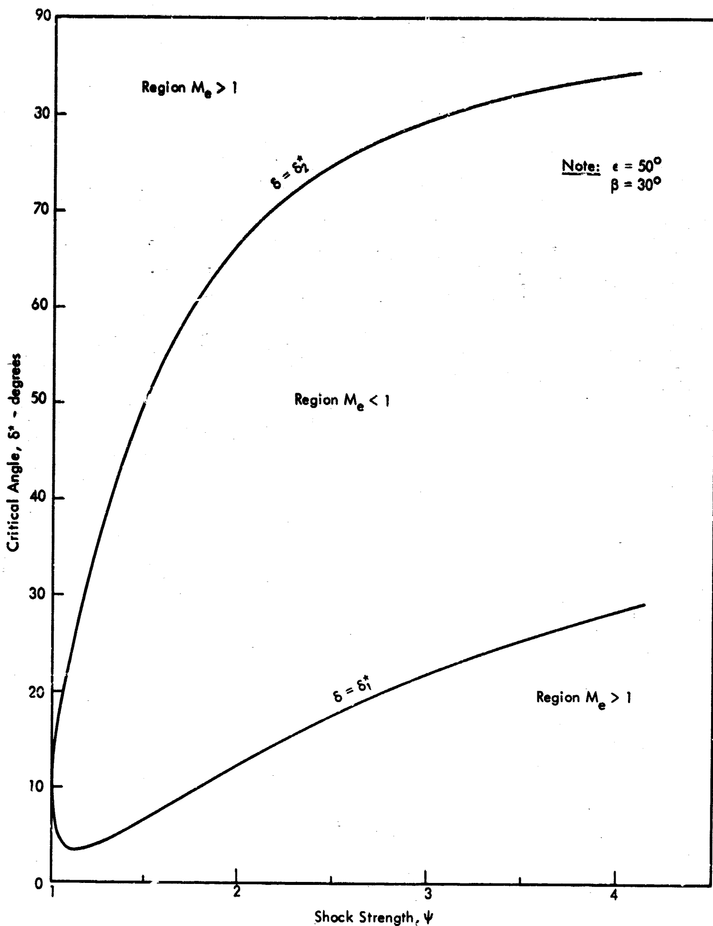
Figure 9. Typical Boundaries of Subsonic Region
