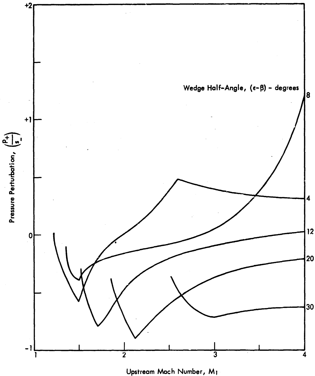
Figure 24. Generated Pressure Disturbance, Oblique Shock Case, \delta = 50^\circ
