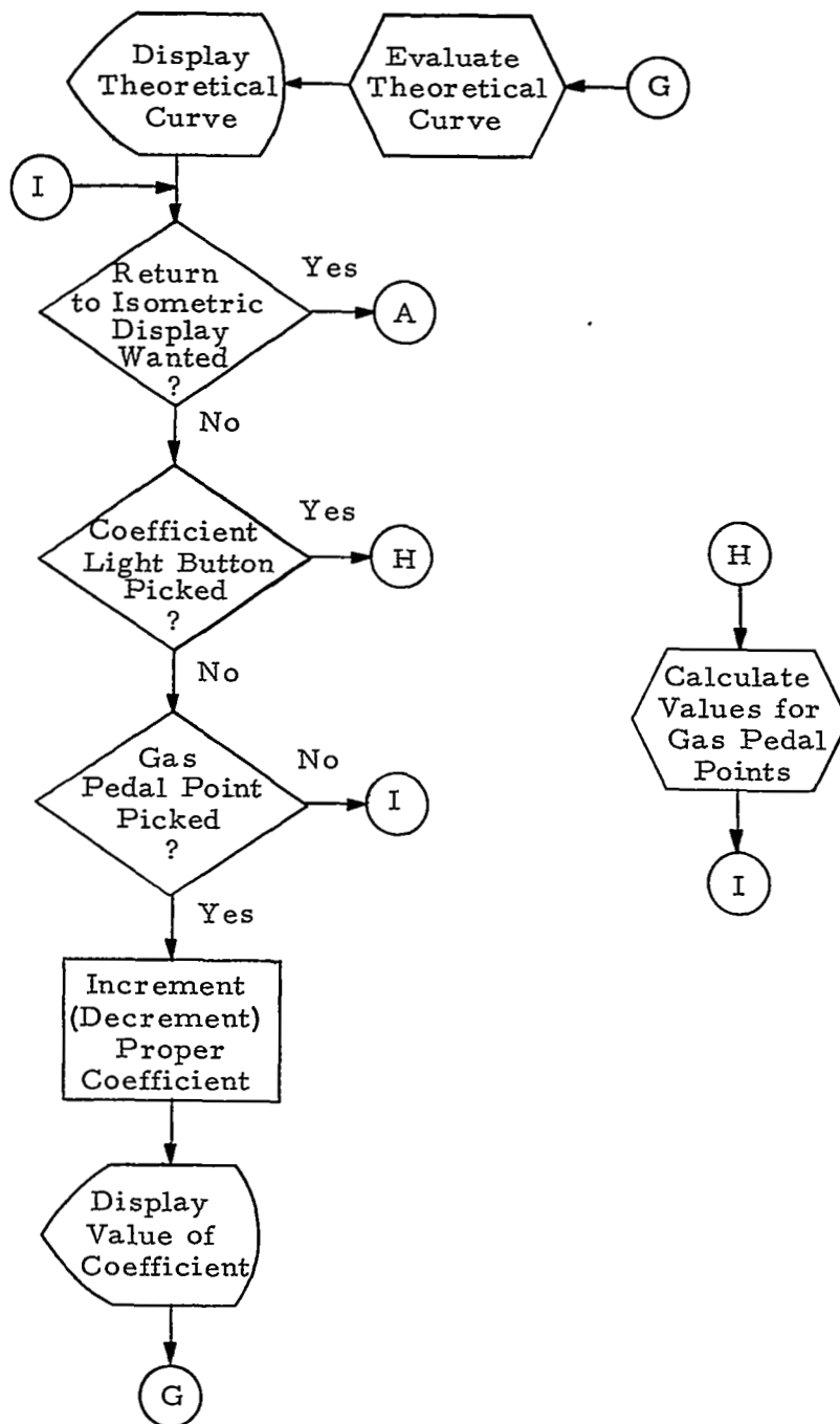
FIGURE VII. 13 ISOMETRIC PROJECTION AND CURVE FITTING FLOW CHARTS (Con't)
