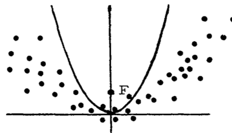
FIGURE 15 CURVE FITTING
