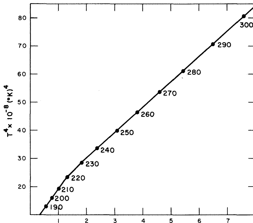
Figure 1. The abscissa is the response of the infrared radiometer, through the 8- to 13- \mu atmospheric window, as a function of the fourth power of the temperature of the planet. The response scale is arbitrary. Temperatures given on the curve are in °K.
