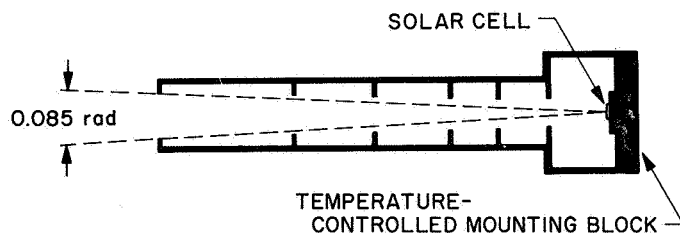
Fig. 1. Solar cell collimating tube
