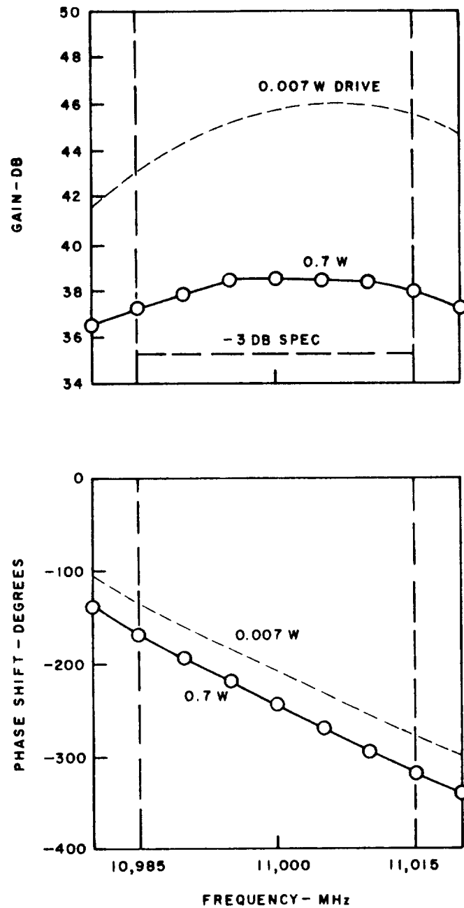
Figure 38(b) - Gain and Phase Shift Characteristics of 11,000-MHz FM Klystron
