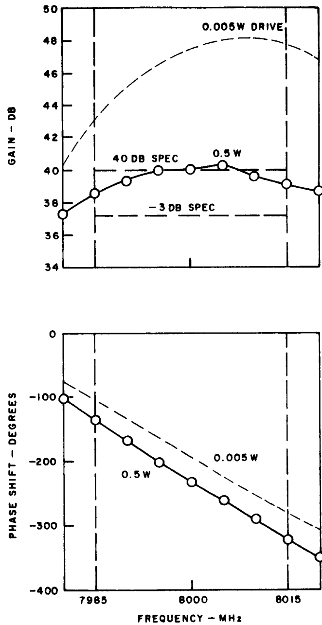
Figure 37(b) - Gain and Phase Shift Characteristics of 8000-MHz FM Klystron
