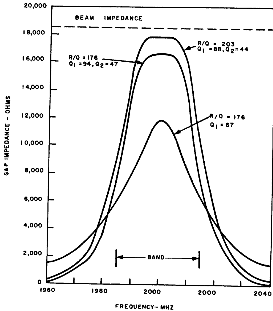
Figure 21 - Impedance of Singly-Tuned and Doubly-Tuned Output Cavities for 2000-MHz FM Klystrons
