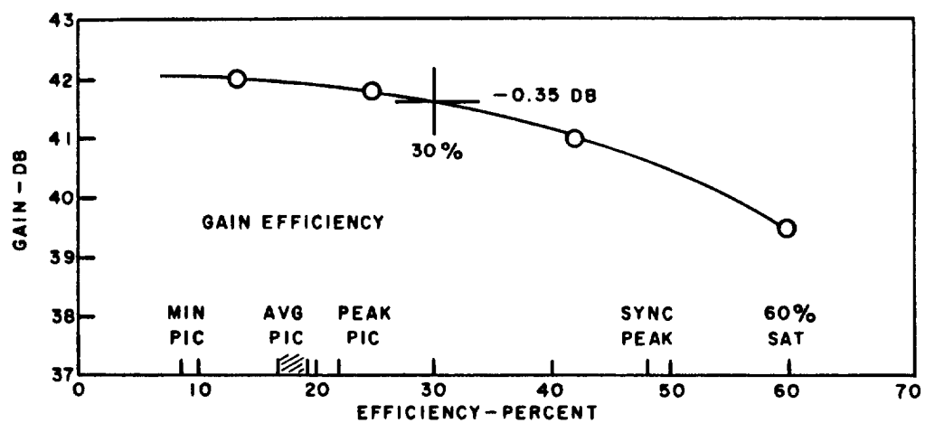
Figure 31 - Large-Signal Characteristics of 850-MHz AM Klystron at Various Signal Levels at Midband
