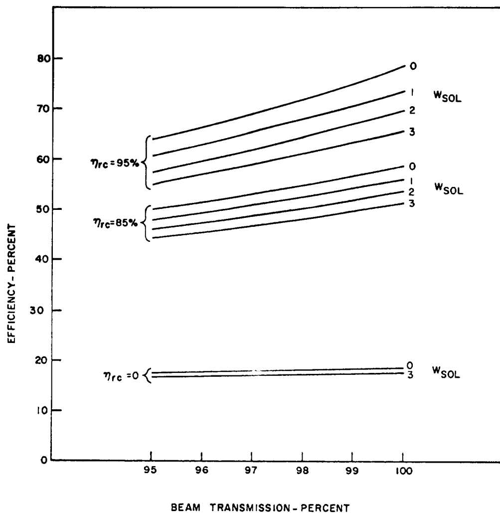
Figure 77 - Efficiency Trade-Offs in 850-MHz AM Klystron (Overall output efficiency versus beam transmission for three values of reflex-collector energy recovery efficiency, \eta_{rc} , and four values of normalized solenoid power, W_{sol} )
