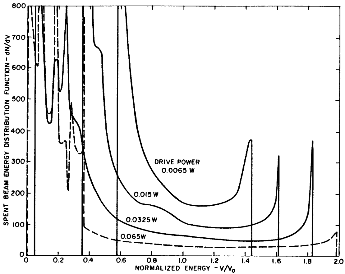
Figure 35 - Spent-Beam Spectrum of 2000-MHz AM Klystron as Function of Drive Level
