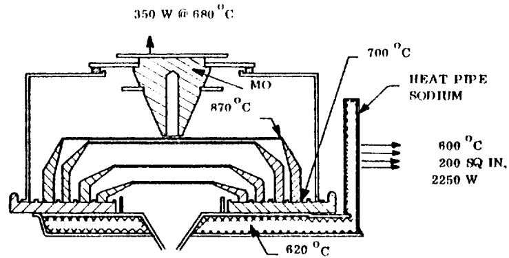
Figure 54 - Heat Pipe Cooling System for Multi-Potential Reflex Collector
