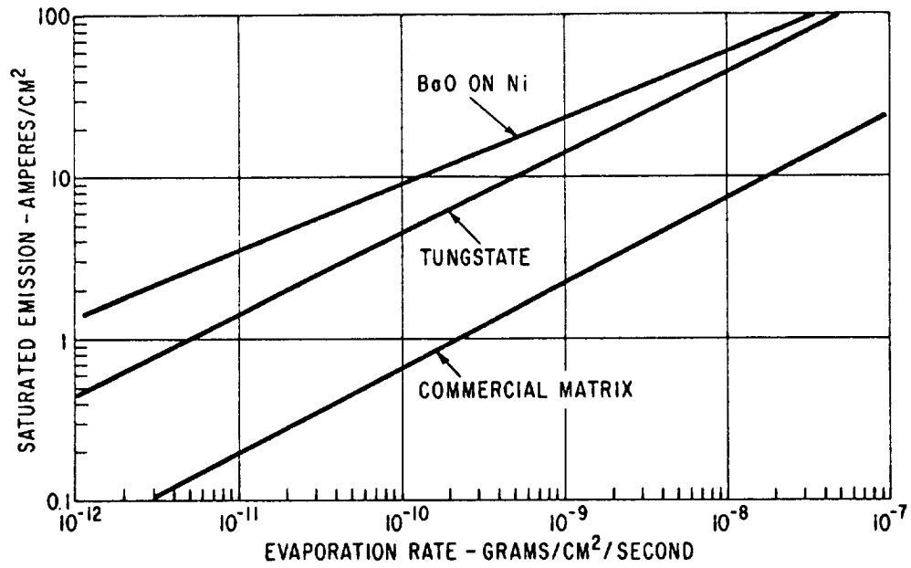
Figure 41*- Saturation Emission Capability of Three Cathodes as Function of Evaporation Rate
