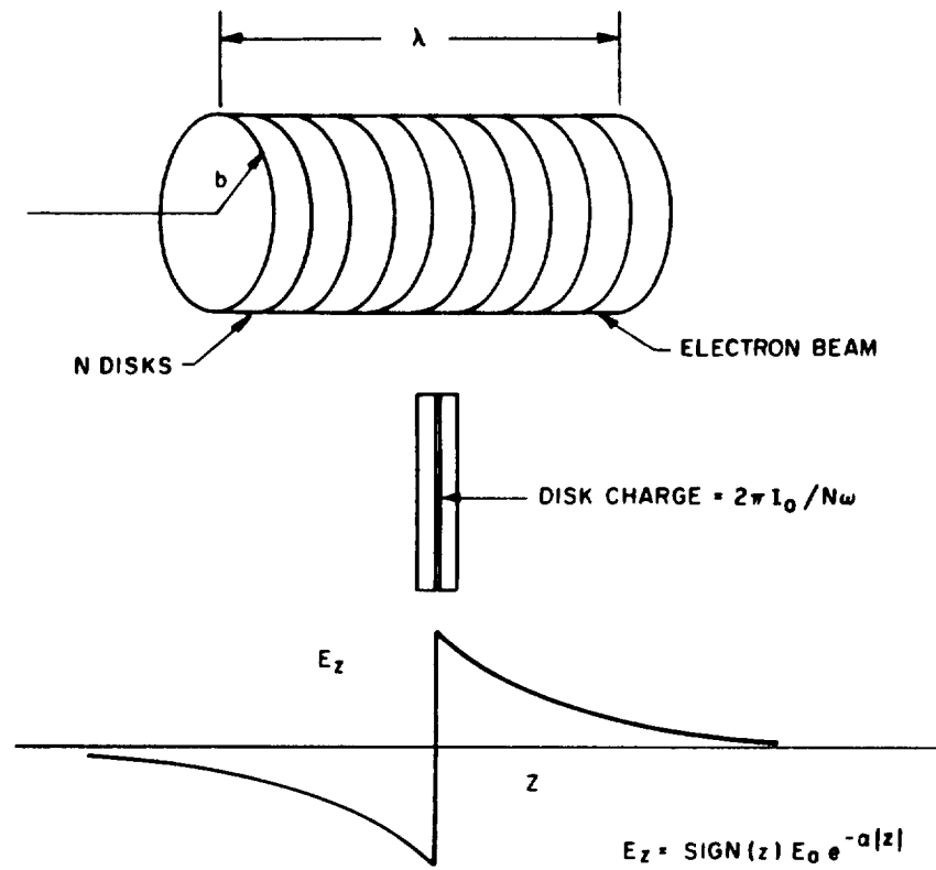
Figure 2 - Disk Model of Electron Beam (Division of One Wavelength into N Disks and Sketch of Axial Field Variation of Single Disk.)
