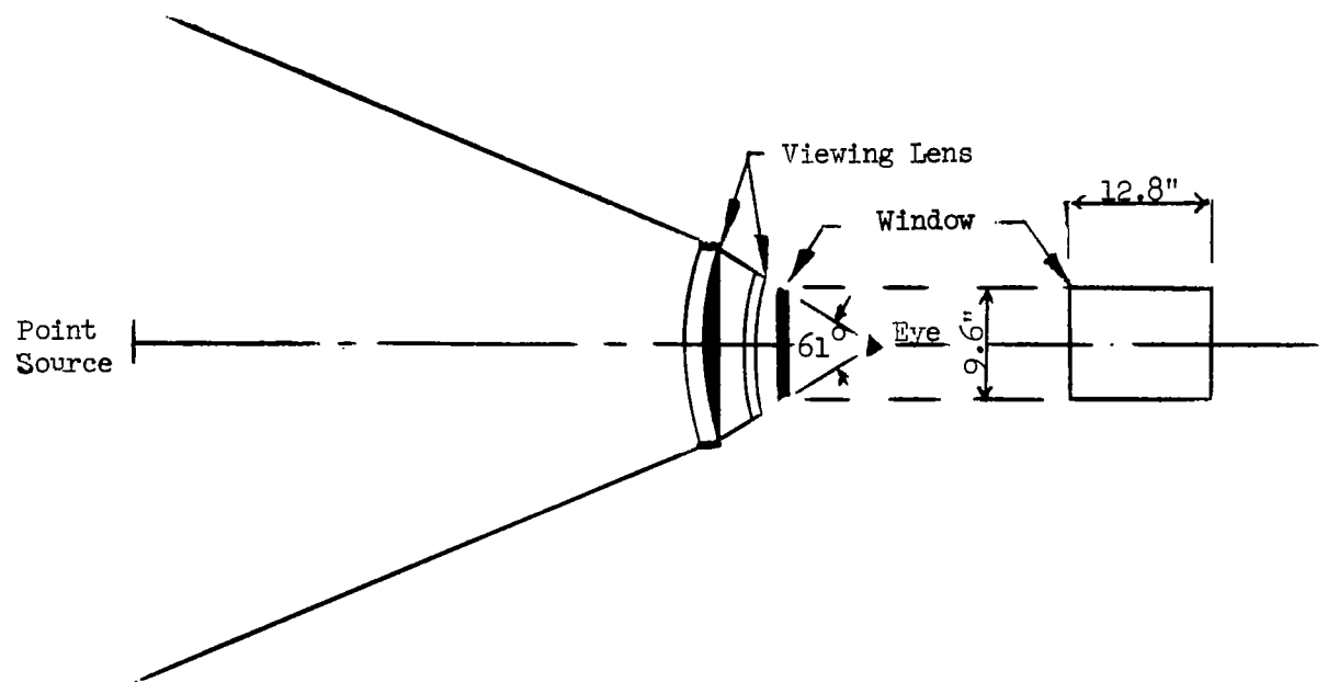
Fig. 2 Lens Schematic
