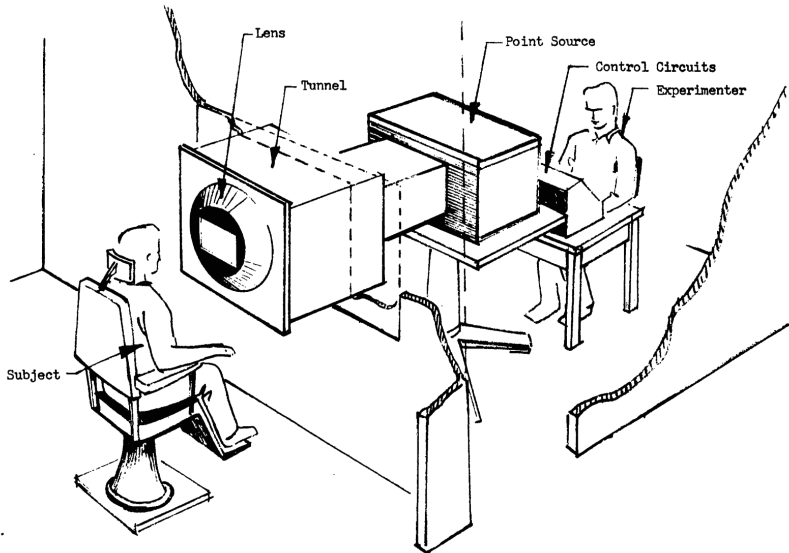
Fig. 1. Experimental Facility
