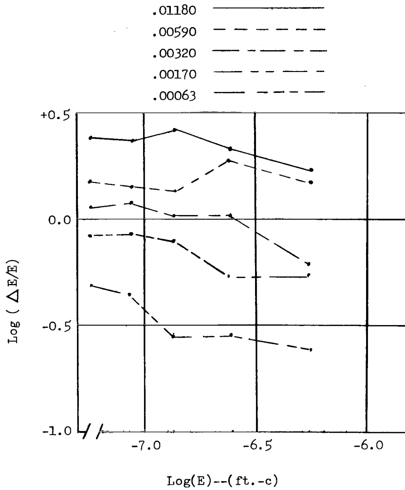
Fig. 6 Log ( \Delta E/E ) as a Function of Log (E) for all Wedge Rates
