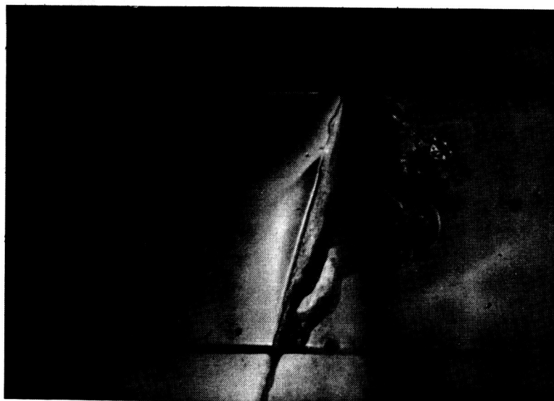
Figure 10. Dydrazine/Nitrogen Tetroxide Impingement at 25°C 50 ft/sec and .100 inch Wide Stream. Regime II-Separation
