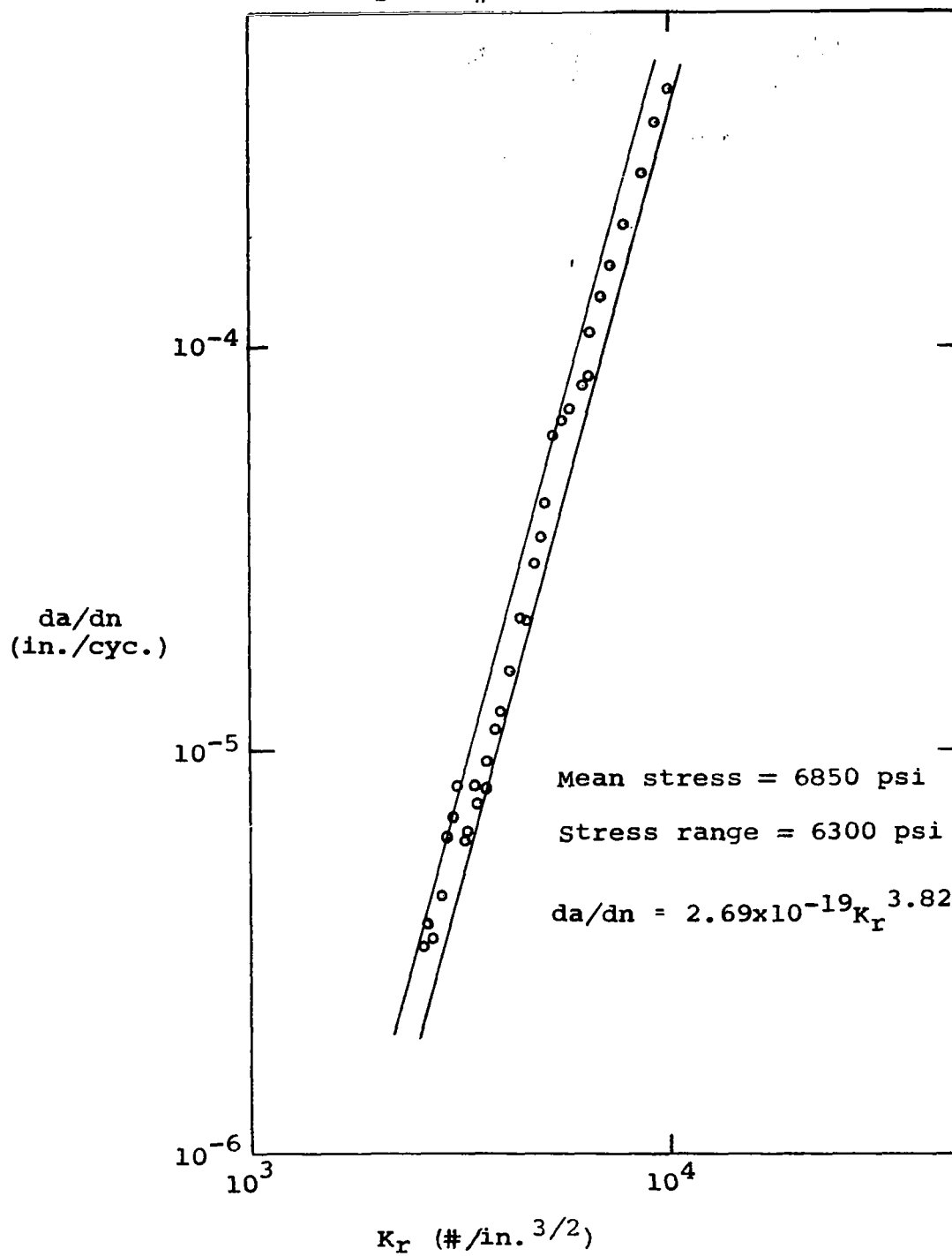
FIGURE 11 da/dn vs. K_r
