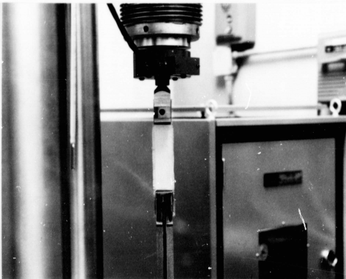
Fig. 4 Specimen in machine before test
