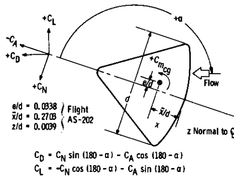
Fig. 6 Apollo Spacecraft 011 - Orientation of Forces and Moments
