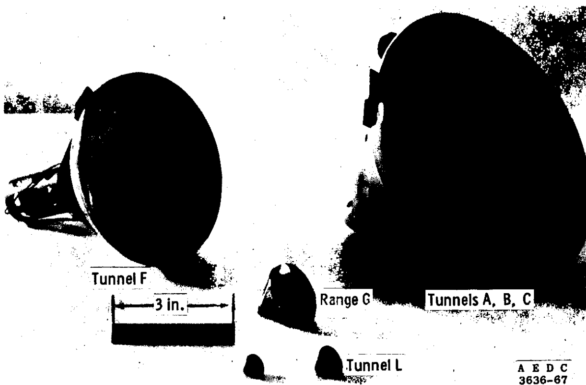
Fig. 2 Photograph of AEDC-VKF Apollo Models
