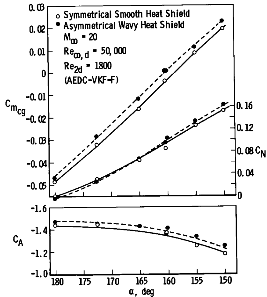
b. Multi-Component Balance Data, M_\infty = 20
