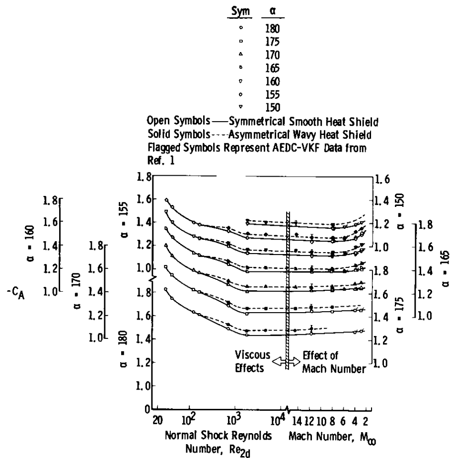
Fig. 14 Variation of Axial-Force Coefficient ( C_A ) with M_\infty and Re_{2d} , Apollo
