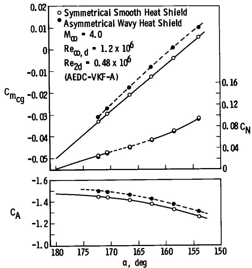
a. Multi-Component Balance Data, M_\infty = 4
