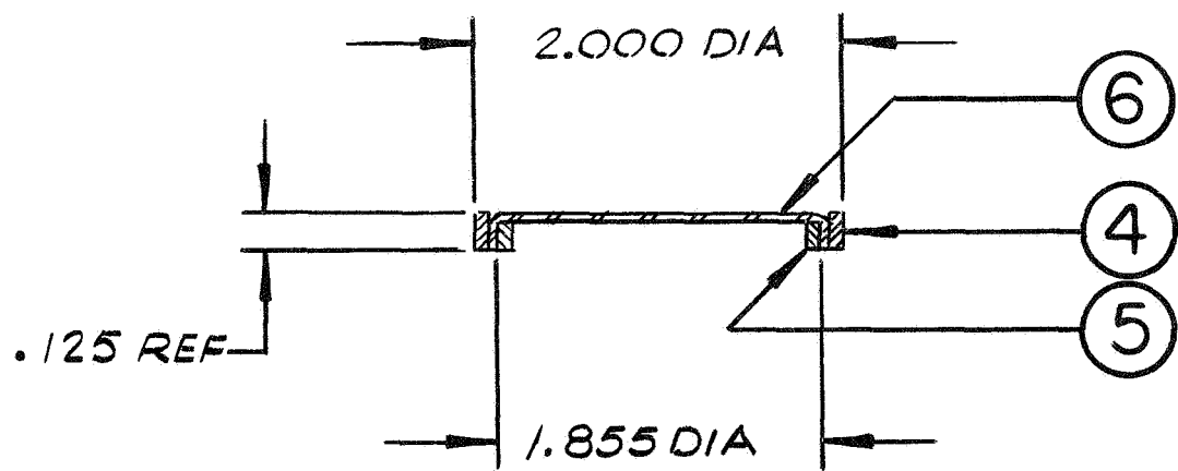
SCREEN ASSEMBLY
