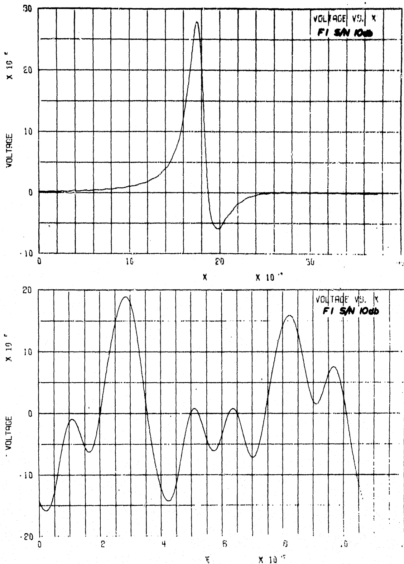
Fig. 14 Single Pulse and Multi-cycle Waveform - Filter #1, S/N = 10 db
