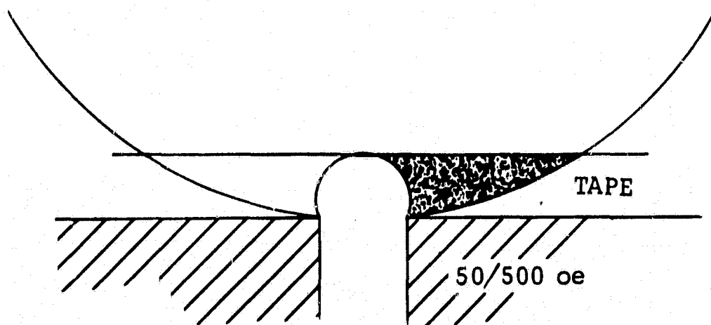
Fig. 4 Record Zones for Different Switching Fields
