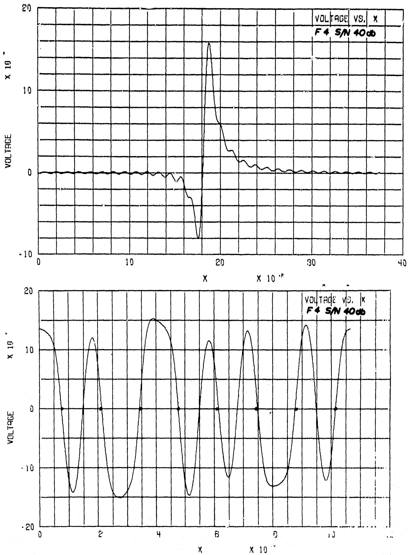
Fig. 29 Single Pulse and Multibit Waveform - Filter #4, S/N = 40 db
