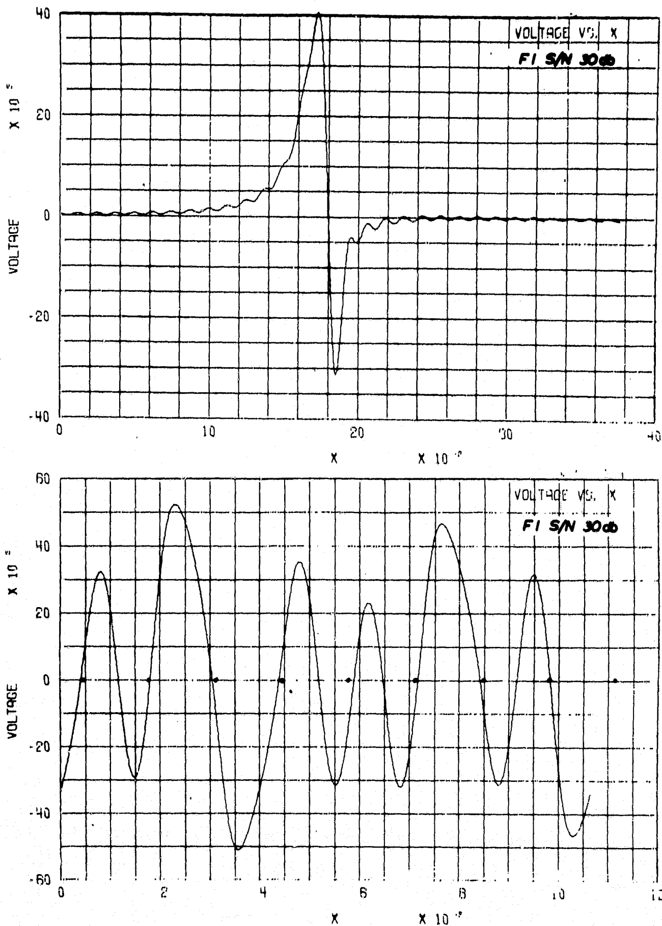
Fig. 16 Single Pulse and Multibit Waveform - Filter #1, S/N = 30 db
