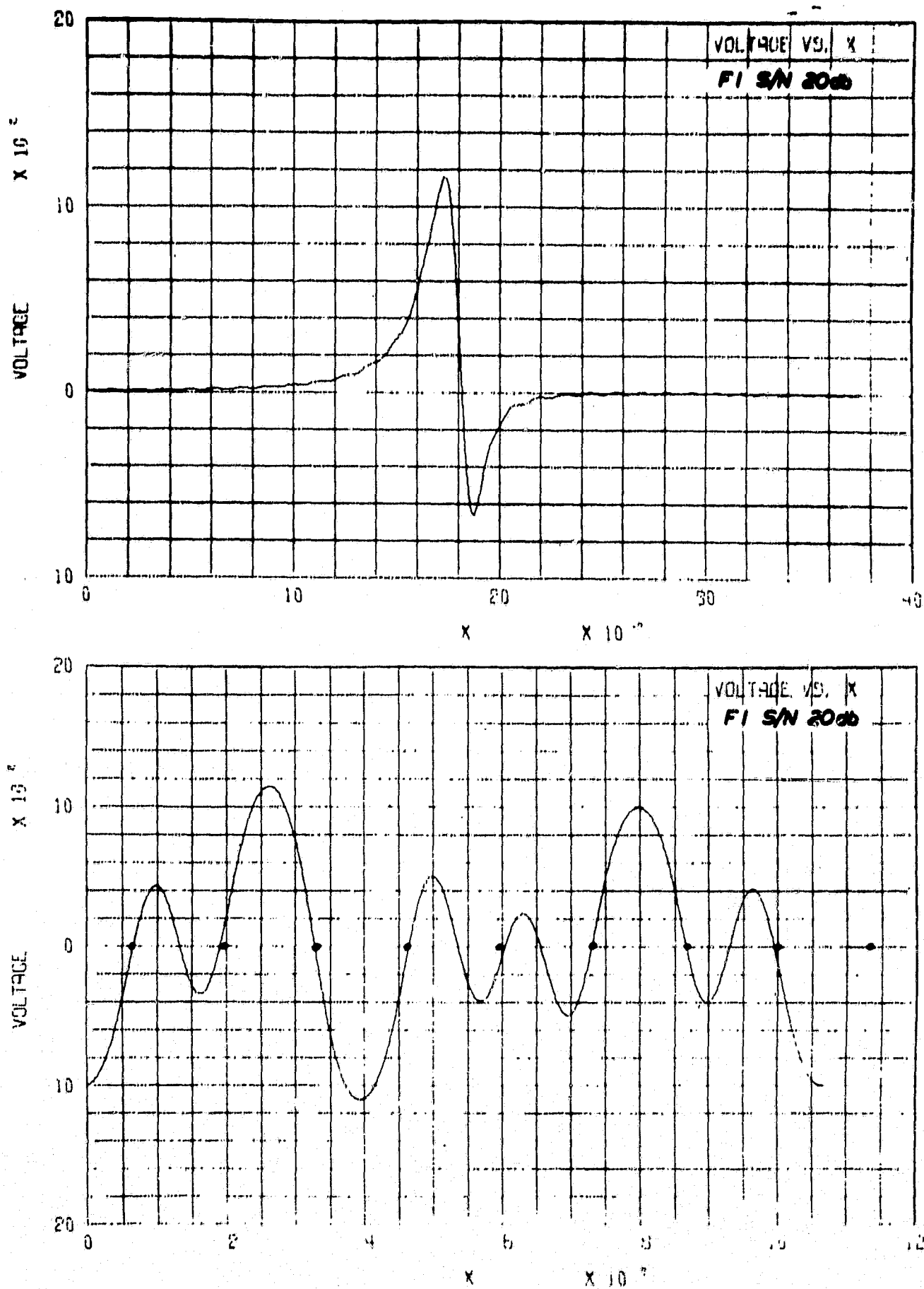
Fig. 15 Single Pulse and Multibit Waveform - Filter #1, S/N = 20 db
