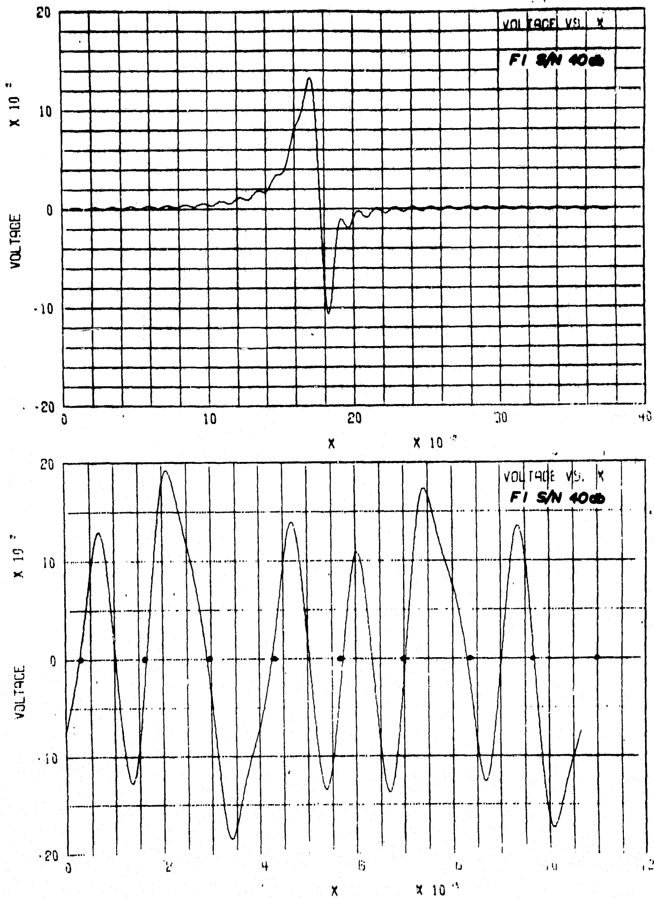
Fig. 17 Single Pulse and Multibit Waveform - Filter #1, S/N = 40 db
