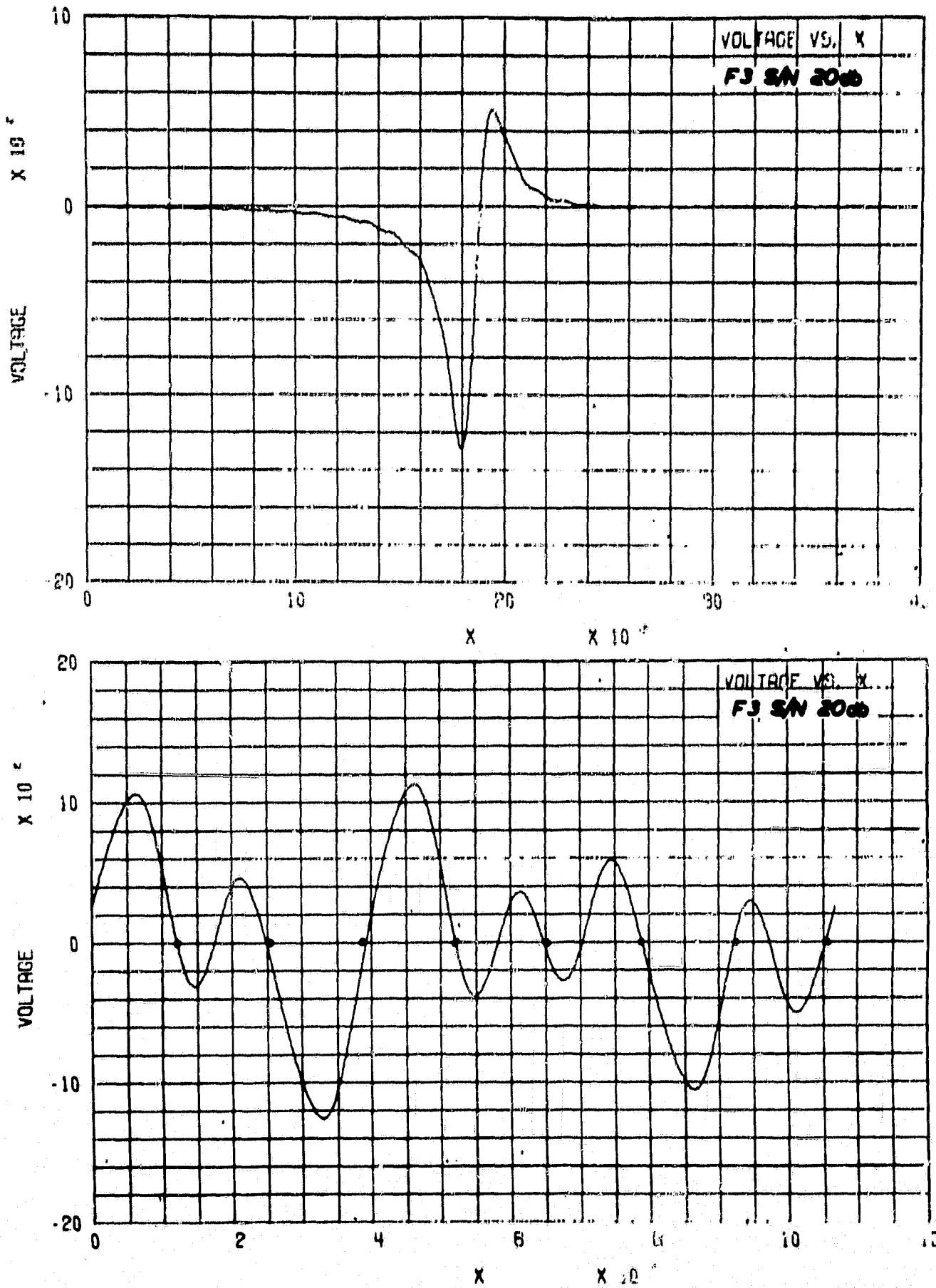
Fig. 23 Single Pulse and Multibit Waveform - Filter #3, S/N = 20 db
