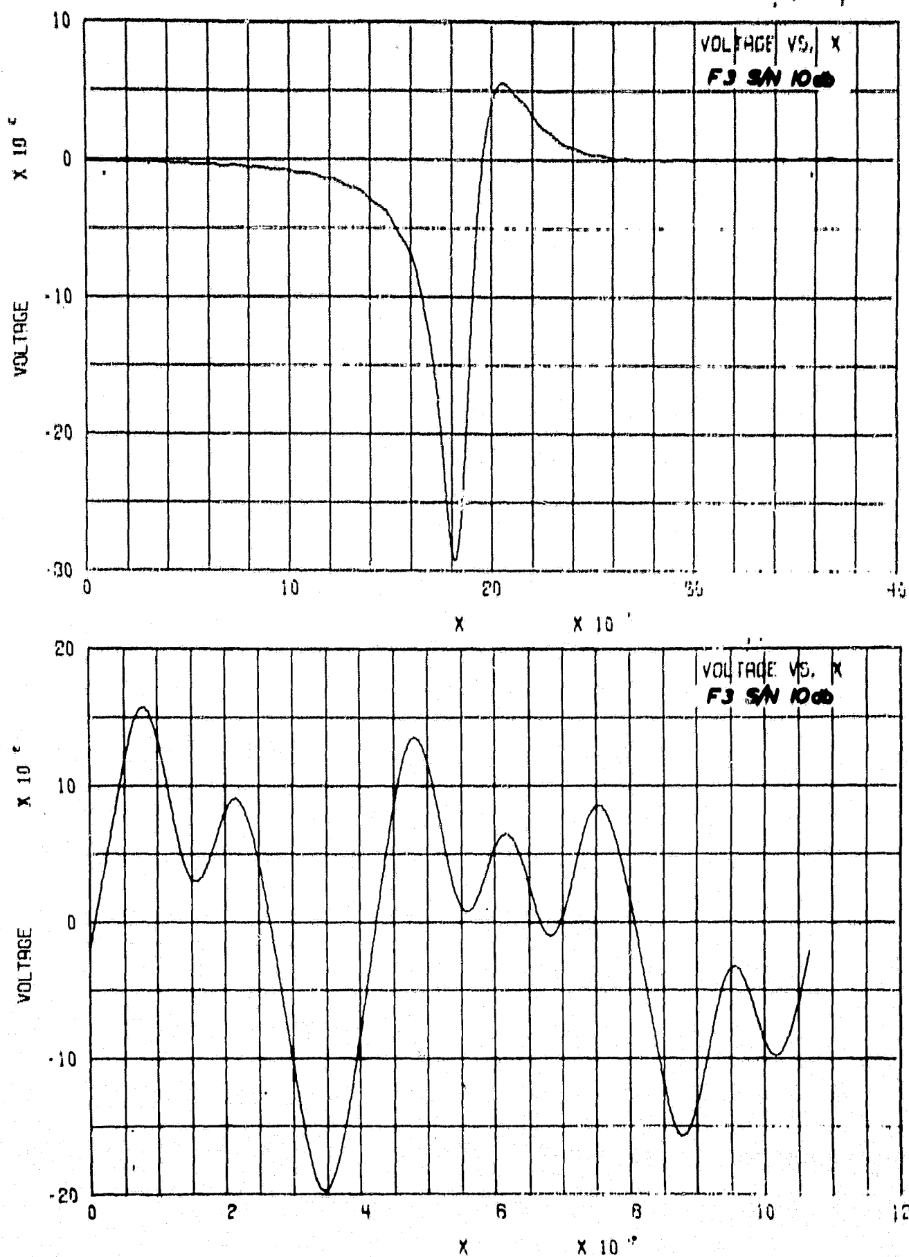
Fig. 22 Single Pulse and Multibit Waveform - Filter #3, S/N = 10 db
