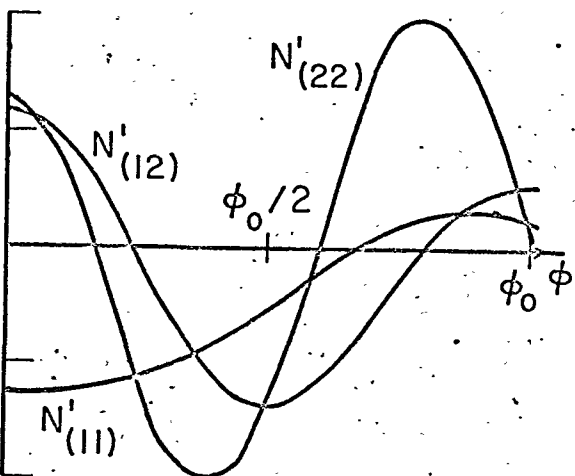
2nd Mode: \omega = 72.541977
