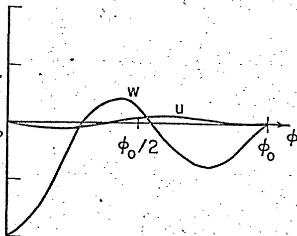
3rd Mode: \omega = 76.69792
