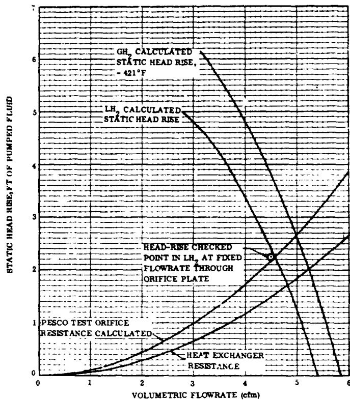
Figure 5-49. Pesco Pump Performance Curves
