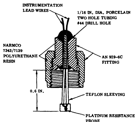
Figure 5-3. Temperature Probe Vacuum Pass-Through
