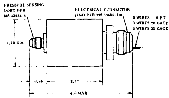
Figure 3-3. Pressure Switch Envelope
