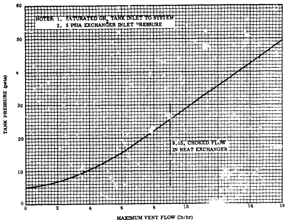
Figure 4-1. System Flow Limitation With \text{GH}_2 Inlet
