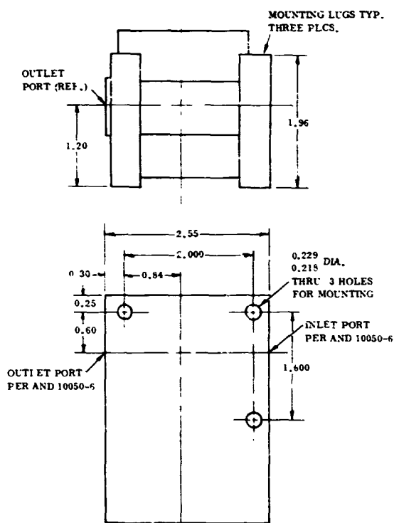
Figure 3-1. Regulator Envelope
