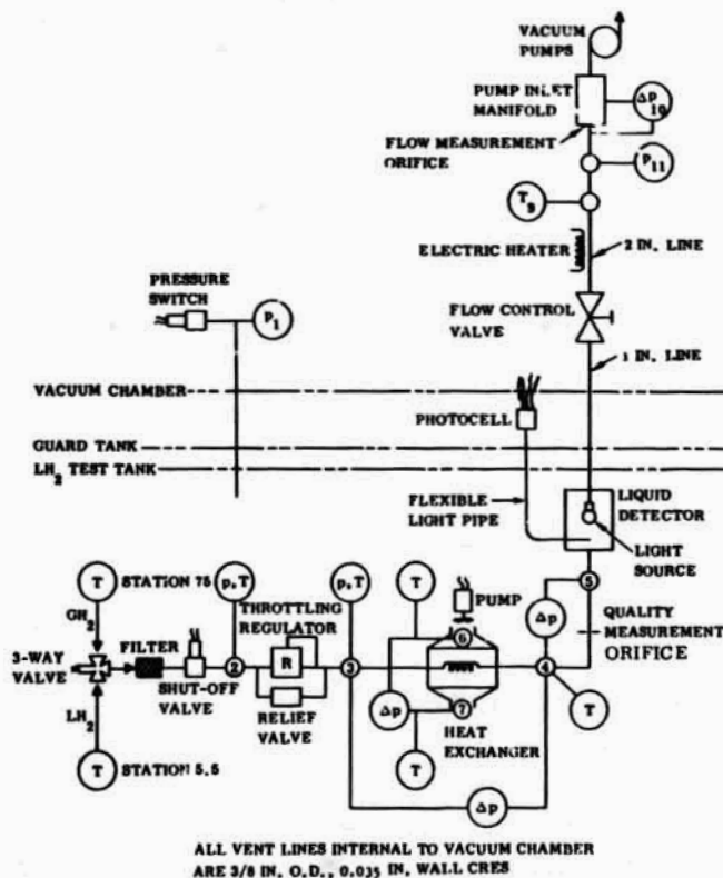
Figure 5-1. Basic Vent System Test Schematic
