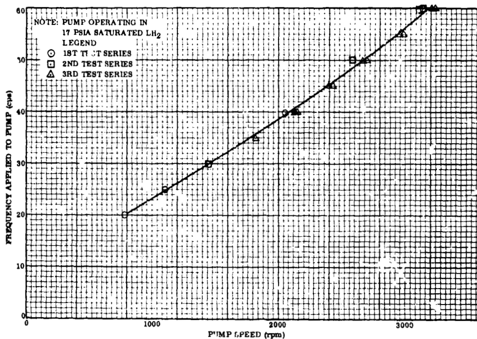
Figure 5-47. Pump Speed Versus Applied Frequency
