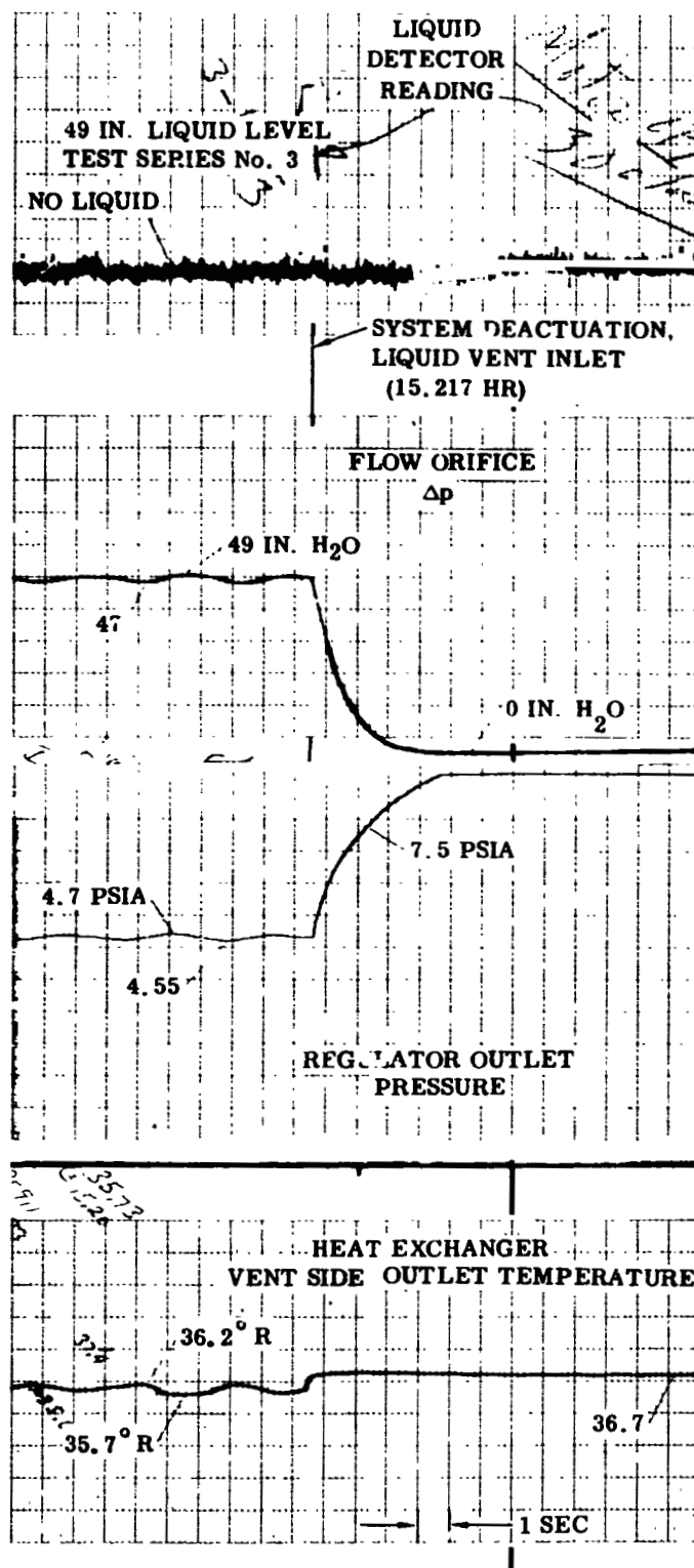
Figure 5-36. System Deactuation - Shutoff Downstream
