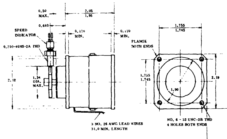
Figure 3-4. Pump Envelope
