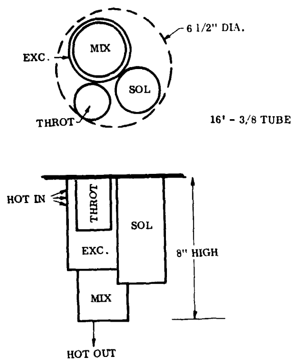
Figure 2-17. Typical Exchanger System Package (Coiled Tube)
