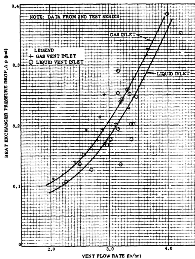
Figure 5-45. Heat Exchanger Pressure Drop Versus Flow Rate
