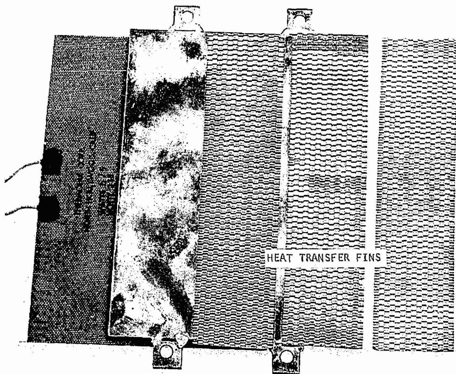
Figure 2-6. Wick Performance Test Module Assembly
