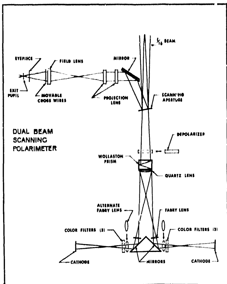
FIG. 1. Optical system of scanning polarimeter. As shown in this diagram, the direction of the aperture scan is perpendicular to the plane of the paper.
