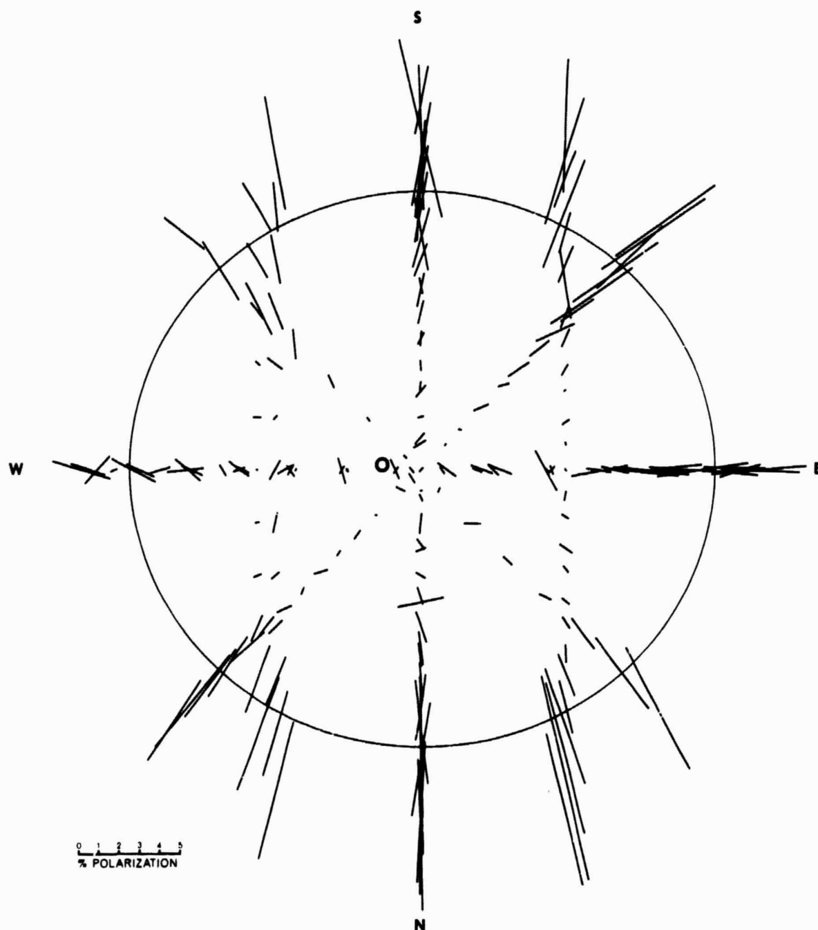
Figure 8. Observations similar to those described in Figure 4 but made on seven nights with the 72-inch and on three nights with the 30-inch reflector.
