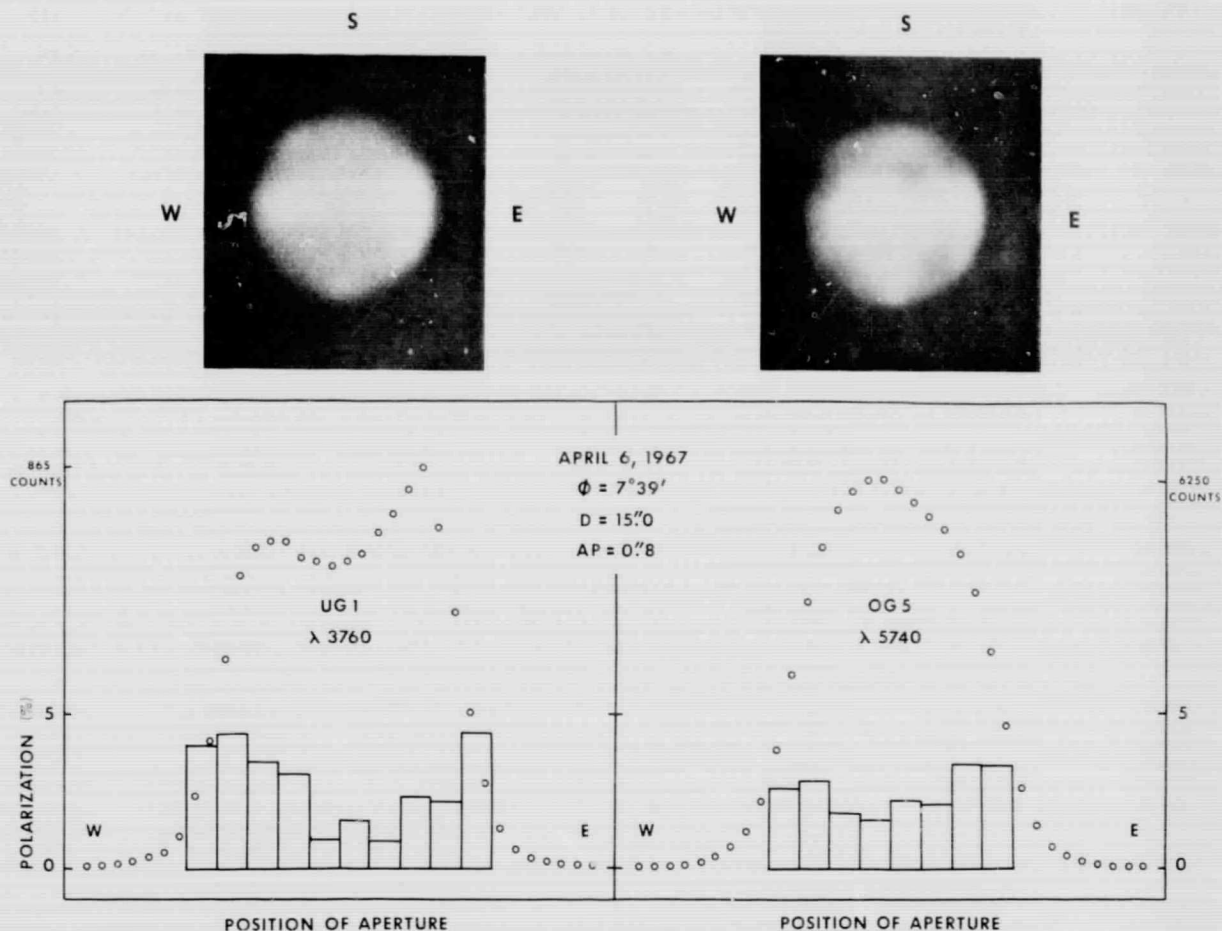
Figure 1. Intensity scans along the equatorial zone of Mars made on April 6, 1967. The polarization observed is indicated by the histograms. The phase angle of Mars was 7.6 degrees, its apparent diameter 15.0 arc seconds, and the aperture 0.8 arc seconds. In both wavelength regions the clouds at the limbs show the most polarization. The photographs were obtained in the blue and yellow regions with the Lowell 24-inch refractor near the time when the observations below them were obtained.
