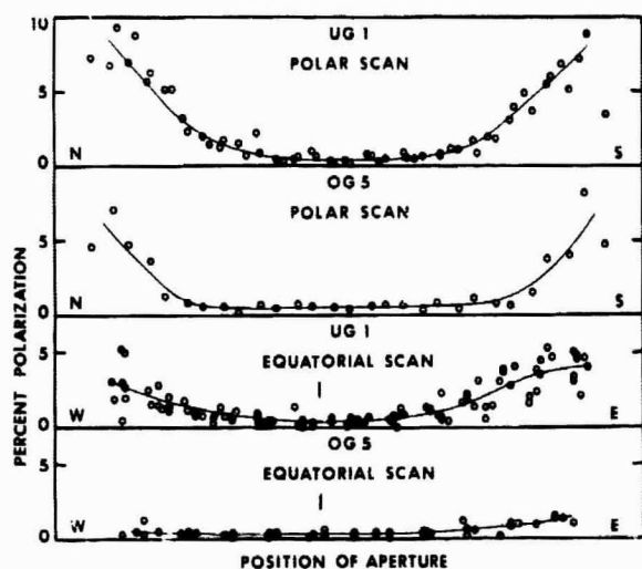
Figure 6. Degree of polarization of points on Jupiter's disk along polar and equatorial diameters. The polar scans in both colors show symmetry with respect to the center of the disk. The equatorial data for UG 1 are more nearly symmetrical with respect to the subsolar point (designated by vertical markers) than to the center of the planet. All observations are included.
