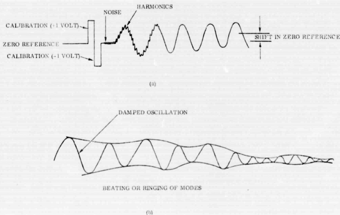
Figure 14. Examples of Superimposed Effects on Damping Determination
