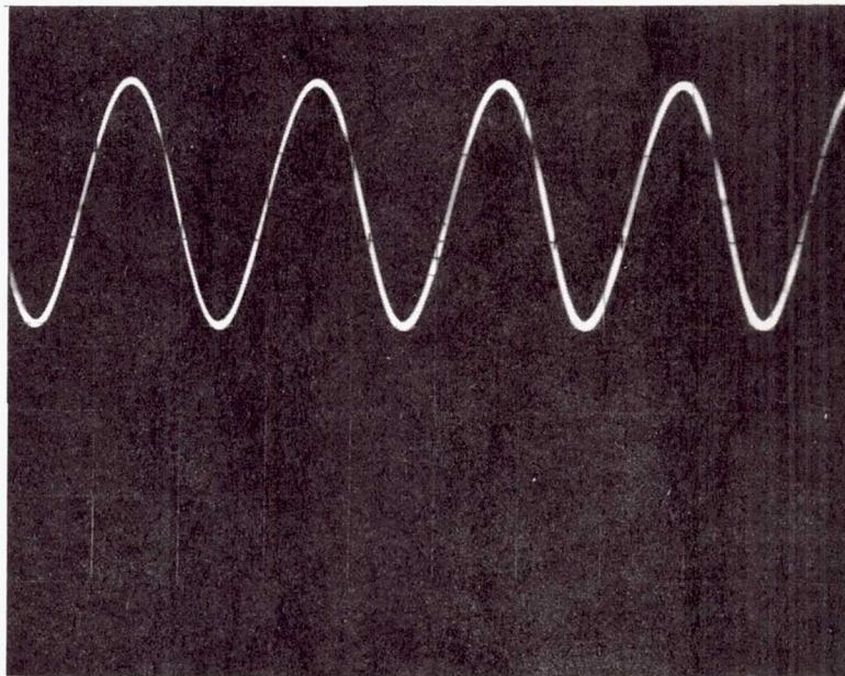
Figure A2b. Oscilloscope Trace of Beat Frequency of Approximately 1 MHz of Two Lasers. Internal trigger operation, 0.5 \times 10^{-7} Second/cm Horizontal Sweep, 1 second Exposure.
