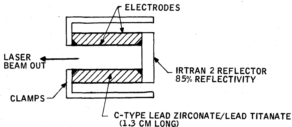
(a) TRANSDUCER FOR TRANSITION CONTROL (ONE IN EACH LASER)
