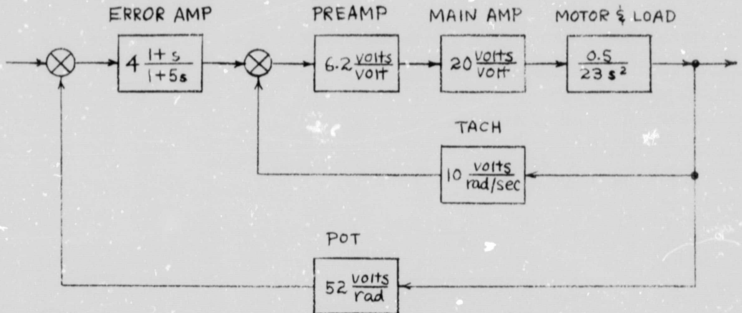
Figure 6-28. Block Diagram of Azimuth Servo Loop
