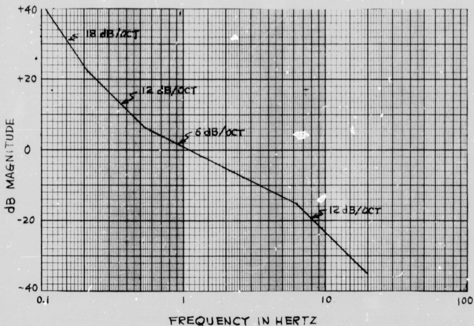
Figure 6-20. Bode Asymptotic Diagram for Compensated Open-Loop Transfer Function of Manual Control Loop
