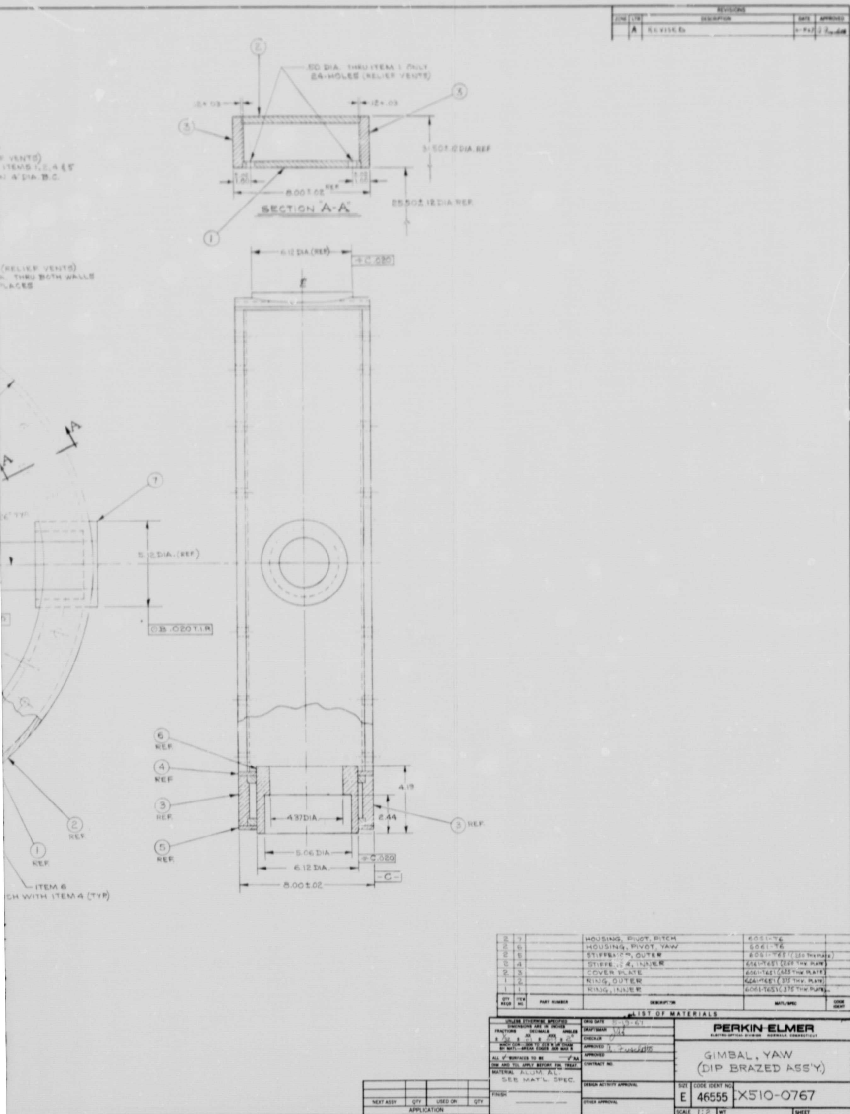
Figure 4-2. Yaw Gimbal Assembly 4-7
