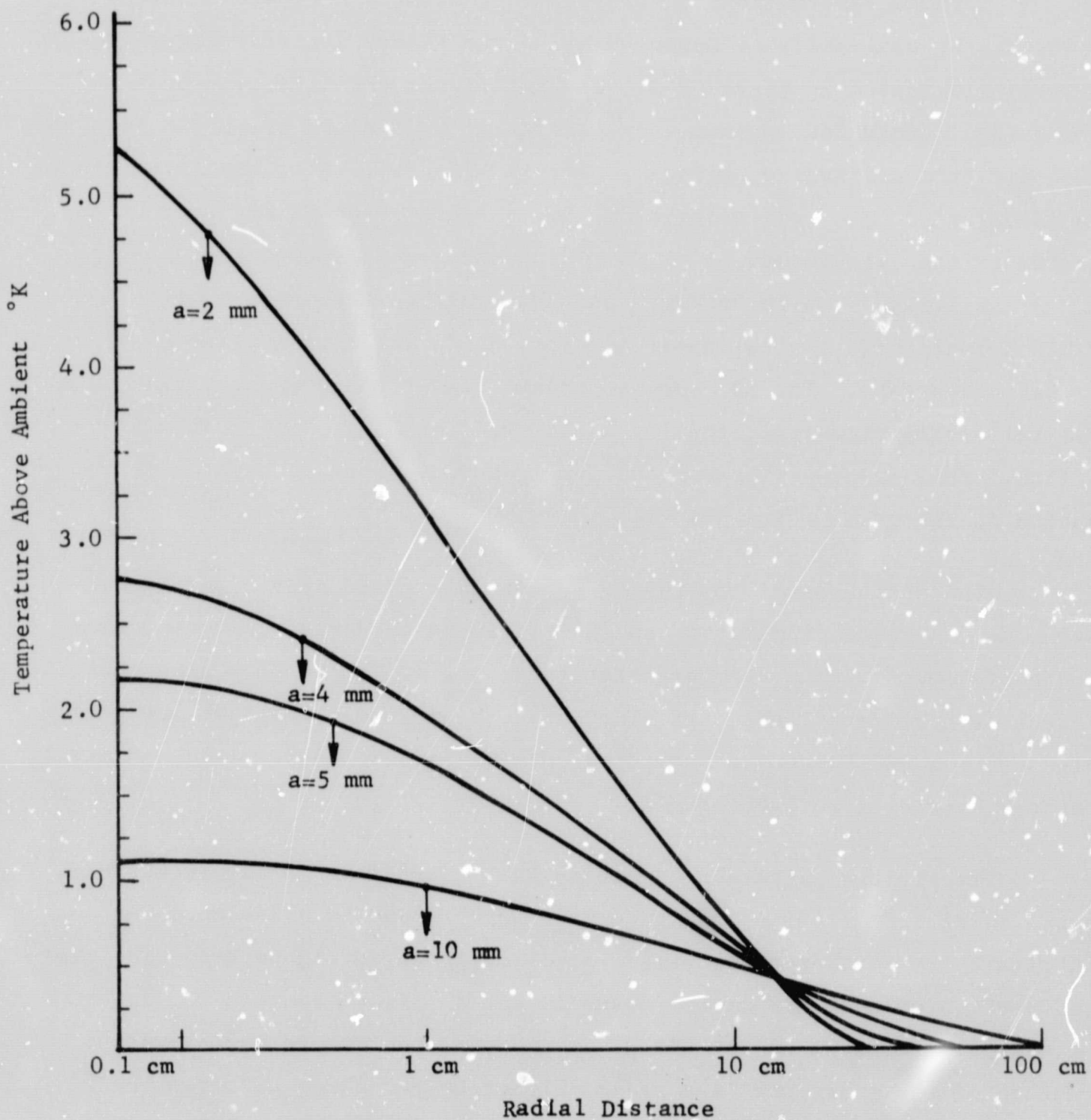
Figure B-3. Radial Temperature Distribution in a Thin Plate of \text{BaF}_2 with 1 Watt of \text{CO}_2 (Gaussian) Passing Through It. \alpha = 0.15 \text{ cm}^{-1} at 10.6\mu
