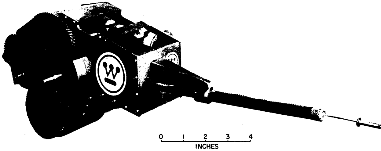
Fig. 3. Deployer for 150-ft-long boom, with provision for tip mass
