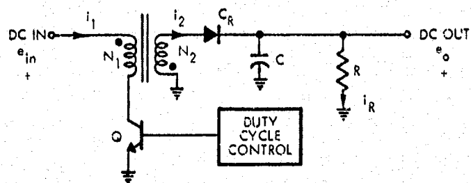
Figure 3-5. Basic Energy Ladling Circuit
