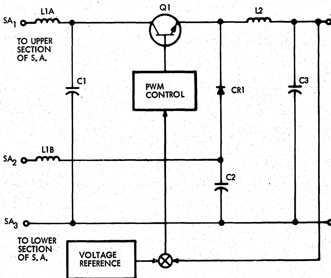
Figure 6-5. Quasi-Buck Series Regulator
