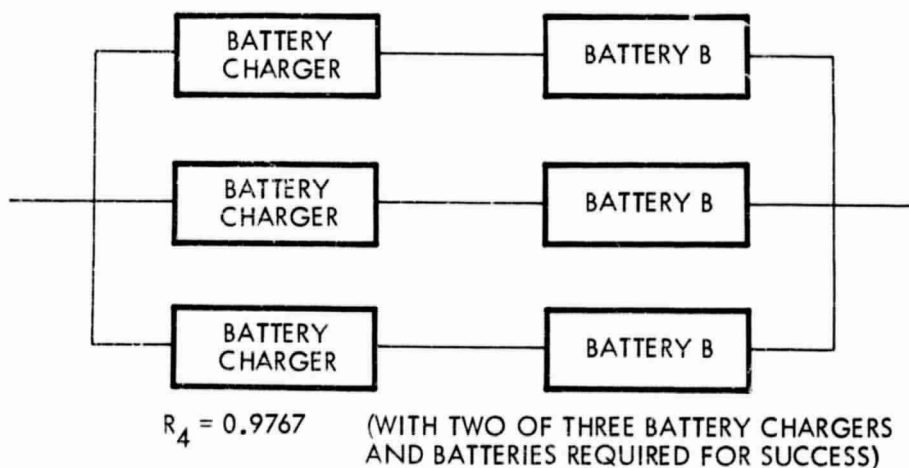
Figure C-4. Case 4 - Battery Redundancy Configuration No. 4
