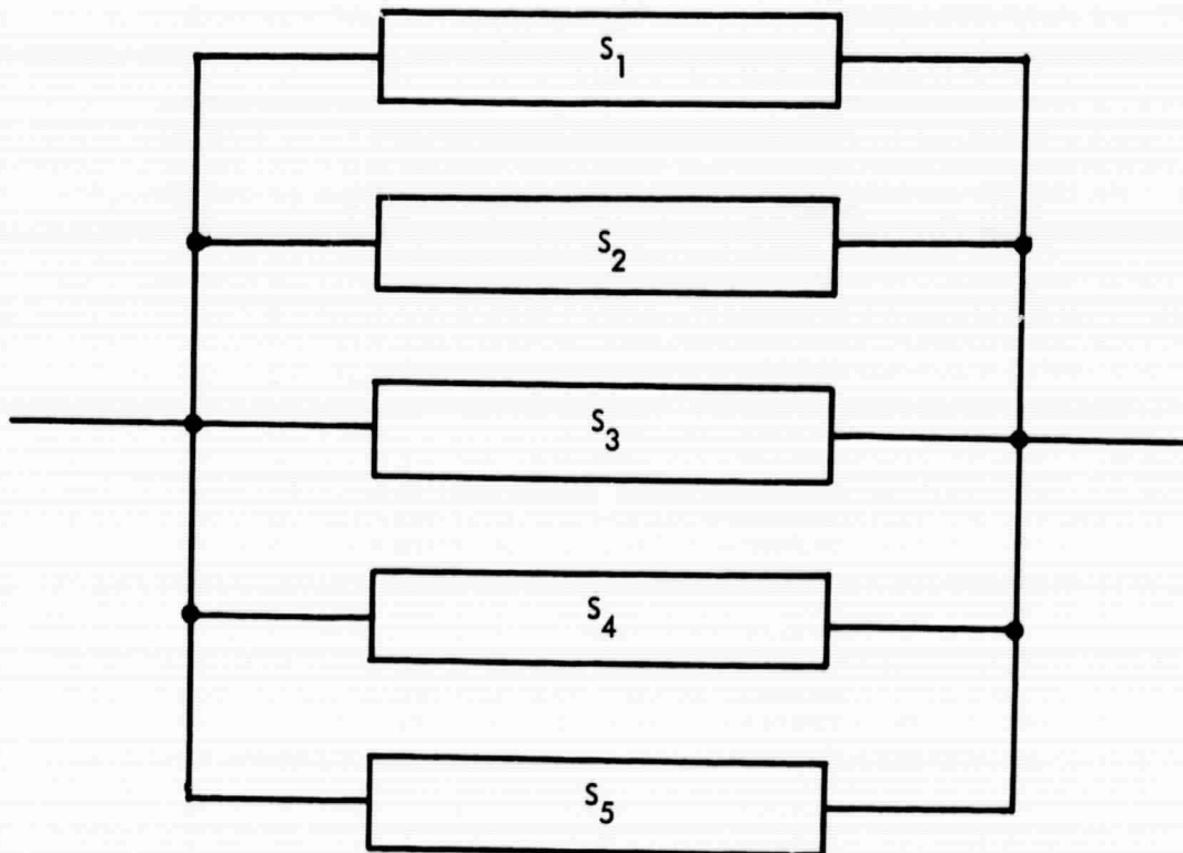
Figure 8-8. Parallel Redundancy
