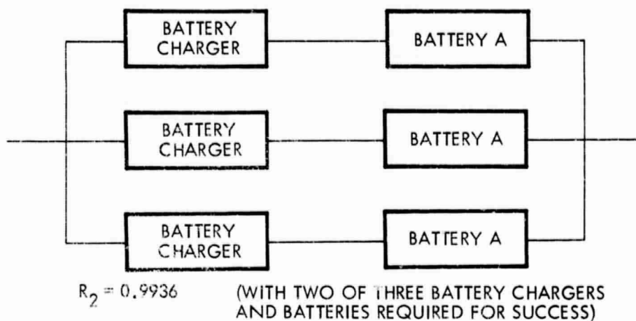
Figure C-2. Case 2 - Battery Redundancy Configuration No. 2
