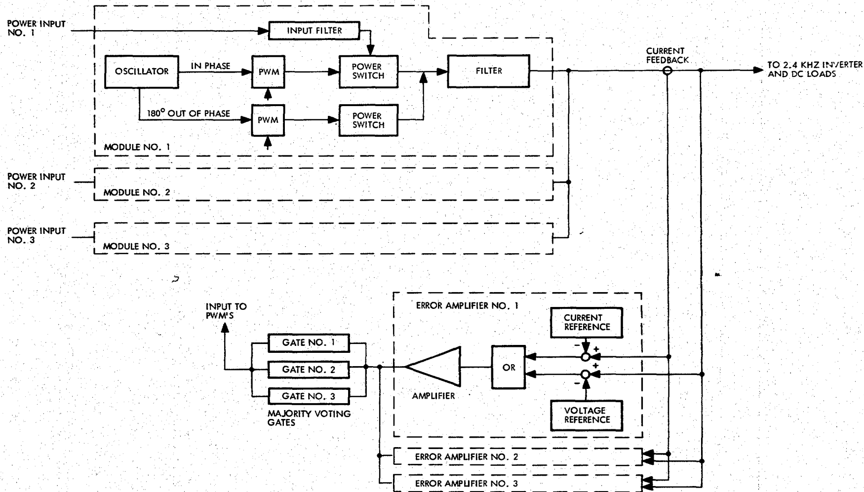
Figure 6-8. Buck-Boost Regulator Block Diagram
