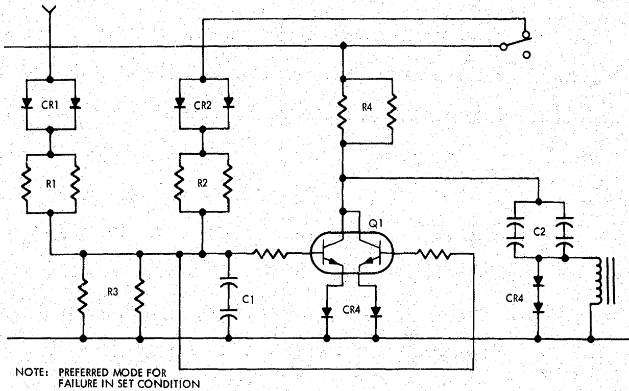
Figure 6-21a. Fail-Safe Relay Driver
