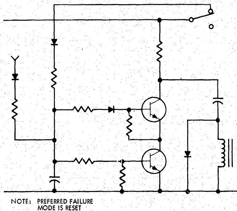
Figure 6-21a. Fail-Safe Relay Driver
