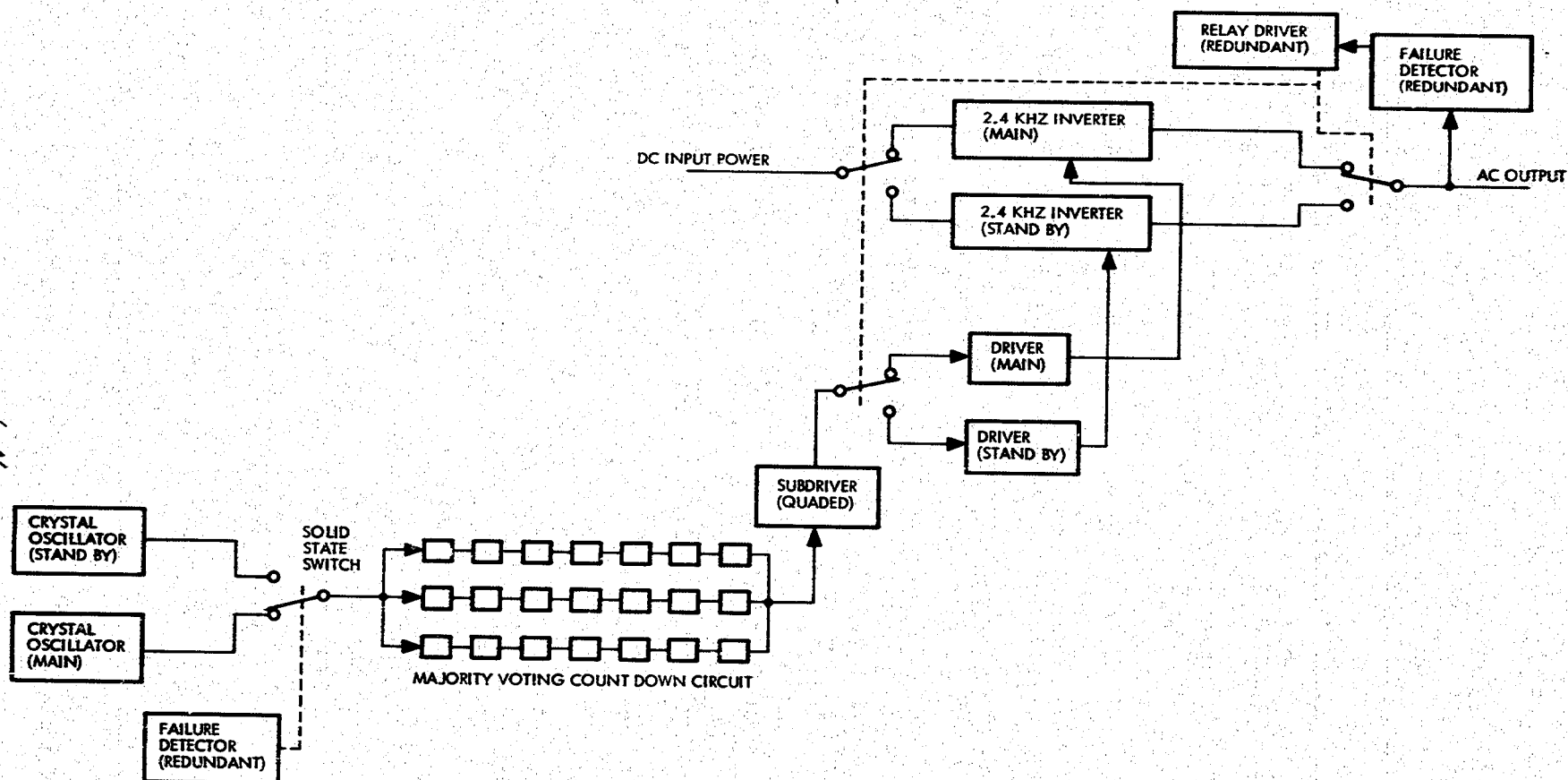
Figure 6-15. 2.4 kHz Inverter Block Diagram
