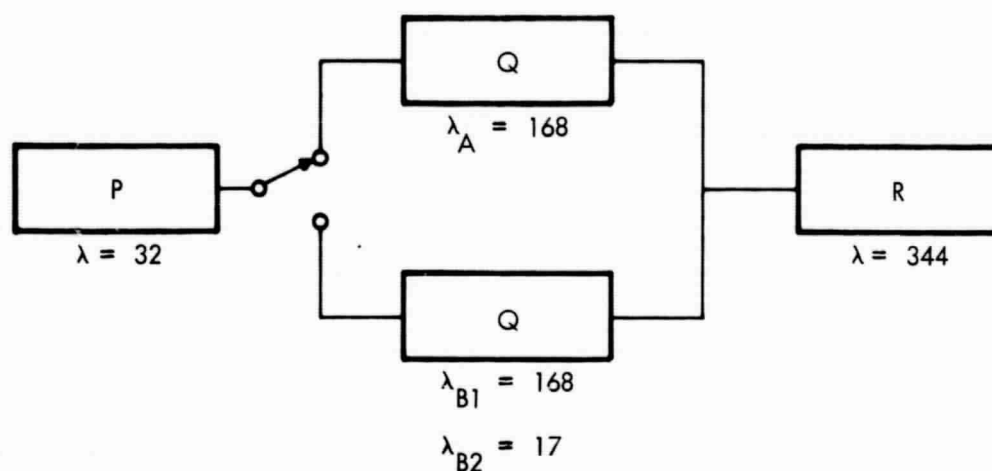
RELIABILITY BLOCK DIAGRAM
