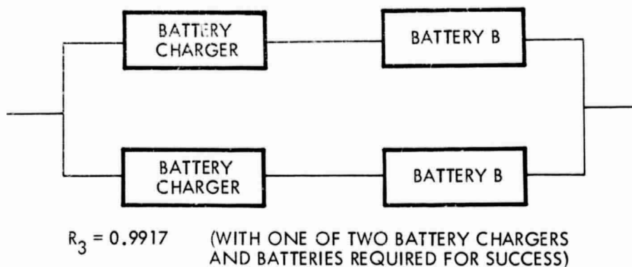
Figure C-3. Case 3 - Battery Redundancy Configuration No. 3
